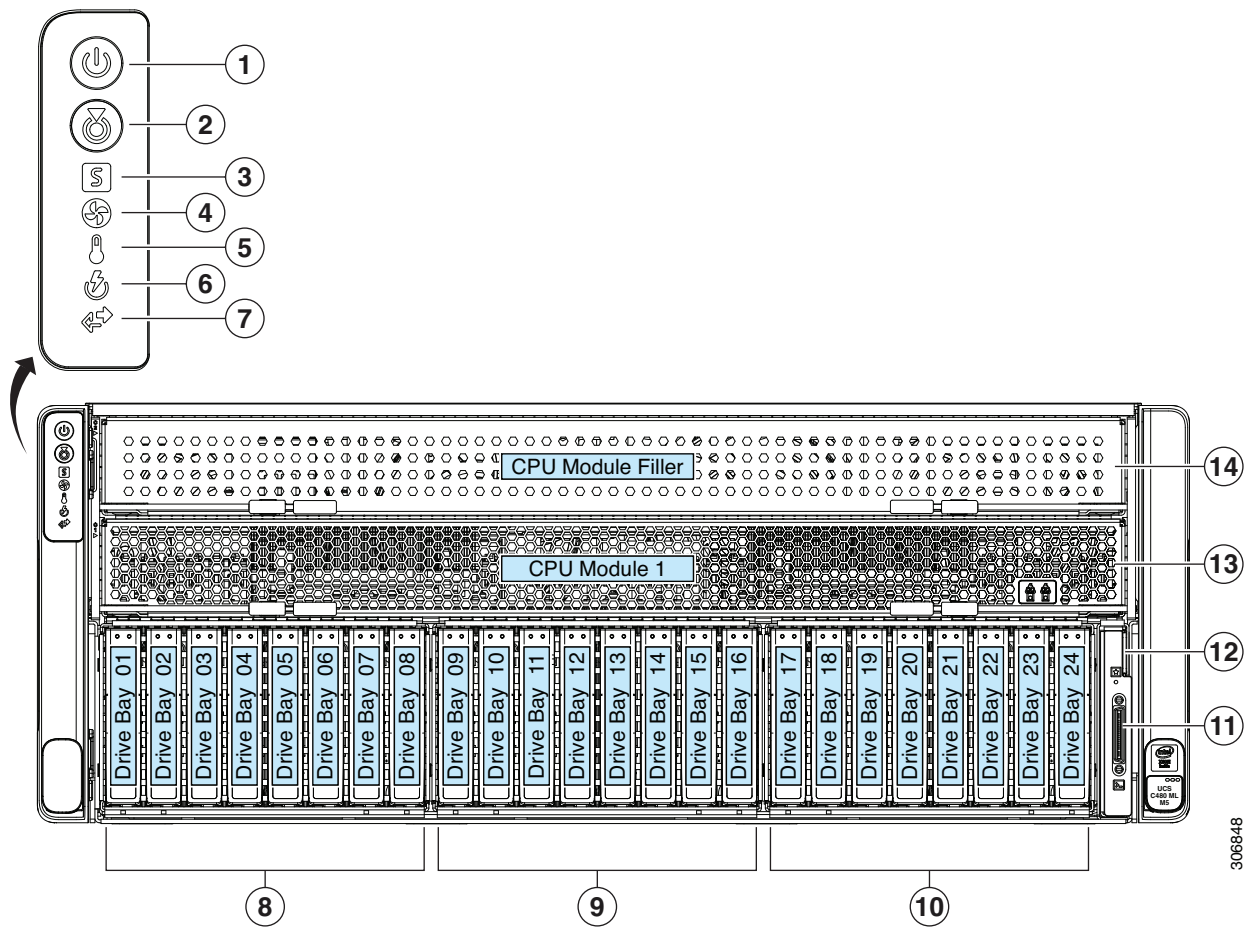
Figure 2 Chassis Front View
