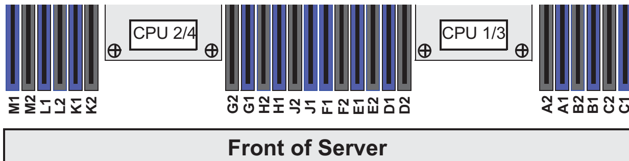
Figure 9 Physical Layout of CPU DIMM Channels and Slots
