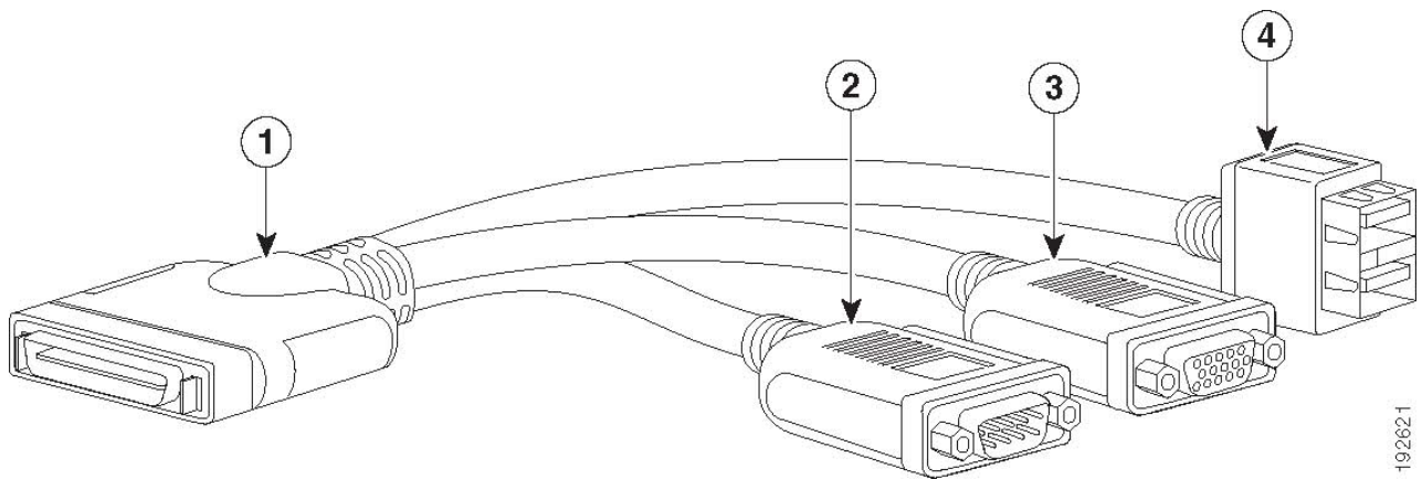
Figure 10 KVM Cable
