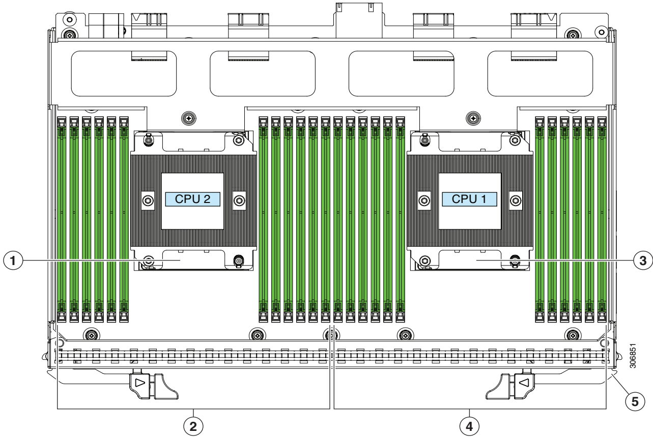
Figure 7 Serviceable Component Locations Inside a CPU Module
