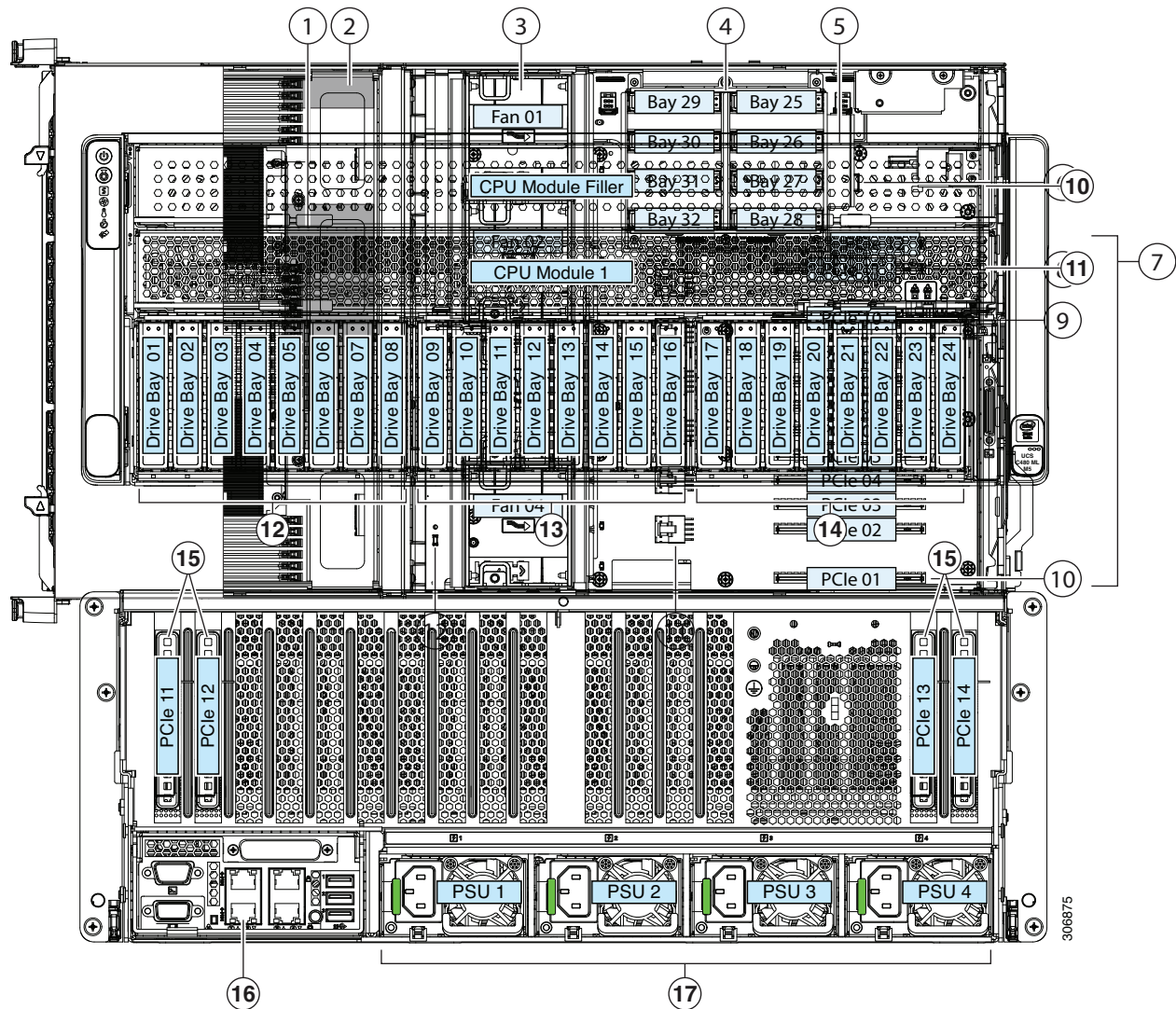
Figure 6 Serviceable Component Locations Inside the Main Chassis (Front and Rear Views)
