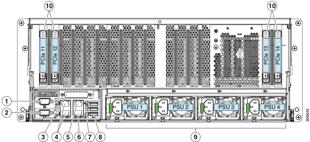
Figure 3 UCS C480 ML M5 Server Rear Panel
