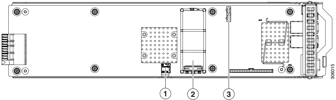
Figure 8 Serviceable Component Locations Inside a I/O Module
