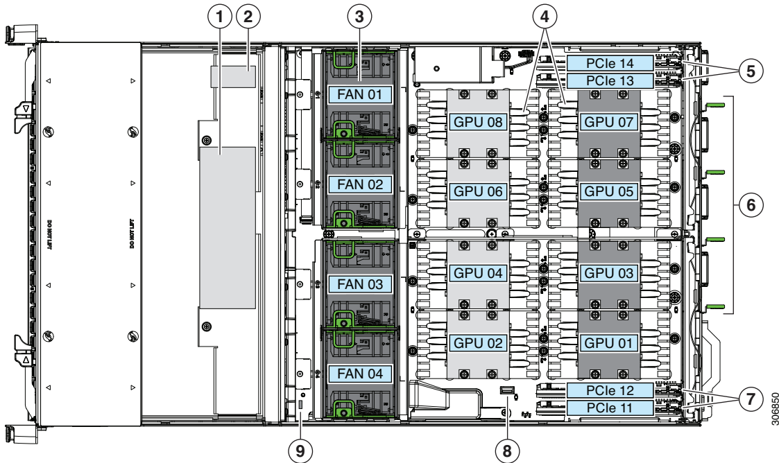
Figure 5 C480 ML M5 With Top Cover Removed
