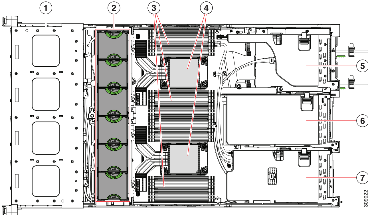
Figure 5 C245 M6 Server With Top Cover Off
