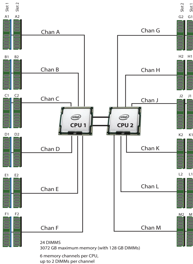
Figure 4 HXAF240c M5 Node Memory Organization
