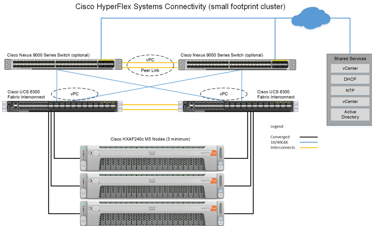
Figure 5 Small Footprint Cluster Using HXAF240c M5 Nodes With Fabric Interconnect Deployment Mode
