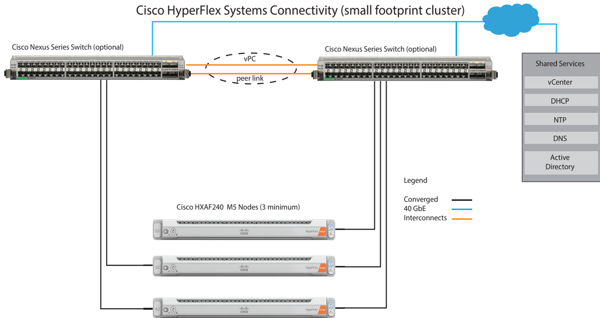
Figure 6 Small Footprint Cluster Using HXAF240c M5 Nodes Data Centre Without Fabric Interconnect Deployment Mode
