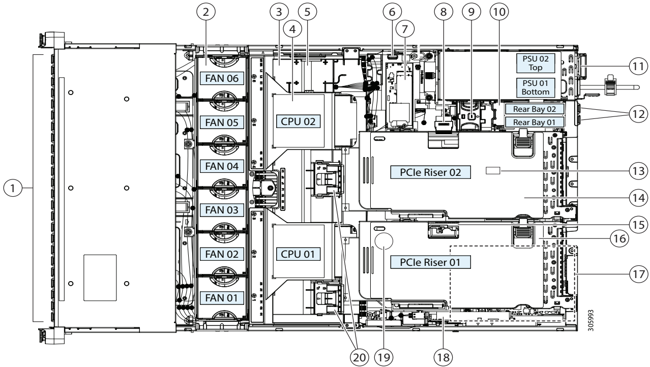
Figure 8 HXAF240c M5 With Top Cover Off
