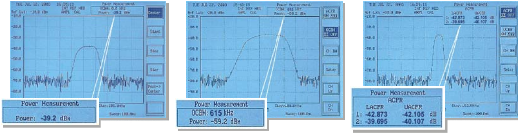
Channel Power Measurement
