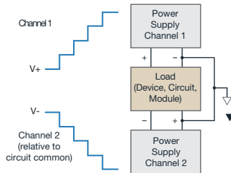
Use the two 30V channels to test a bipolar integrated circuit or a bipolar module over its specified voltage operating range.
