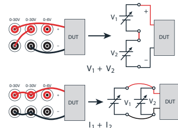
Combine two channels in series to output up to 60V or combine two channels in parallel to output up to 3A. The Model 2220/2230display will show the combined value.
