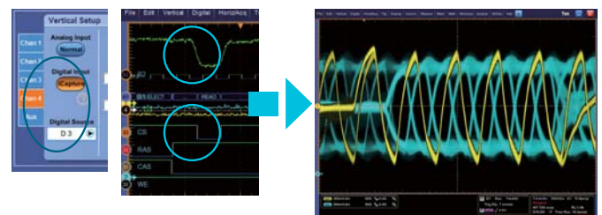
Example: Using iCapture function to observe the analog terminals connected to digital channels
