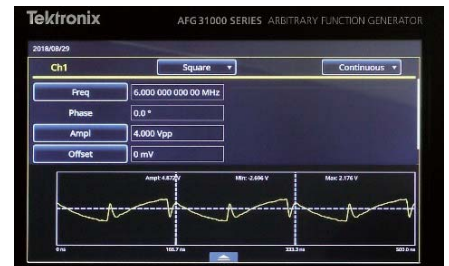
With InstaView on AFG31000 turned on. The AFG31000 shows the waveform as observed at the DUT.
