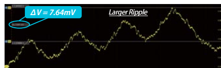
TPP1000 Passive Probe 20MHz Band Limitation
