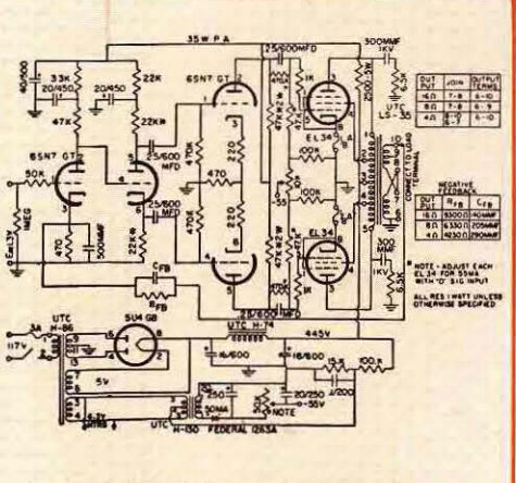
CIRCUIT PROVIDING 35 WATTS, \pm 1 db from 15 cycles to 30 KC ... At 1 watt, \pm 1 db 7 cycles to 100 KC.
