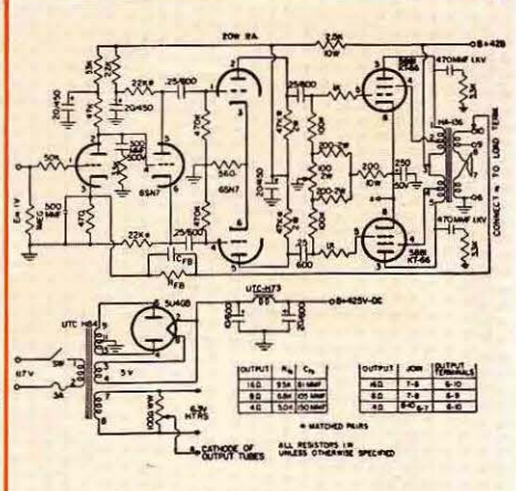
CIRCUIT PROVIDING 20 WATTS, \pm 1 db 20 cycles to 30 KC ... At 1 watt, \pm 1 db 7 cycles to 100 KC.
