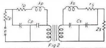
Fig 2 ILLUSTRATING A PHYSICAL TRANSFORMER
