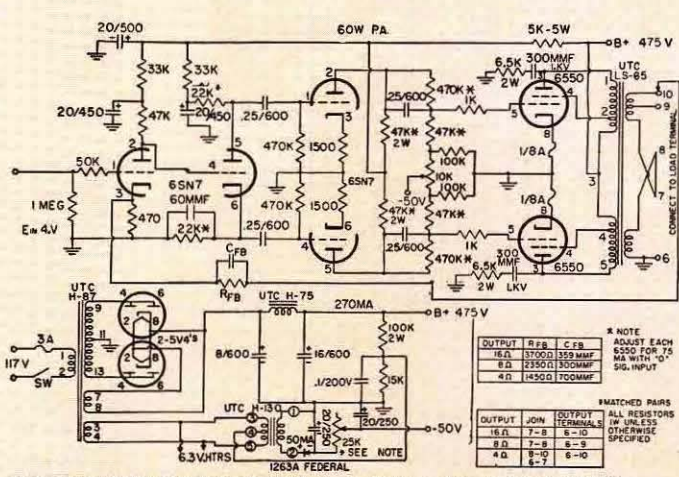
CIRCUIT PROVIDING 60 WATTS, \pm 1 db from 15 cycles to 30 KC ... At 1 watt, \pm 1 db 3 cycles to 80 KC.
