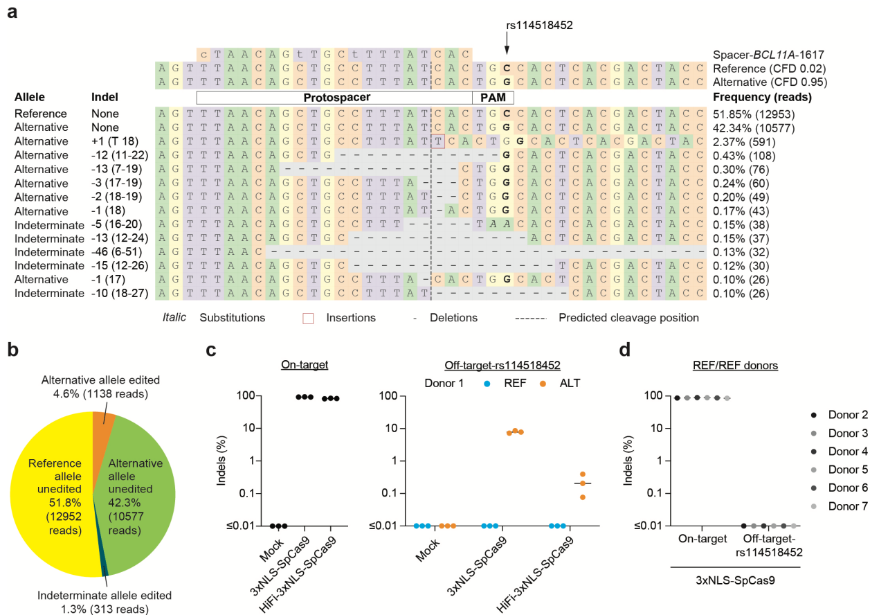
Figure 3. Allele-specific off-target editing by a BCL11A enhancer targeting gRNA in clinical trials associated with a common variant in African-ancestry populations. a) Human CD34+ HSPCs from a donor heterozygous for rs114518452-G/C (Donor 1, REF/ALT) were subject to 3xNLS-SpCas9:sg1617 RNP electroporation followed by amplicon sequencing of the off-target site around chr2:210,530,659-210,530,681 (off-target-rs114518452 in 1-start hg38 coordinates). CFD scores for the reference and alternative alleles are indicated and representative aligned reads are shown. Spacer shown as DNA sequence for ease of visual alignment, with mismatches indicated by lowercase and the rs114518452 position shown in bold. b) Reads classified based on allele (indeterminate if the rs114518452 position is deleted) and presence or absence of indels (edits). c) Human CD34+ HSPCs from a donor heterozygous for rs114518452-G/C (Donor 1) were subject to 3xNLS-SpCas9:sg1617 RNP electroporation, HiFi-3xNLS-SpCas9:sg1617 RNP electroporation, or no electroporation (mock) followed by amplicon sequencing of the on-target and off-target-rs114518452 sites. Each dot represents an independent biological replicate ( n = 3 ). Indel frequency was quantified for reads aligning to either the reference or alternative allele. d) Human CD34+ HSPCs from 6 donors homozygous for rs114518452-G/G (Donors 2-7, REF/REF) were subject to 3xNLS-SpCas9:sg1617 RNP electroporation with 1 biological replicate per donor followed by amplicon sequencing of the on-target and off-target-rs114518452 sites.
