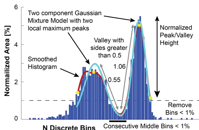
Figure A1: Multi-modality Detector. Generic function to determine if more than one mode (group) is present in a 1 dimensional data set. Histogram is formed from data in N bins ( N is the square root of the number of data points (Mosteller, F. and Tukey (1977, p. 49)). Histogram is normalized by the sum of the bin area. A smoothed histogram generated by choosing each bin value as the median of the bin before and after it (Cocatre-Zilgien 1992); the output is filtered by a moving average (window size = 5 bins). All preceding and trailing bins less than 1% are removed from analysis. Three identifiers are used to find number of modes. First, a Gaussian Mixture Model is generated with M components ( M is equal to the number of local max peaks of the smoothed histogram); second, if consecutive middle bins are found below the 1% threshold then two or more modes are present; third, a local valley is found with both sides greater than the normalized height of .50 then two or more modes are present.
