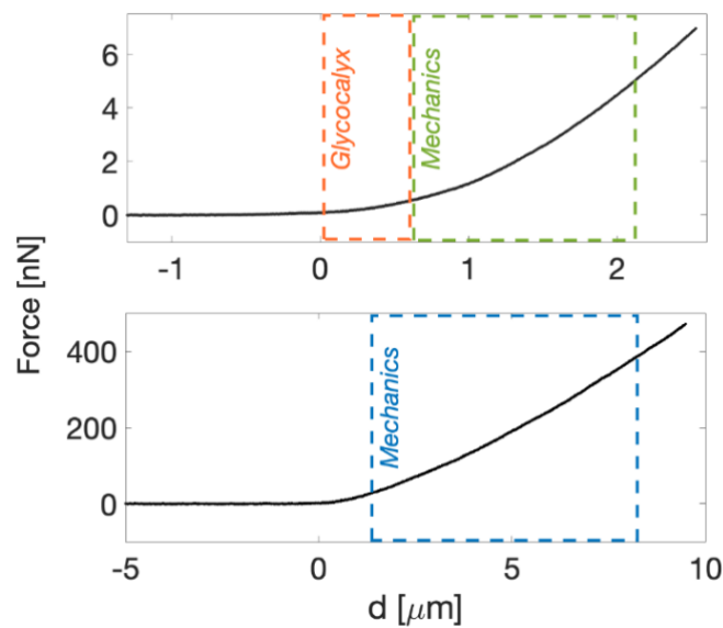
Figure 2. Typical approaching force curve on top of a cell (top) and ECM (bottom). The indentation range for model fitting are highlighted; on cells, we used typically [0-10%] for the glycocalyx and [10-80%] for the YM, while on ECMs we used [20-80%] for the Young's modulus.
