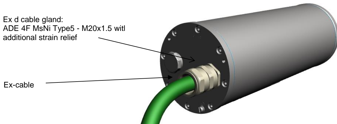
Fig. 5-2 Cable gland and Ethernet cable
