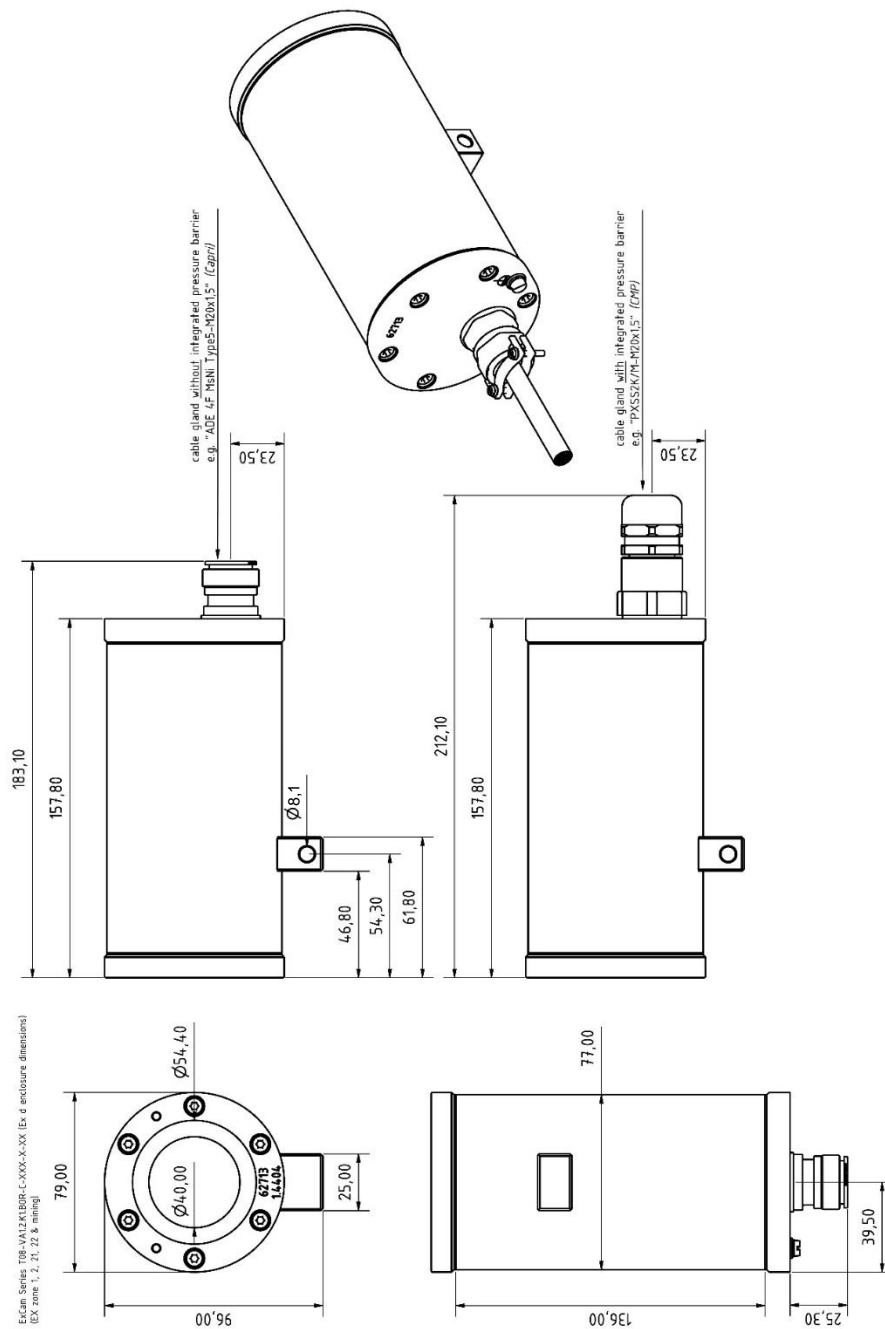
Fig. 11-1 – Dimensions of the T08 ExCam XF M3016
