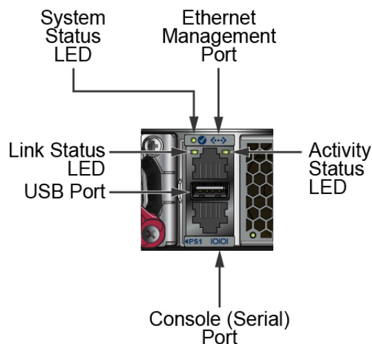
Figure 4-6: Rear Panel Ports
