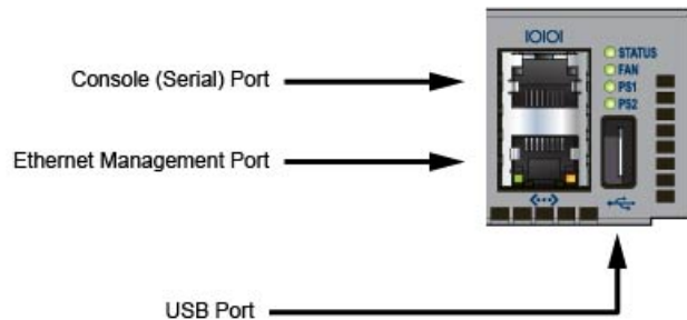
Figure 4-6: Rear Panel Ports
