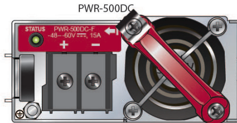
Figure 4-4: Supported DC power supplies
