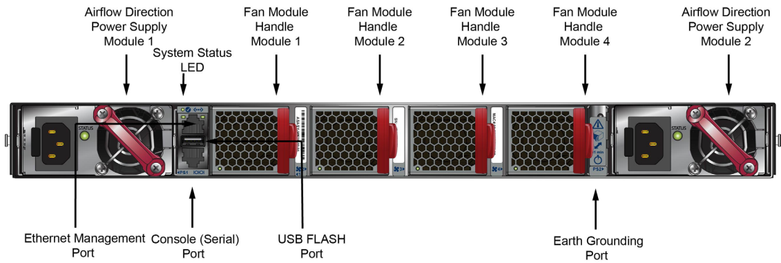
Figure D-2: Rear Panel for DCS-7020SR-24C2 and DCS-7020SRG-24C2
