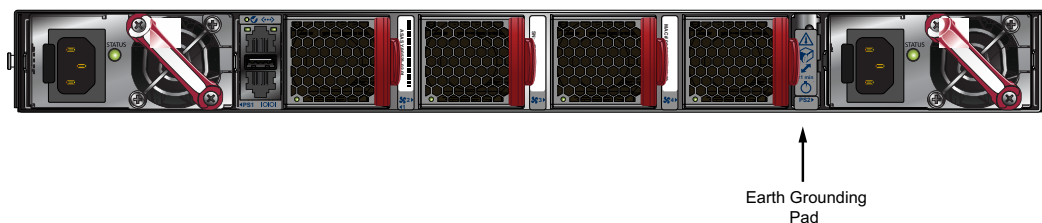
Figure 4-2: Earth Grounding Pad Sockets for DCS-7020SR-24C2 and DCS-7020SRG-24C2
