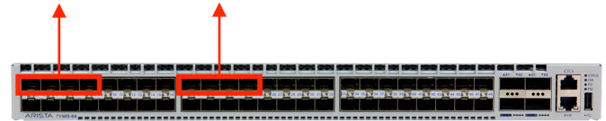
Arista 7150 Series AgilePorts - Four SFP+ grouped to deliver 40GbE
