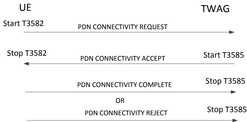
Figure 5.2.2.1: PDN connectivity establishment procedure
