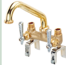
04-008 4" Brass Laundry tray faucet, with 6" spout 24pc/23kg/24kg/1.5'
