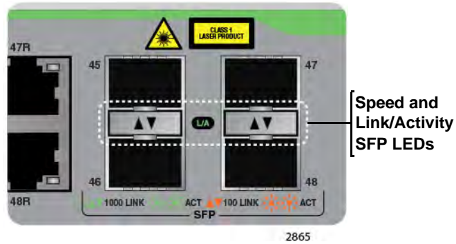
Figure 17. AT-GS950/48PS SFP Status LEDs
