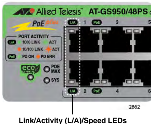
Figure 13. AT-GS950/48PS Link/Activity/Speed Port LEDs
