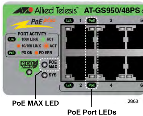
Figure 21. AT-GS950/48PS PoE and PoE MAX LEDs
