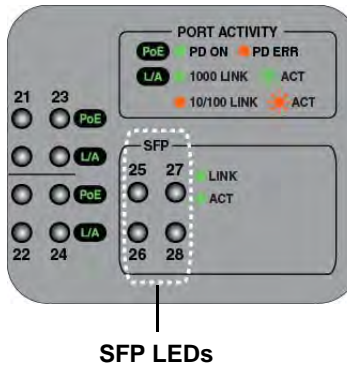
Figure 16. AT-GS950/28PS SFP Status LEDs
