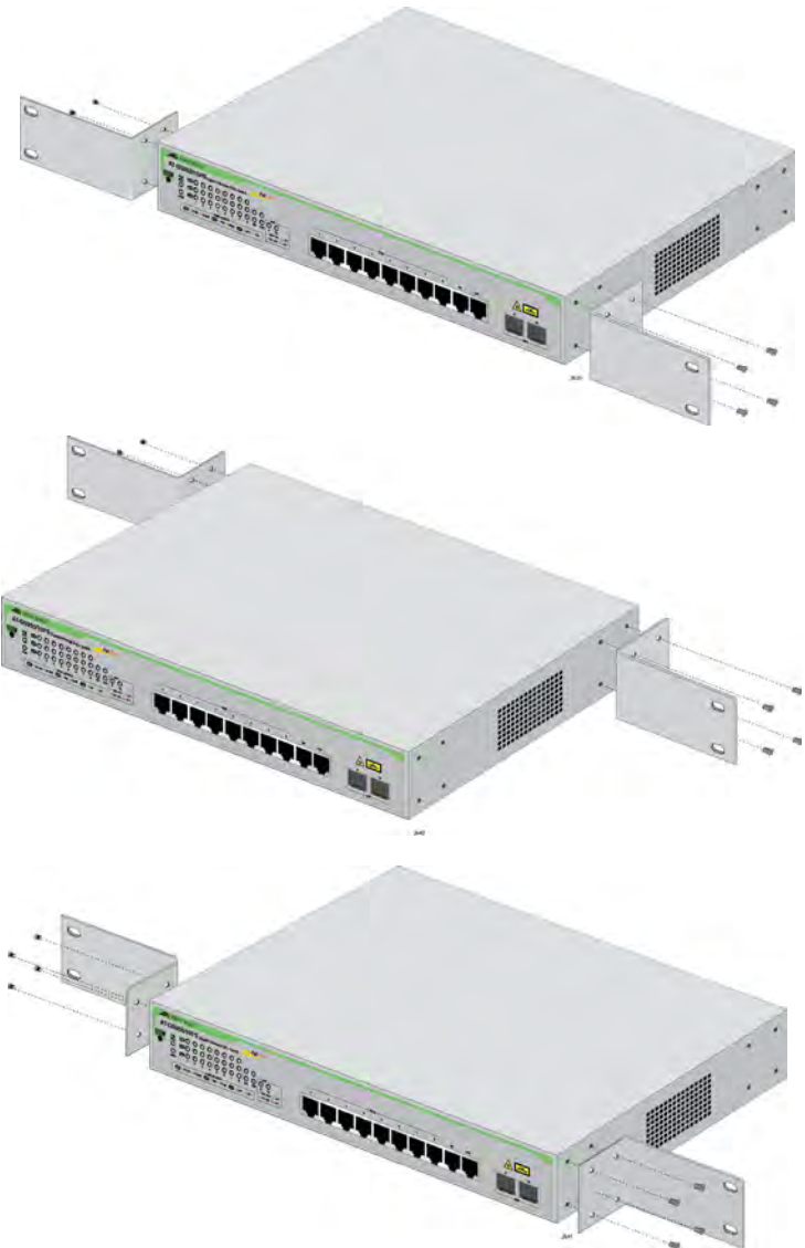
Figure 26. Attaching the Rack-Mount Brackets to the Switch
