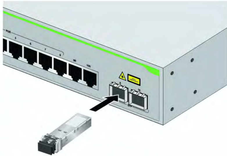
Figure 32. Inserting the SFP
