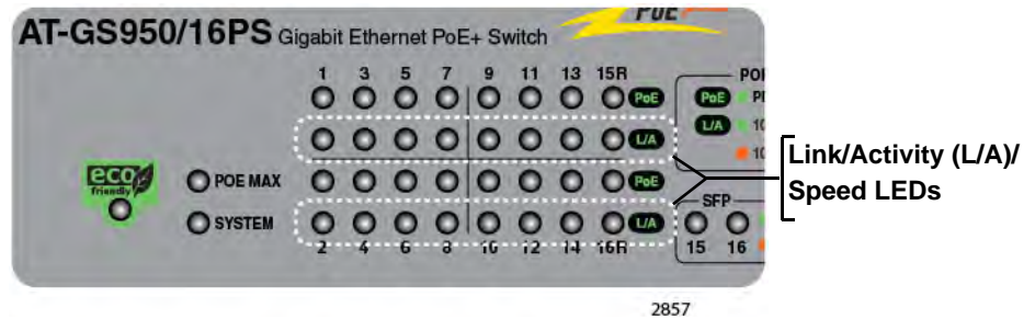
Figure 11. AT-GS950/16PS Link/Activity/Speed LEDs
