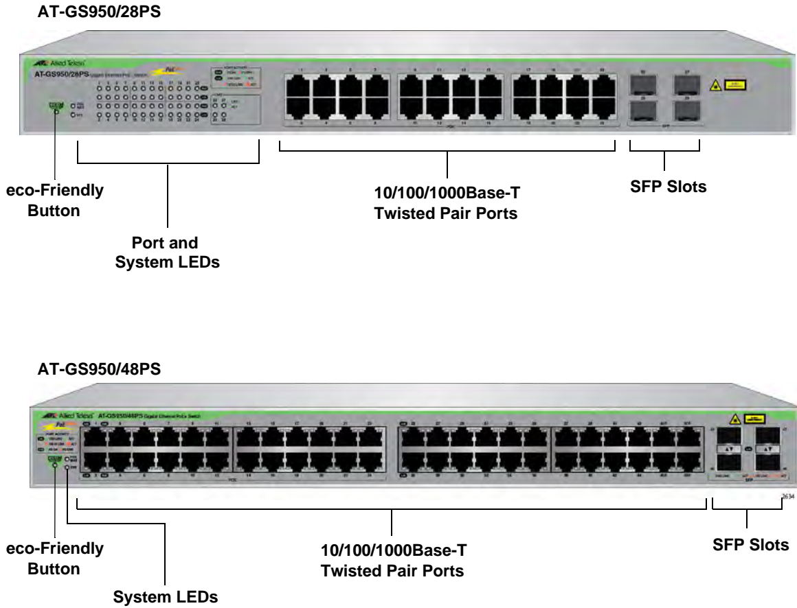
Figure 2. AT-GS950/28PS and AT-GS950/48PS Front Panels
