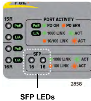
Figure 15. AT-GS950/16PS SFP Status LEDs
