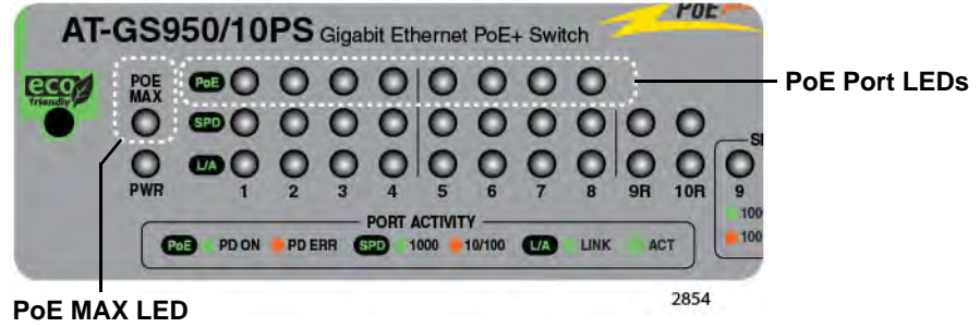
Figure 18. AT-GS950/10PS PoE and PoE MAX LEDs
