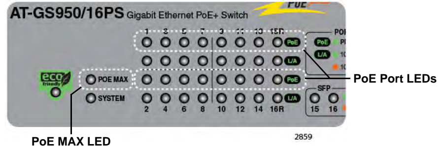
Figure 19. AT-GS950/16PS PoE and PoE MAX LEDs
