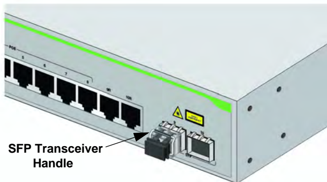
Figure 33. Positioning the SFP Handle in the Upright Position
