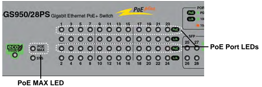
Figure 20. AT-GS950/28PS PoE and PoE MAX LEDs
