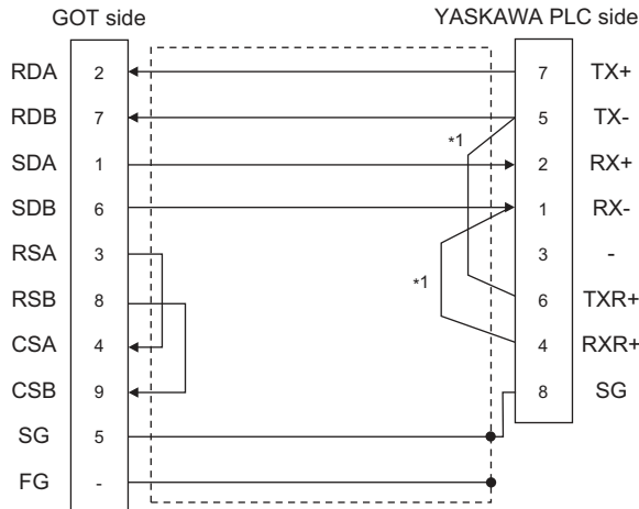
(b) RS-422 connection diagram 2)
