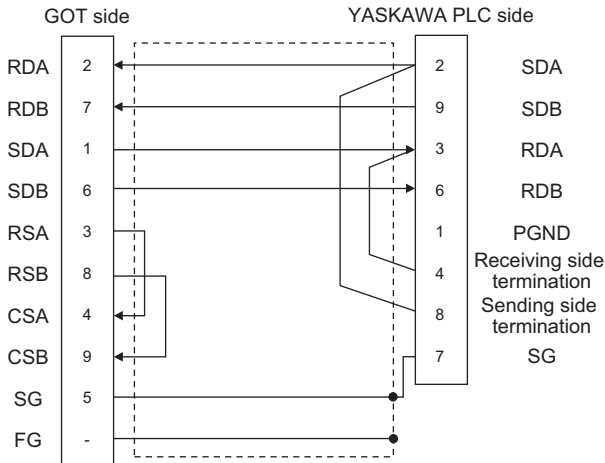
(b) RS-422 connection diagram 2)
