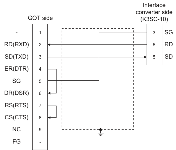
(3) RS-232 connection diagram 3)
