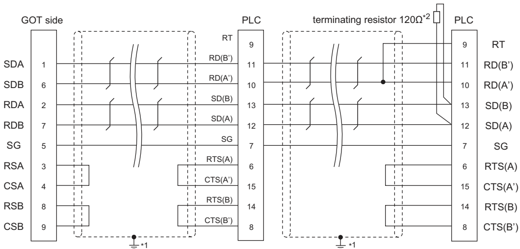
(2) RS-422 connection diagram 2)
