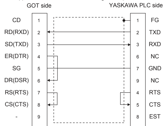
(f) RS-232 connection diagram 6)
