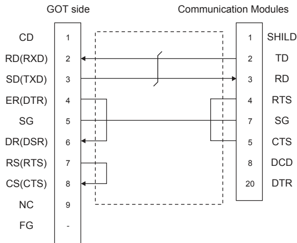
(1) RS-232 connection diagram 1)
