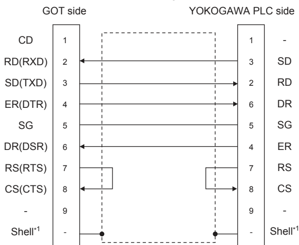
(b) RS-232 connection diagram 2)
