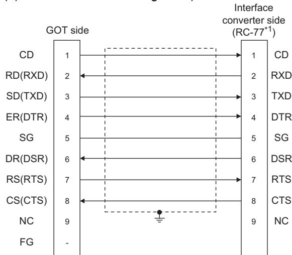
(1) RS-232 connection diagram 1)
