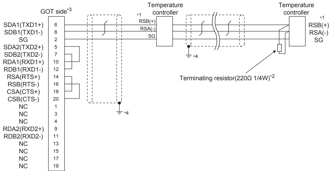
(19) RS-485 connection diagram 19)
