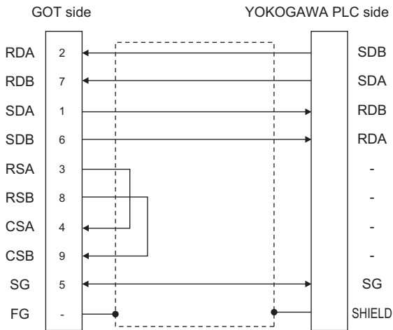
(b) RS-422 connection diagram 2)
