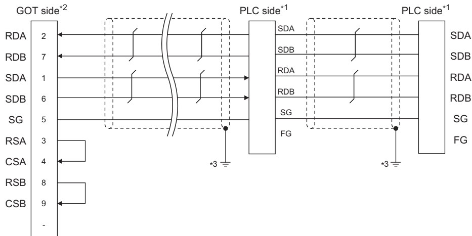
(1) RS-485 connection diagram 1
