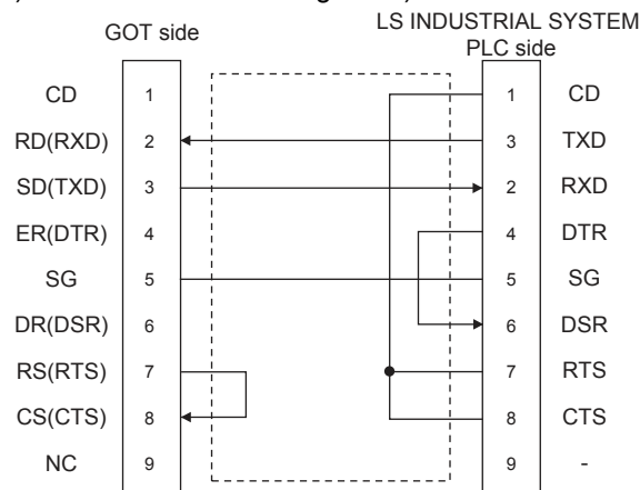
(2) RS-232 connection diagram 2)
