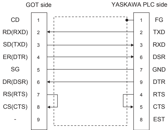
(a) RS-232 connection diagram 1)
