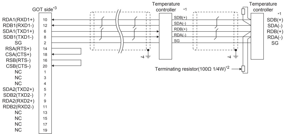
(17) RS-485 connection diagram 17)
