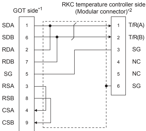
(1) RS-485 connection diagram 1)
