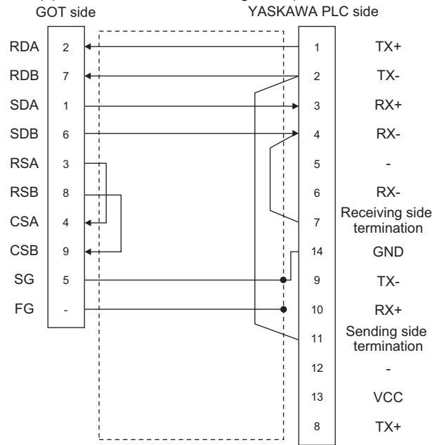
(c) RS-422 connection diagram 3)
