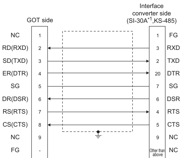
(2) RS-232 connection diagram 2)
