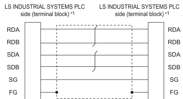
(2) RS422 connection diagram 3)
