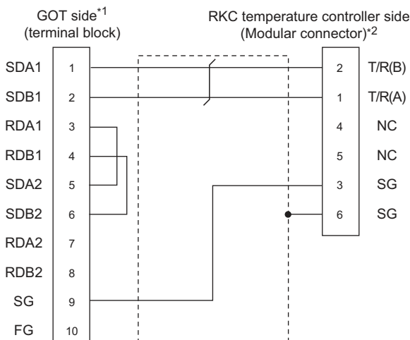
(2) RS-485 connection diagram 2)
