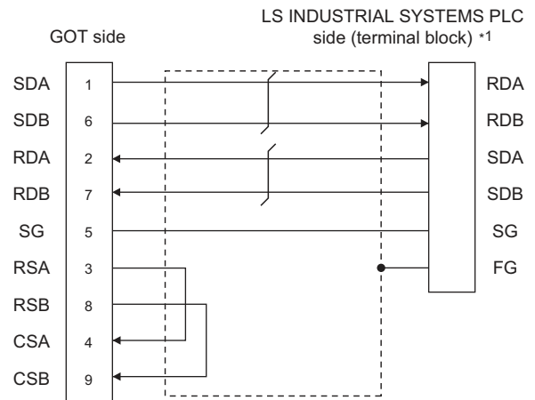
(1) RS-422 connection diagram 1)
