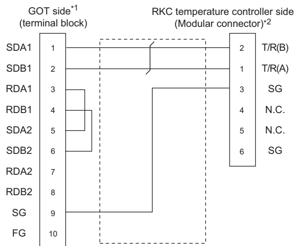
(4) RS-485 connection diagram 4)
