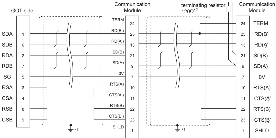
(1) RS-422 connection diagram 1)
