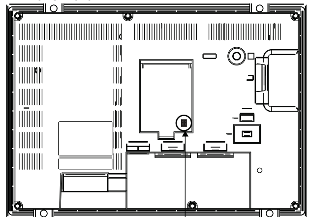
Terminating resistor setting switch (inside the cover)
