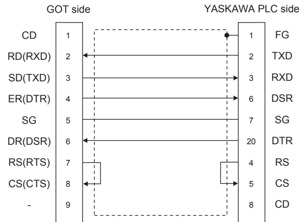
(e) RS-232 connection diagram 5)
