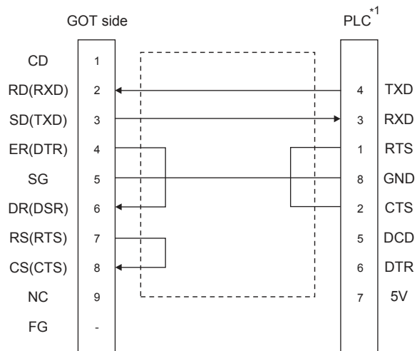
(2) RS-232 connection diagram 2)
