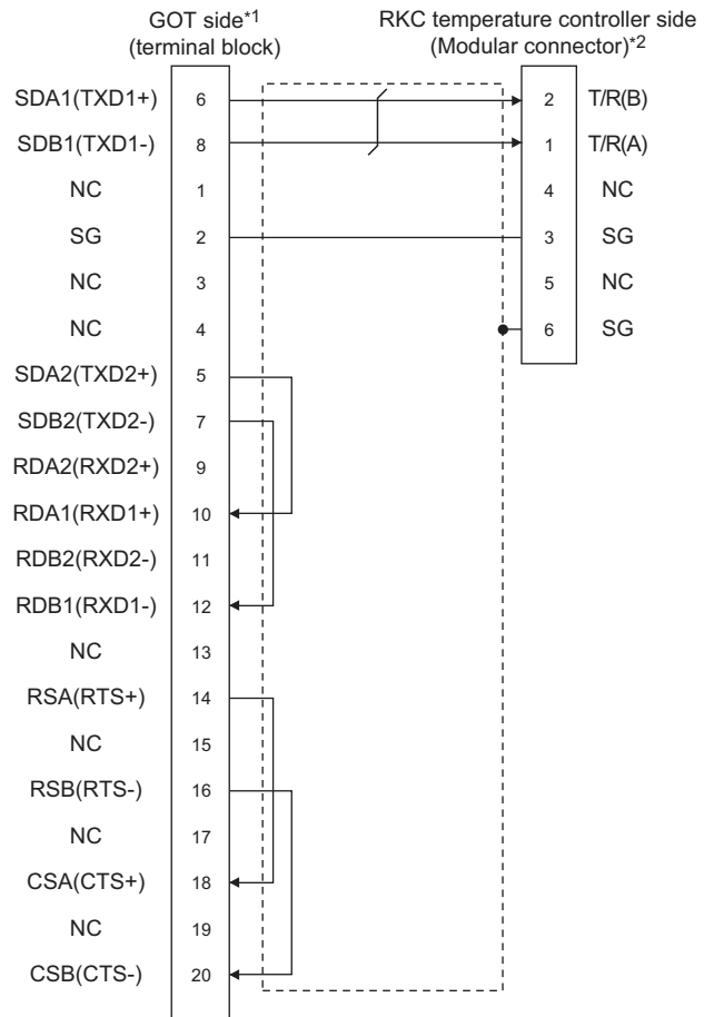
(3) RS-485 connection diagram 3)
