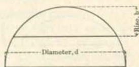
AREAS OF CIRCULAR SEGMENTS TABLE II, FOR RATIOS OF RISE AND DIAMETER
