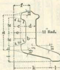
S 90 RB to S 60 RB
