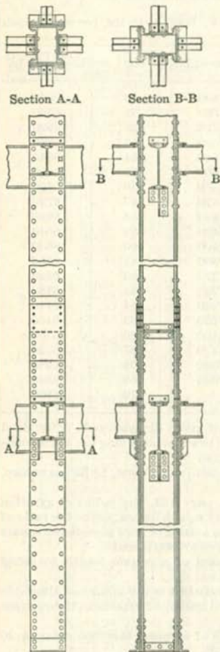
TYPICAL CHANNEL COLUMN
