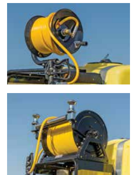
200 GALLON PCO - Unit Shown: Includes LS-PCO-200, Diaphragm Pump Kit, 300 Ft Hose Reel W/ Spool Kit & Stand, 1/2" 600# Hose
