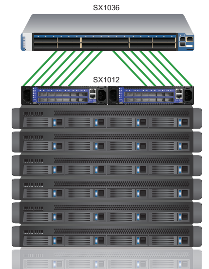
Figure 1. 10GbE ToR Switch
