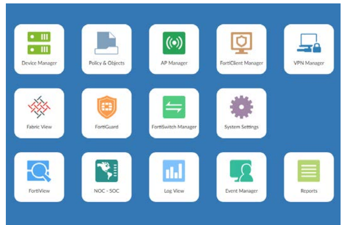
Figure 3: FortiManager Dashboard
