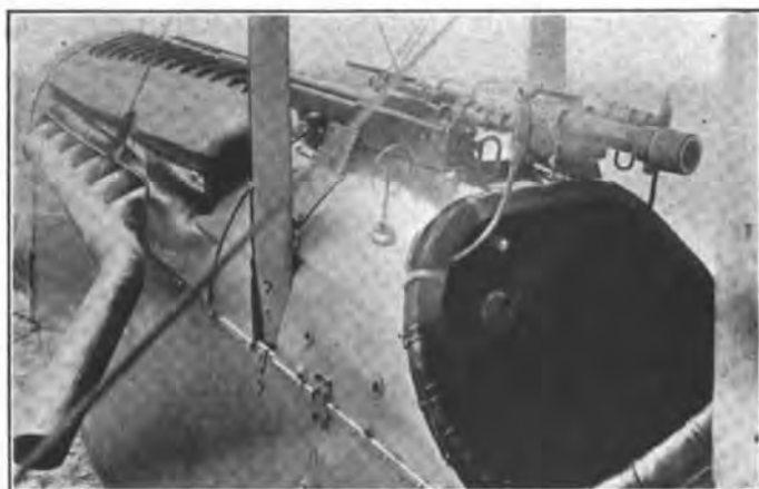
THE MOUNTING OF THE MACHINE GUN
