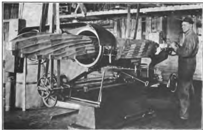
ROUGHING OUT THE DE HAVILAND-4 PROPELLER
