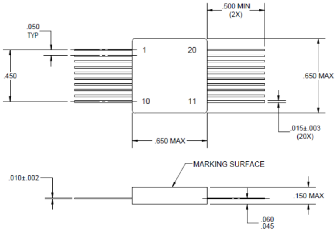
FIGURE 1 Model 1504 Package Outline
