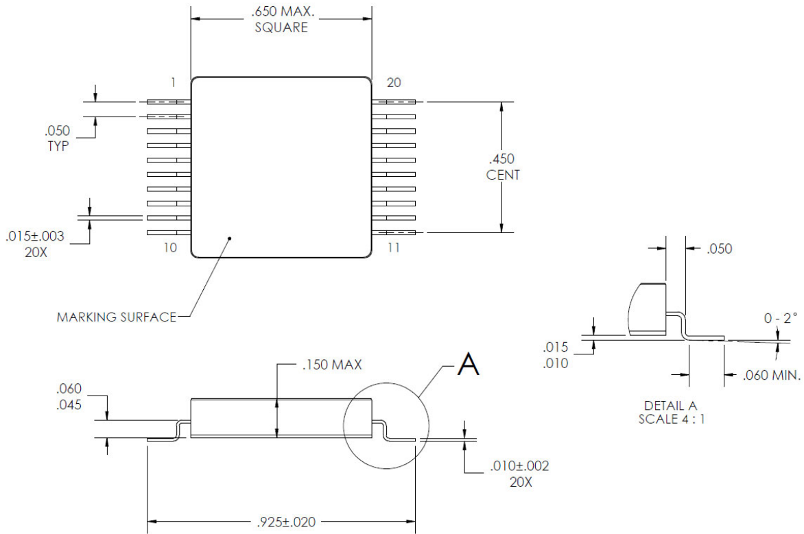
FIGURE 2 Models 1520 Package Outline
