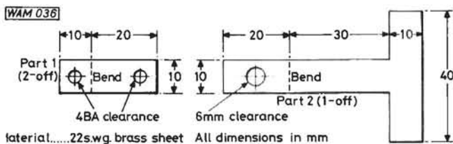
Fig. 8: Folded dipole feed terminal details
