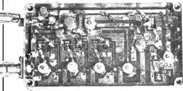
The Solent Scientific down-converter (reviewed in the February 1982 issue of PW ) provides full coverage of the 1.3GHz band and has an i.f. output in the u.h.f. TV bands
