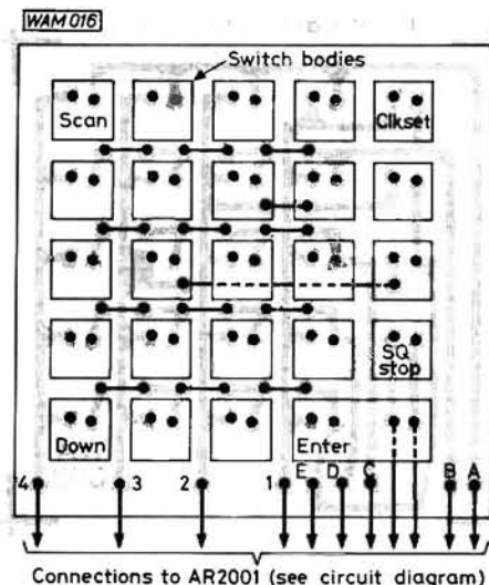
Fig. 3: Reduced scale layout of keyboard p.c.b. A full size paper track pattern is available for 30p from the editorial offices
