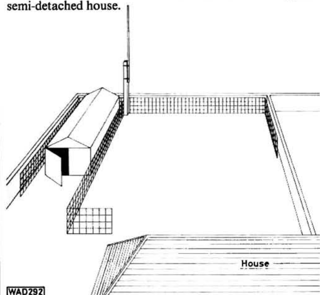
Fig. 1: Typical installation of antenna and earthing system
