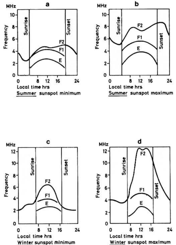
Fig. 3.1: Critical frequencies during 24 hours. A-B=summer and C-D=winter. Shaded areas are approximate hours of darkness
