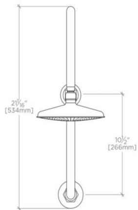
FRONT VIEW SCALE: \frac{1}{2} "=1'-0"
