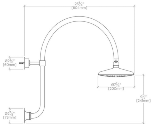
SIDE VIEW SCALE: \frac{1}{2} "=1'-0"
