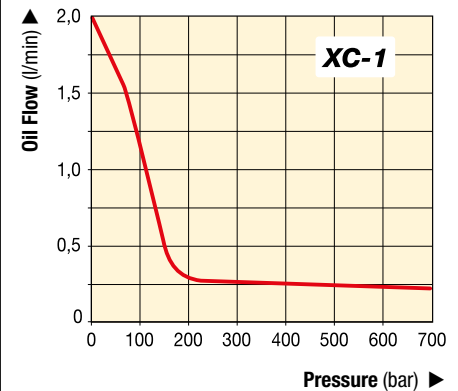
OIL FLOW vs. PRESSURE
