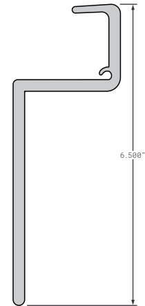
FCB040-806 REPLACES 03-6650-0-423 UTILITY STYLE 3000R REEFER 102" WIDE 1 PIECE WRAP AROUND
