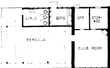
FLOOR PLAN
