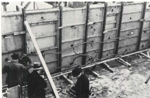
Plywood forms—4' wide and wall height—are placed, concrete poured and vacuum applied. Forms are held in place by compressive force of atmosphere. Concrete is consolidated by pressure, water taken off by vacuum.
