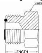
Male O-Ring Face Plug
