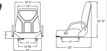
Part Number - 380070-023-E Seat with Electric Switch
