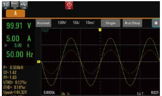
CC mode,CF=1.414
