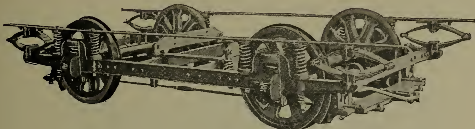
Fig. 5.— Photograph of Truck of the Single-Track Car.
