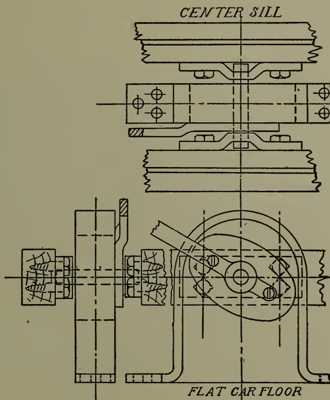
Fig. 182. — Detailed Sketch of Safety-Locking Device.
