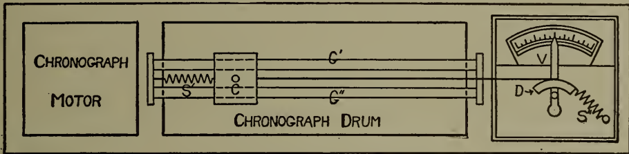
Fig. 27.—Speed Recording Mechanism.
