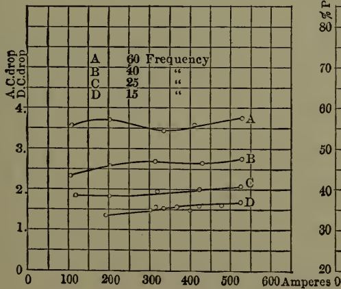
Fig. 148.—Variation of the Ratios \frac{A. C. Drop}{D. C. Drop} with Total Amperes. Single Track and Single Trolley.
