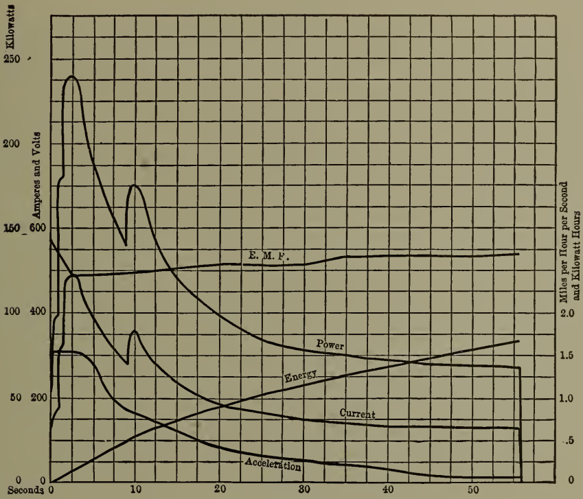
Fig. 71.—Electrical Data of Test No. 18.
