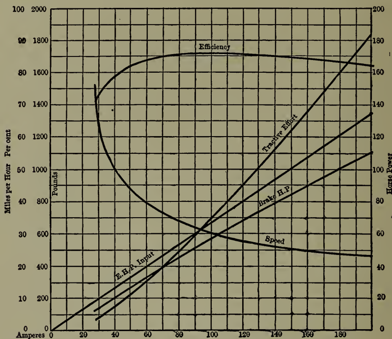
Fig. 47. — General Performance Curves of Westinghouse No. 8 Motors.
