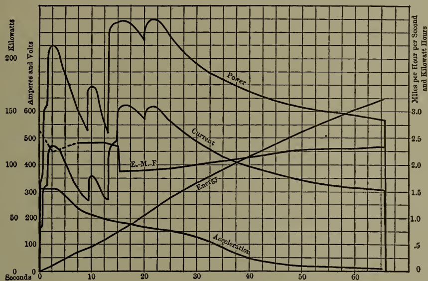
Fig. 73. — Electrical Data of Test No. 19.
