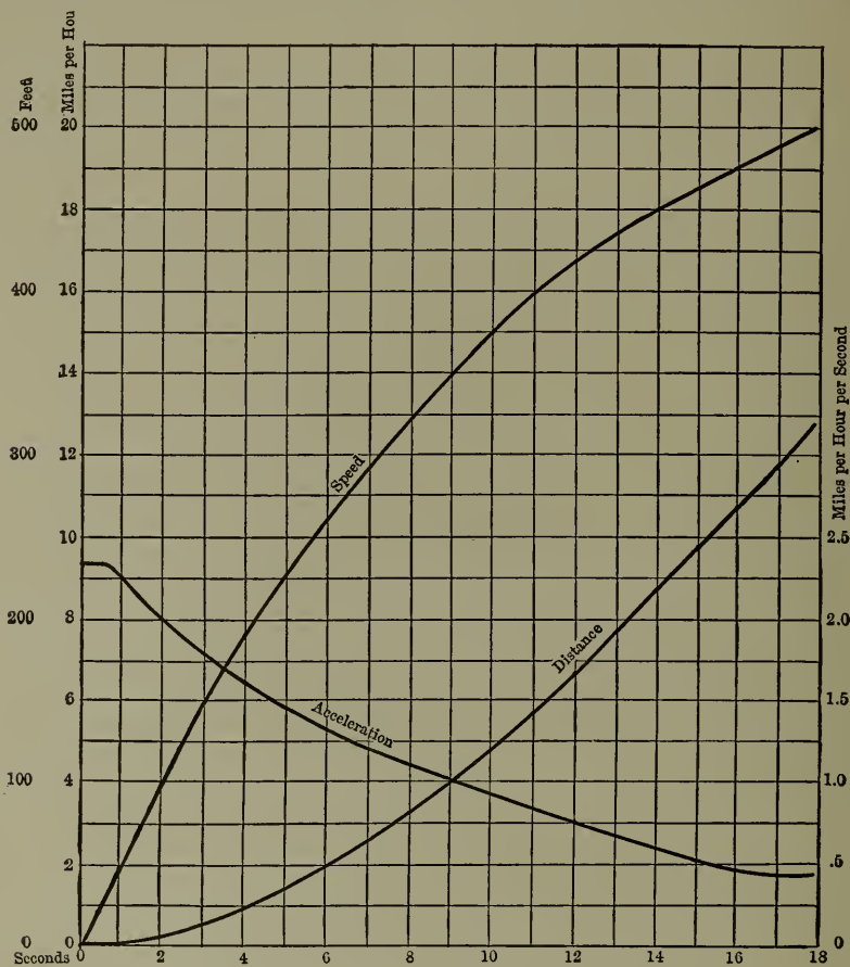
Fig. 62. — Speed and Distance Data, Test No. 15.
