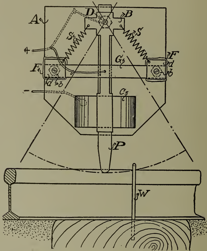
Fig. 55. — Contact Device for Distance Measurements. Acceleration Tests.
