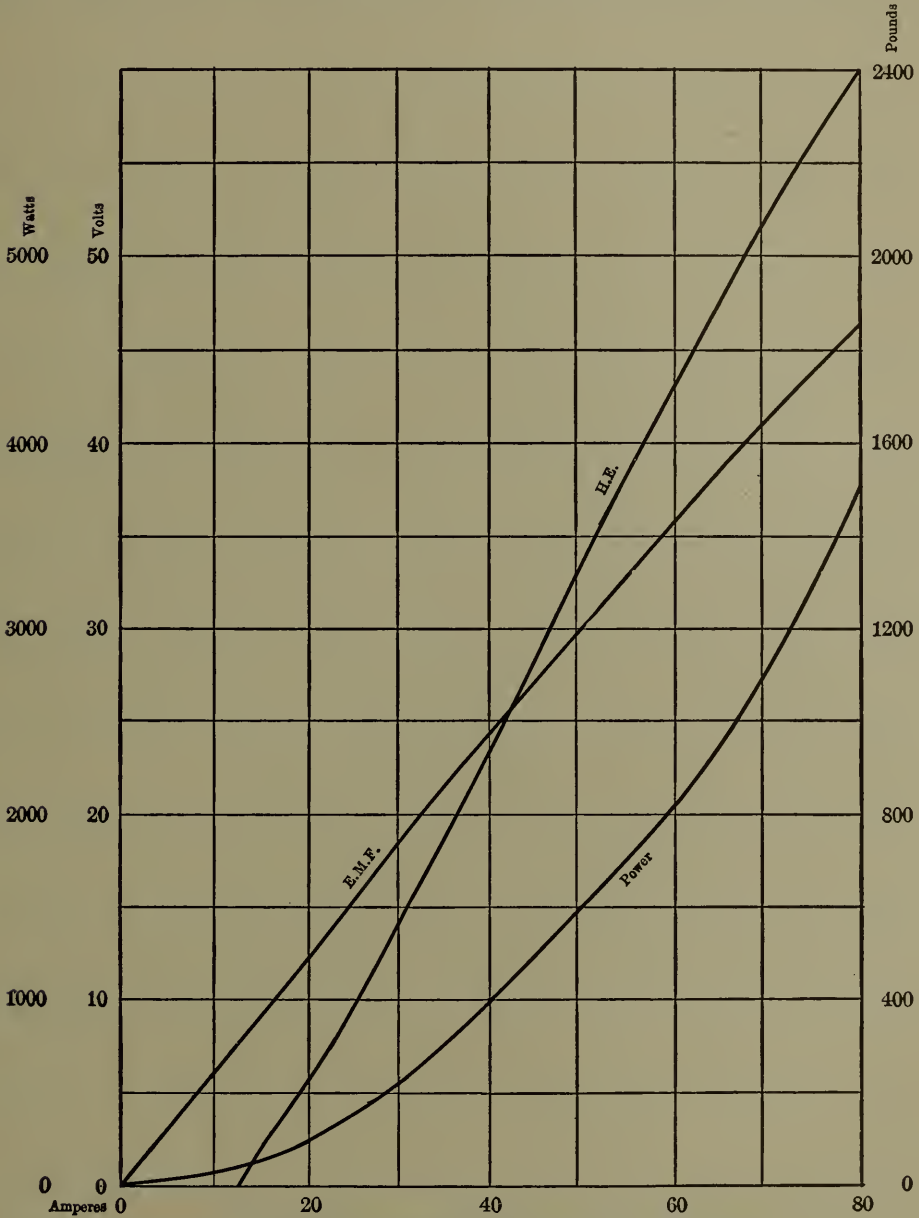
Fig. 106. — General Data, Industrial Locomotive Tests. Run No. 1.
