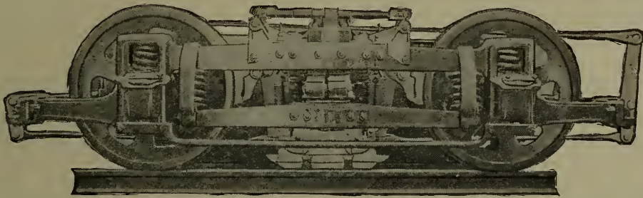
Fig. 9. — Westinghouse Magnetic Brake. (Side View.)
