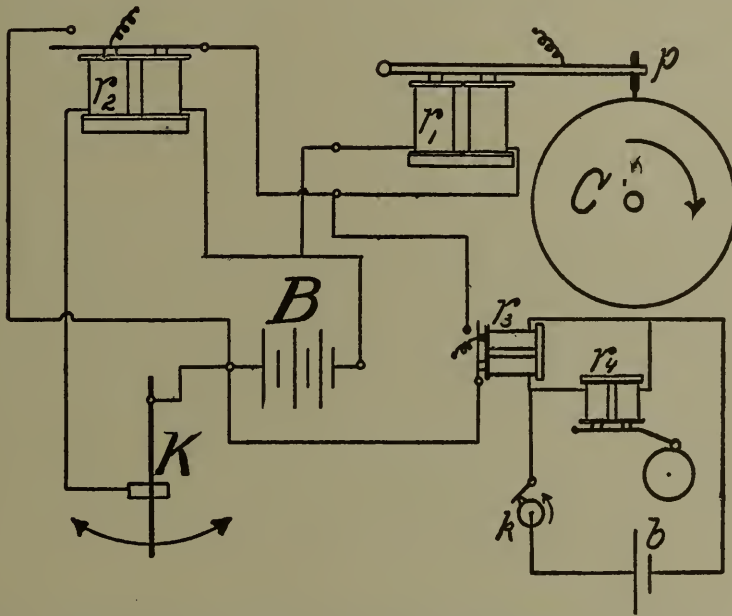
Fig. 56. — Relay Circuits for Time and Distance Measurements. Acceleration Tests.
