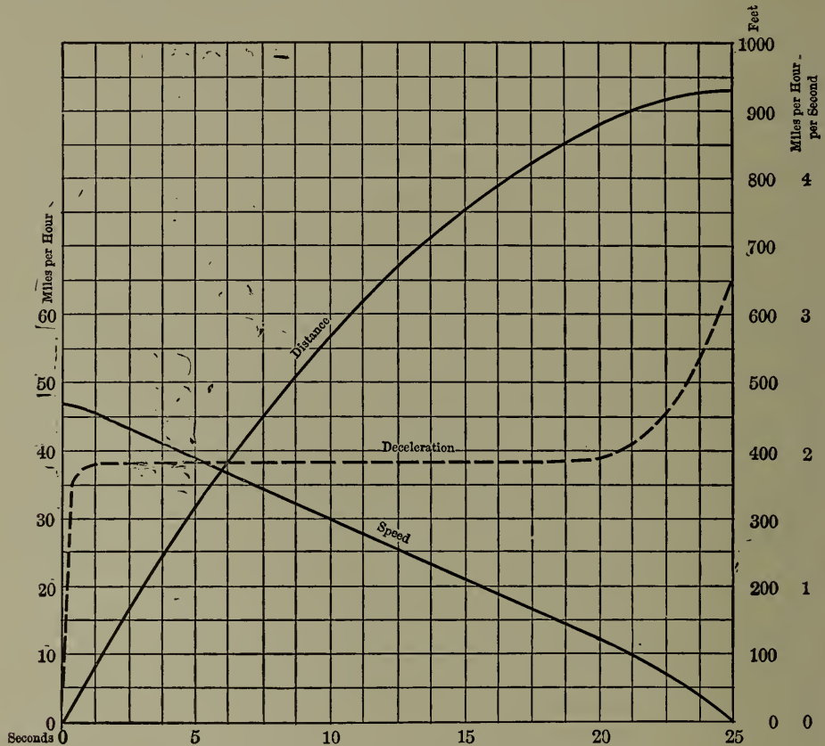
Fig. 91.—Speed and Distance Data. Test No. 31.
