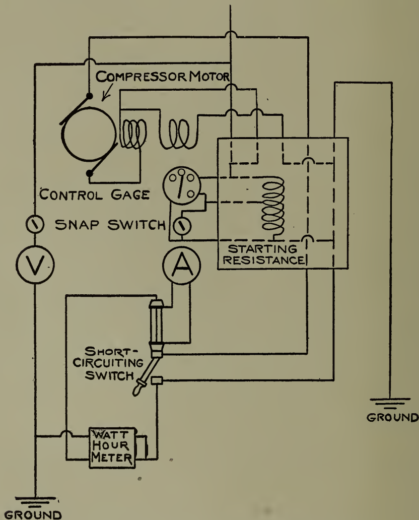
Fig. 79. — Electrical Connections for Tests of Compression Stations.
