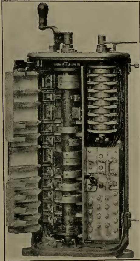
Fig. 16A.—General Electric Company, K. 28, Controller.
