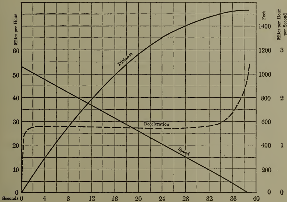
Fig. 90.— Speed and Distance Data. Test No. 30.
