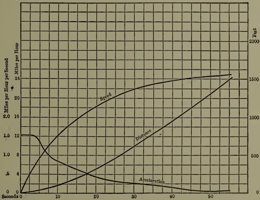
Fig. 72.—Speed and Distance Data, Test No. 18.
