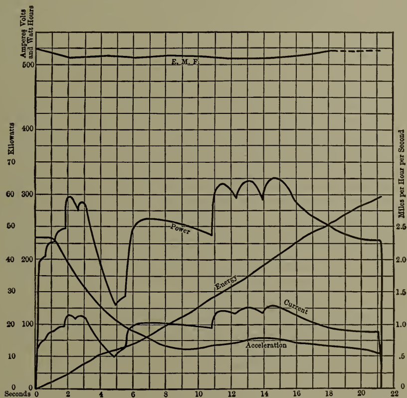
Fig. 65. — Electrical Data of Test No. 17.
