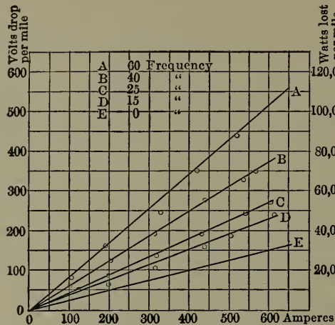
Fig. 138. — Variation of Pressure Drop per Mile with Total Amperes. Double Track and Trolley.
