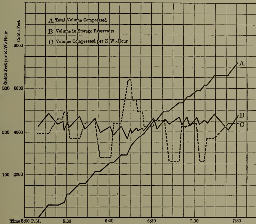
Fig. 83. — General Air Data of Test No. 21.
