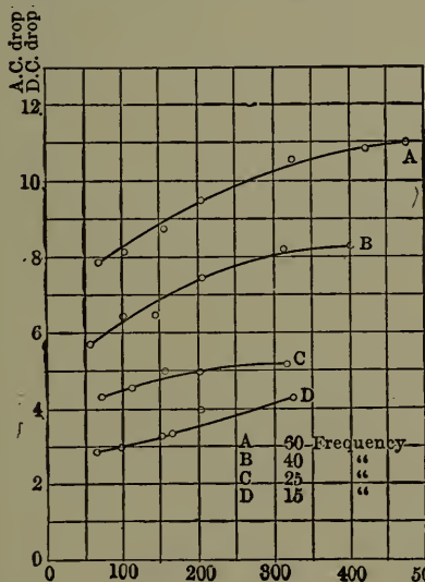
Fig. 160. — Variation of Ratio \frac{A.C. Drop}{D.C. Drop} with Total Current, Single Rail.
