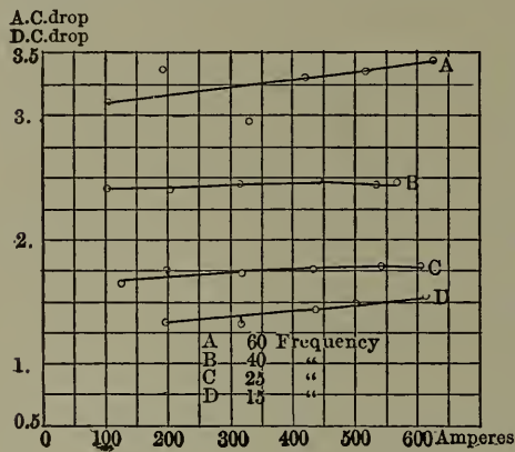
Fig. 140. — Variation of Rates \frac{A.C. Drop}{D.C. Drop} with Total Amperes. Double Track and Trolley.
