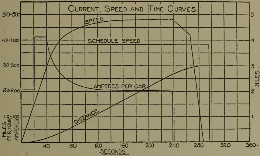
Fig. 1. — Currents, Speed and Time Curves.
