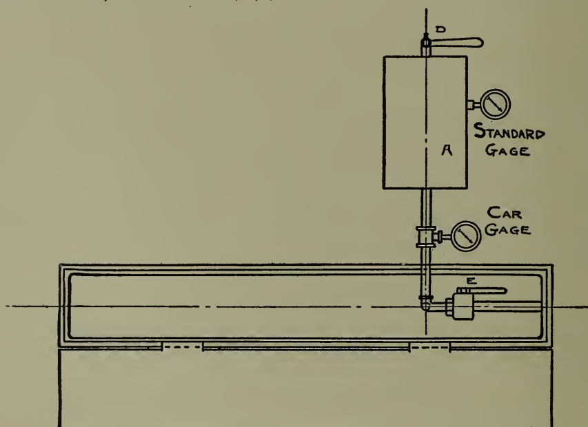
Fig. 80.—Connection for Calibrating Car Gages.
