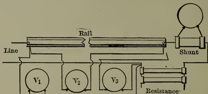
Fig. 116. — Diagram of Connections for A. C. Rail Tests.
