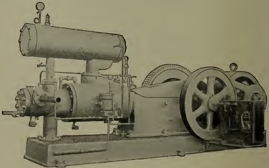
Fig. 77.—Station Compressor and Motor, Showing Controller.
