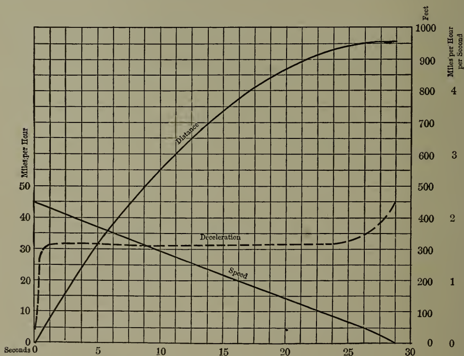
Fig. 89. — Speed and Distance Data. Test No. 29.
