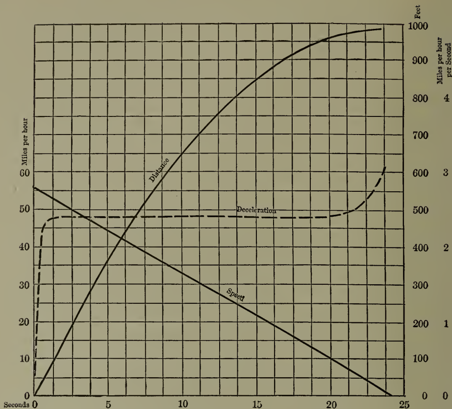
Fig. 93.—Speed and Distance Data. Test No. 33.
