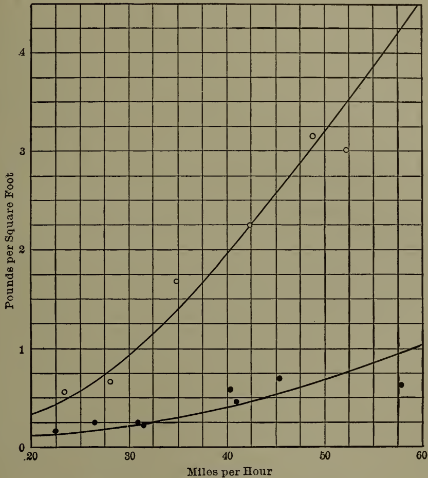
Fig. 202.—Air Resistance Curves for Standard Vestibule.
