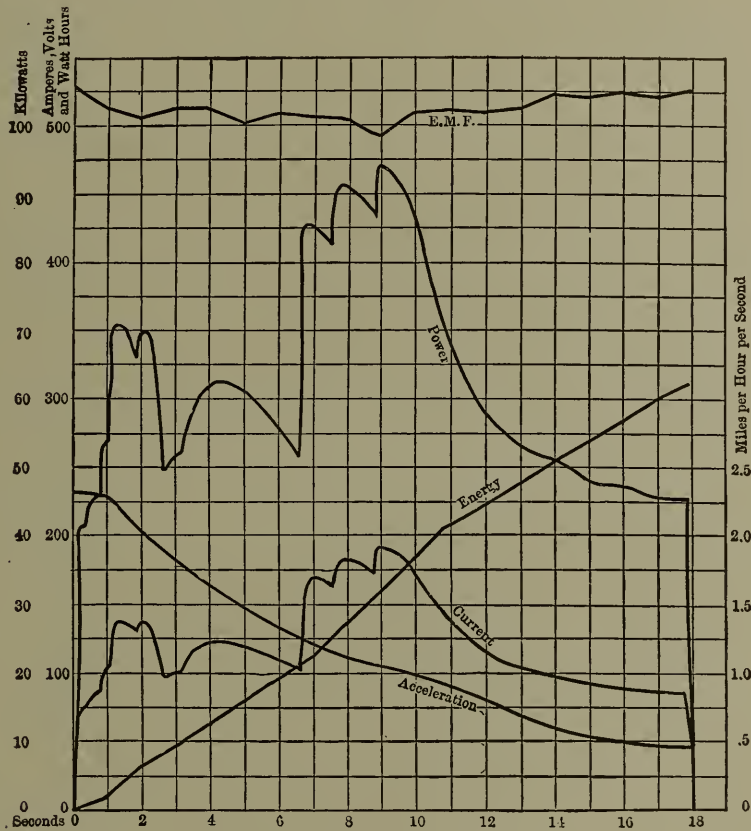
Fig. 61.—Electrical Data of Test No. 15.
