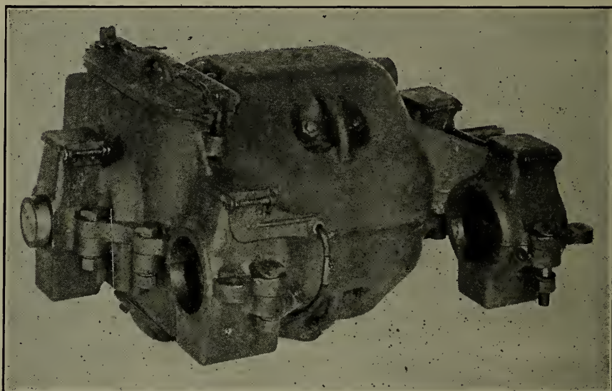
Fig. 15.—General Electric Company, Type 54, Motor.
