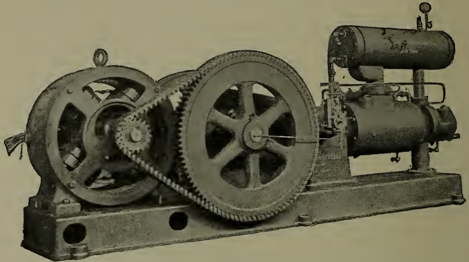
Fig. 76.—Station Compressor and Motor, Showing Gear Case Removed.
