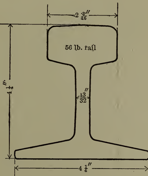
Fig. 119. — Section of 55 lb. Rail A. C. Tests.
