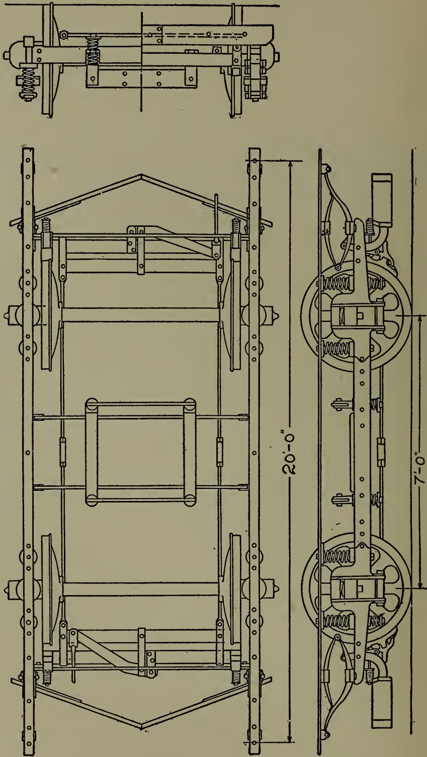
Fig. 6. — Drawing of Truck of the Single-Track Car.
