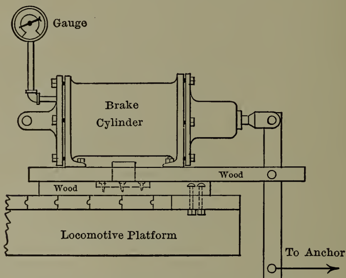
Fig. 105.—Oil Dynamometer. Industrial Locomotive.
