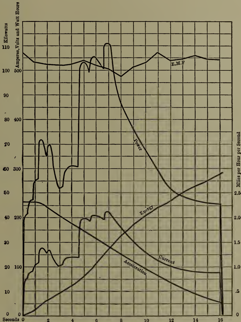
Fig. 59. — Electrical Data of Test No. 14.
