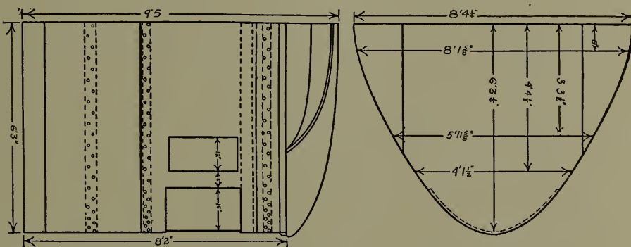
Fig. 173. — Sketch of "Parabolic" Movable Vestibule.
