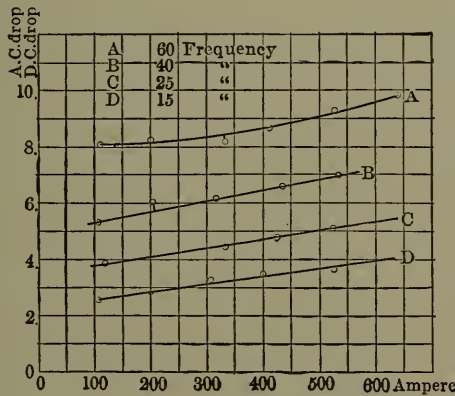
Fig. 152. — Variation of \frac{\text{A. C. Drop}}{\text{D. C. Drop}} with Total Current. Single Track Alone.
