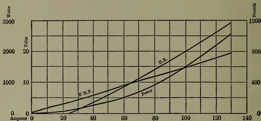
Fig. 111.—General Data, Industrial Locomotive Tests. Run No. 6.
