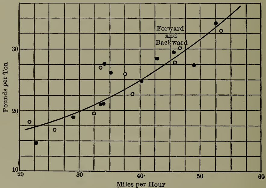
Fig. 166. — Resistance Curves, Test No. 52. Car No. 284.
