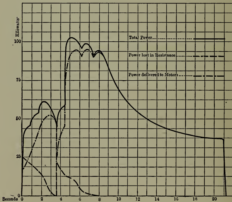
Fig. 32. — Division of Power, Test No. 2, Sept. 24, 1904.
