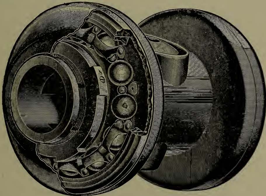
Fig. 184. — General View Chapman Double-Ball Bearing.
