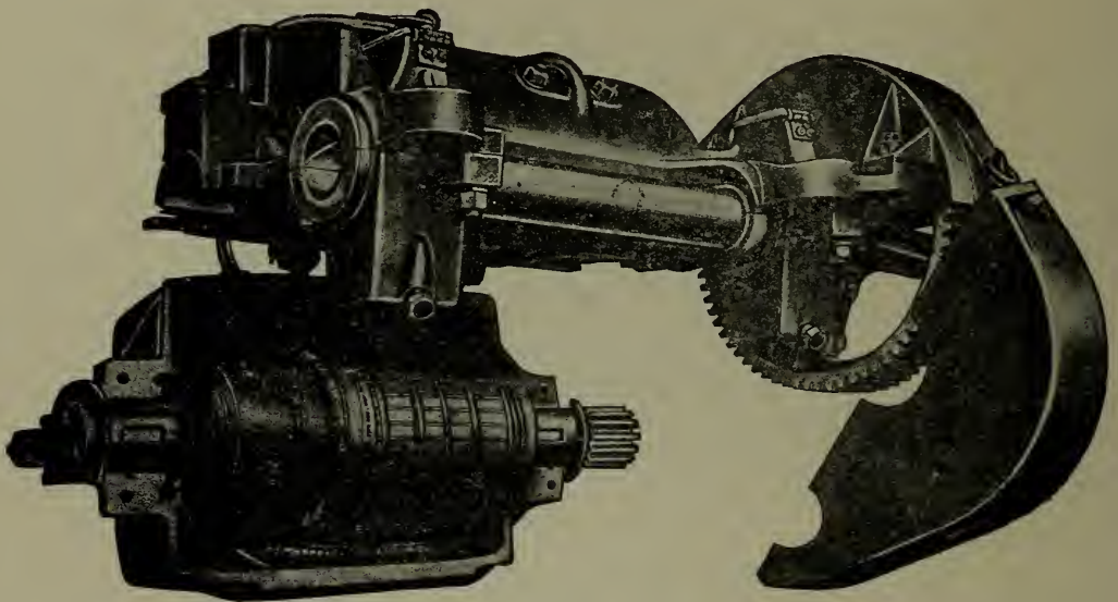
Fig. 8. — Westinghouse No. 56 Motor. (Motor open.)
