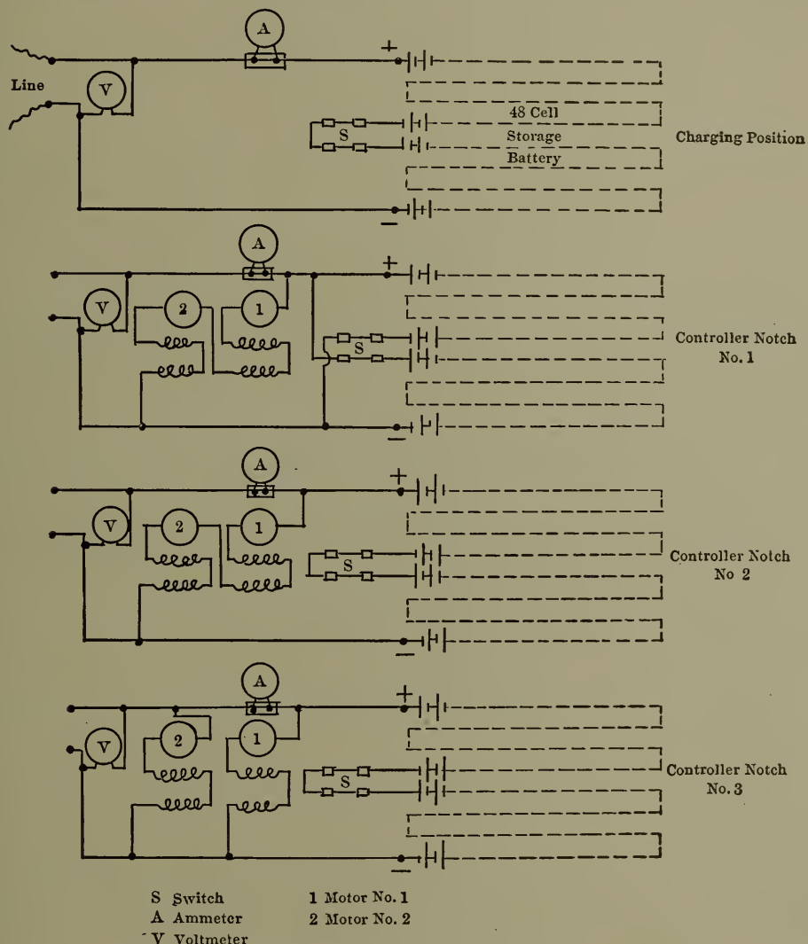
Fig. 104.—Diagram of Connections Industrial Locomotives.
