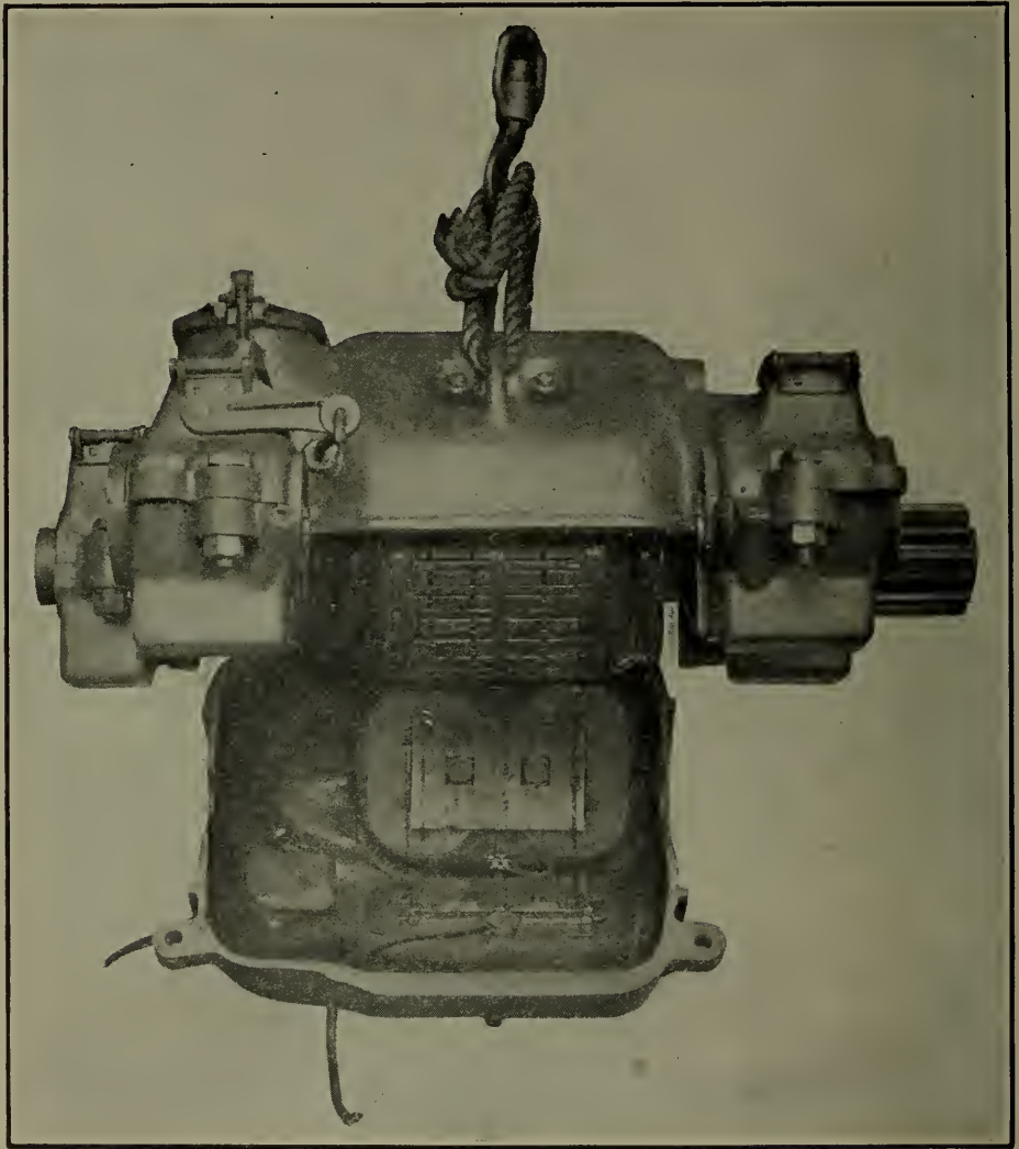
Fig. 16. — General Electric Company, Type 54, Motor.
