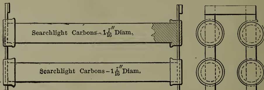
Fig. 115. — Carbon Resistance for A. C. Rail Tests.
