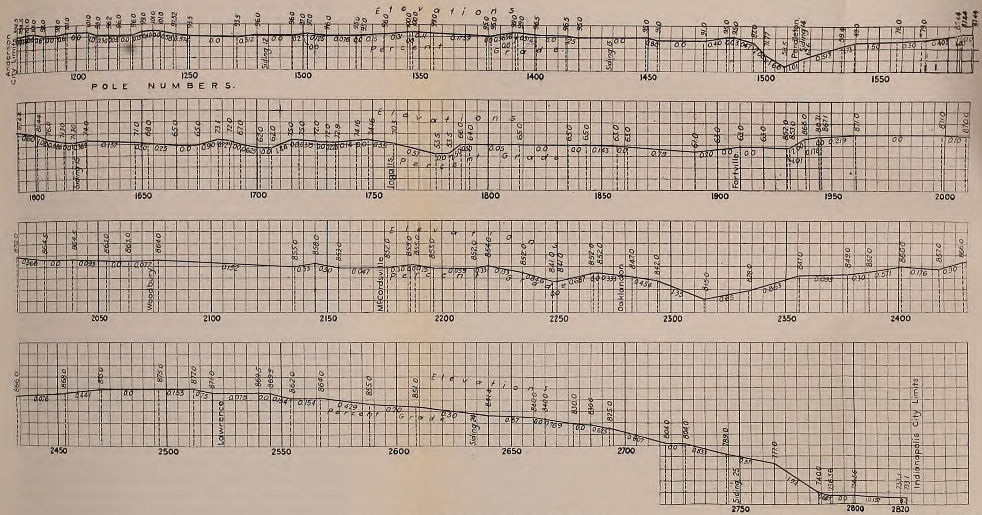
FIG. 53 B.—Profile between Anderson and Indianapolis.
