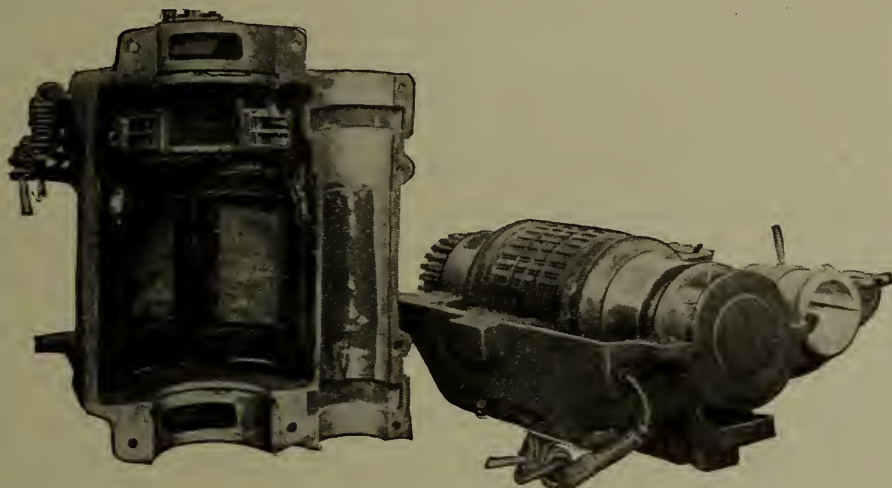
Fig. 23.— Westinghouse No. 85 Motor. (Showing Parts.)
