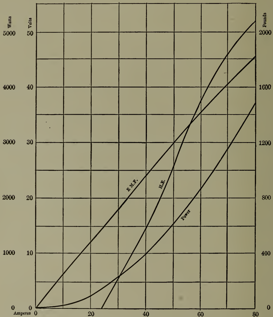
Fig. 107.—General Data, Industrial Locomotive Tests. Run No. 2.
