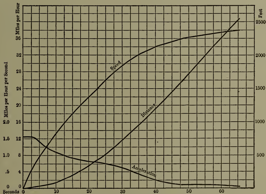
Fig. 74. — Speed and Distance Data of Test No. 19.
