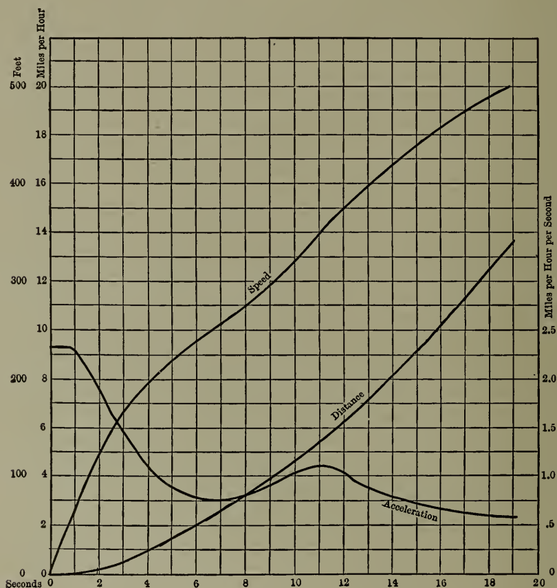
Fig. 64. — Speed and Distance Data, Test No. 16.
