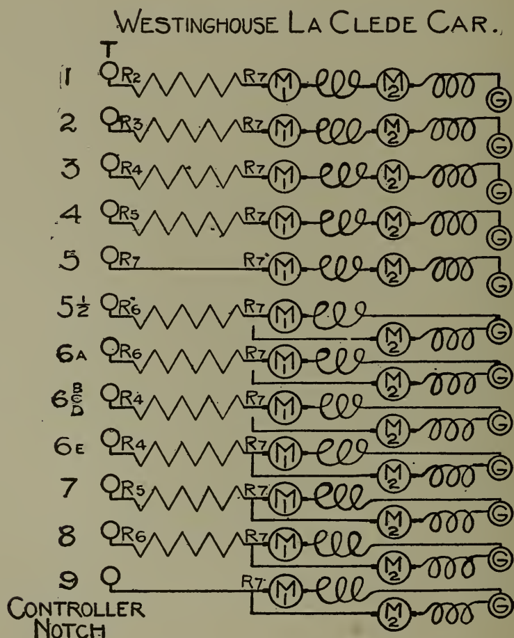
Fig. 54. — Connections of Power Notches of Controller, Single-Truck City Car.
