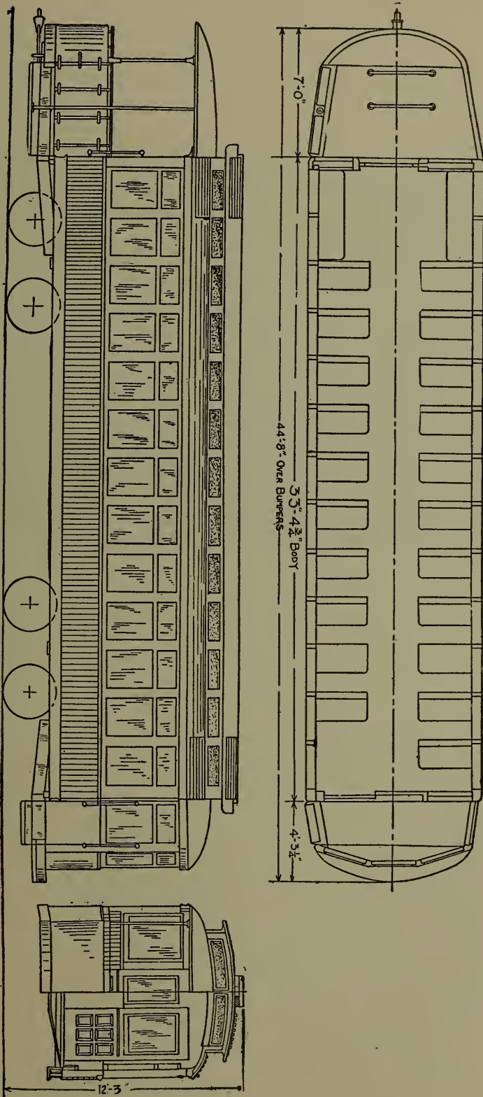
Fig. 12. — General Drawing of Double-Truck City Car.
