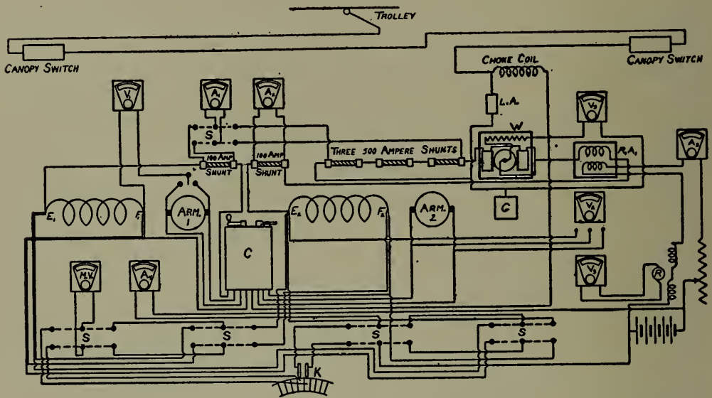
Fig. 29. — Diagram of Connections of Instruments. (Single-Truck Car.)
