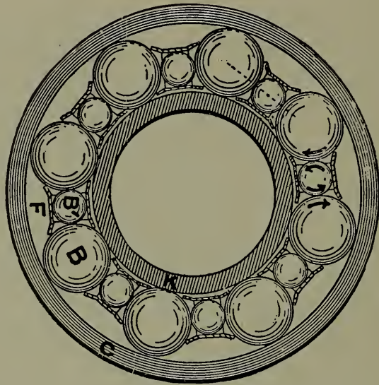
Fig. 185. — Pressed Steel Duct-Ring of Chapman Double-Ball Bearing.
