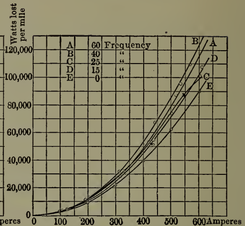
Fig. 139. — Variation of Watts Lost per Mile with Total Amperes. Double Track and Trolley.
