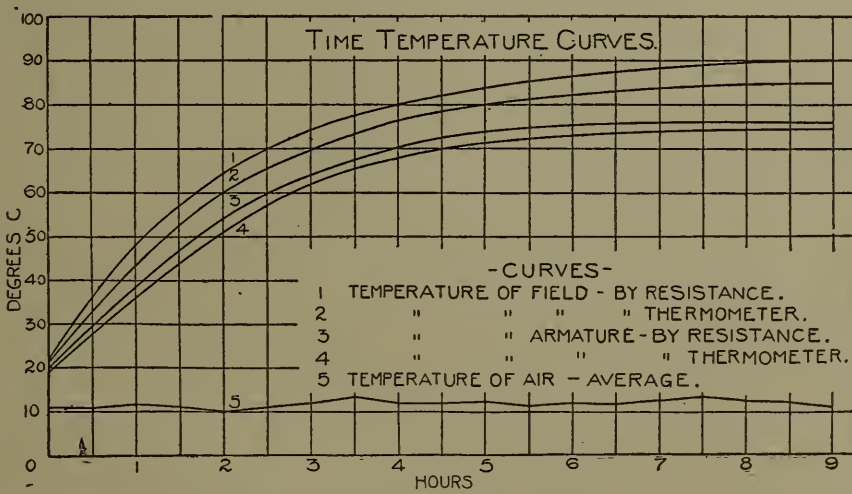
Fig. 2. — Time Temperature Curves.
