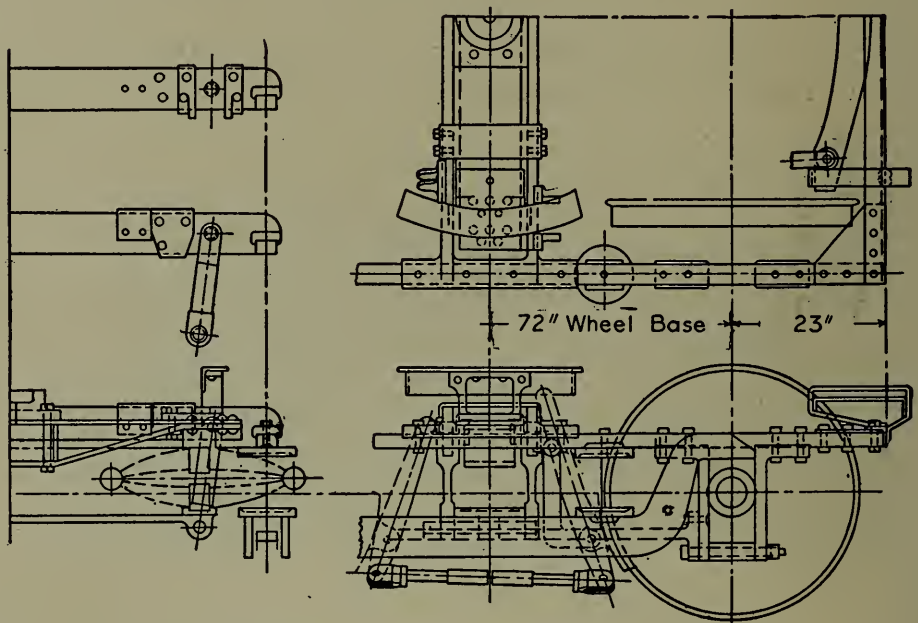
Fig. 21.—General Drawing of Baldwin Truck for Car 284.
