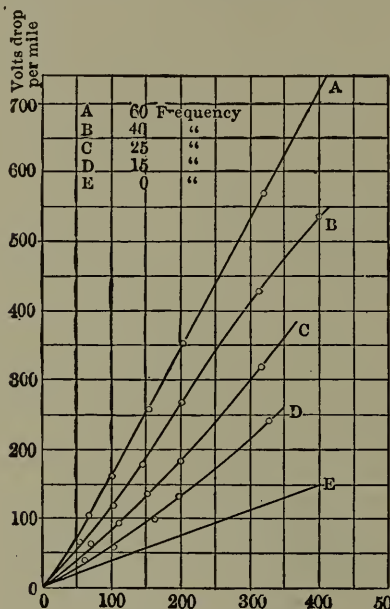
Fig. 154. — Variation of Pressure Drop with Total Current. Single Rail and Single Trolley.
