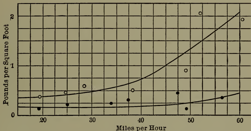
Fig. 199.—Air Resistance Curves for Parabolic Wedge Vestibule.
