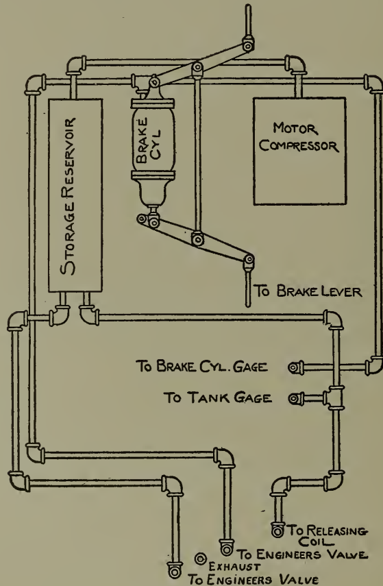
Fig. 84. — Piping of Car 2600, Equipment with Motor Compressor.
