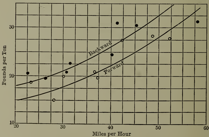
Fig. 170. — Resistance Curves, Test No. 57. Car Louisiana with Standard Front and no Rear Vestibule.
