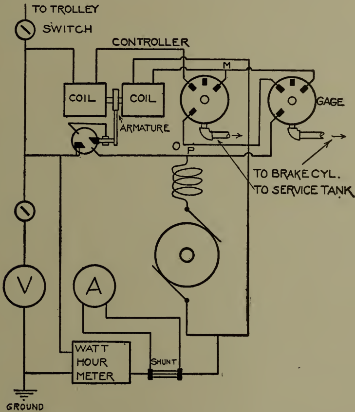
Fig. 85. — Diagram of Connections, Independent Motor, Compressor System.
