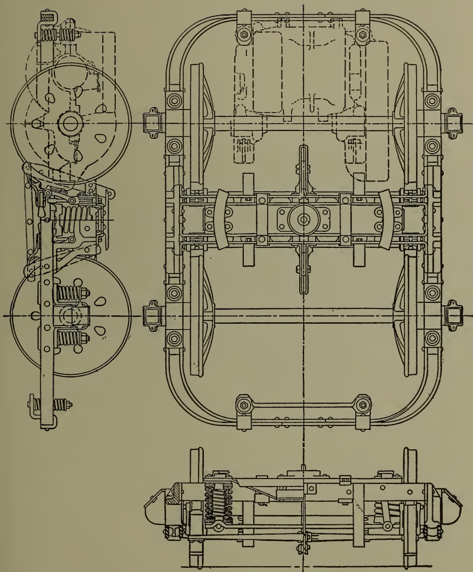
Fig. 14.—General Drawing of St. Louis Transit Company Car Truck.
