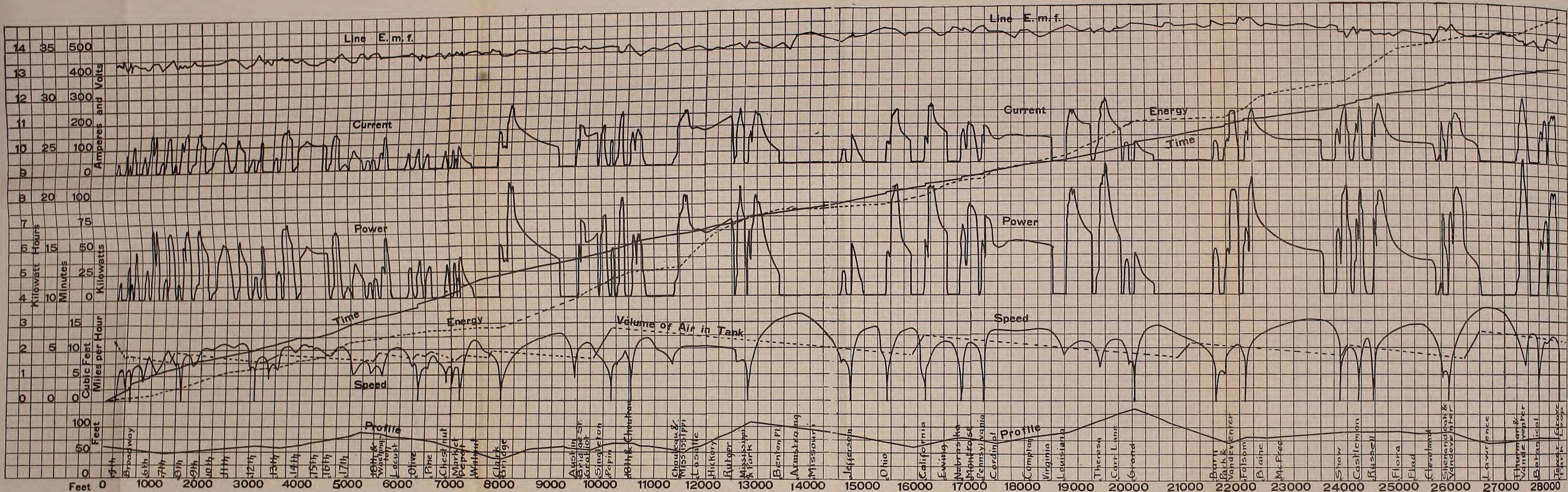
FIG. 87—Graphical Log of One-Half Trip on Park Ave. Line, St. Louis, Mo
