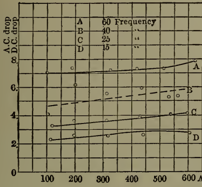
Fig. 144.—Variation of Power \frac{A. C. Drop}{D. C. Drop} with Total Amperes. Double Tracks.
