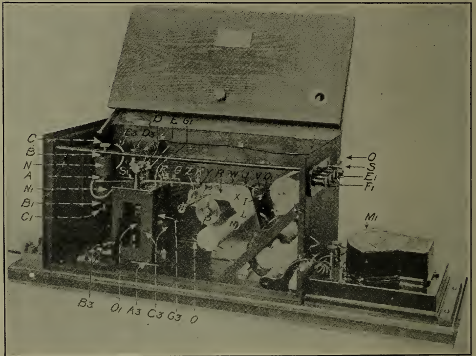
Fig. 24. — General Electric Company's Recording Ammeter.
