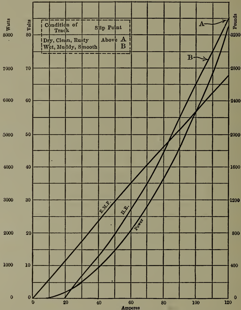
Fig. 109.—General Data, Industrial Locomotive Tests. Run No. 4.
