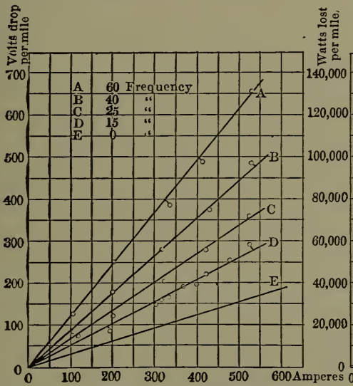
Fig. 146.—Variation of Pressure Drop per mile with Total Amperes. Single Track and Trolley.
