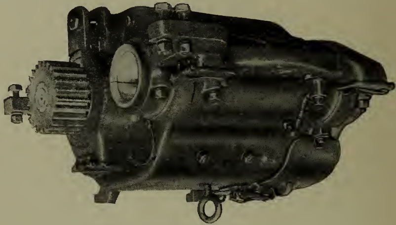
Fig. 22. — Westinghouse No. 85 Motor. (General View.)
