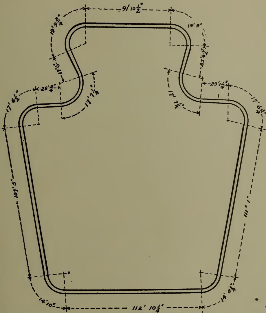
Fig. 103.—General Arrangement of Track. Industrial Locomotive.
