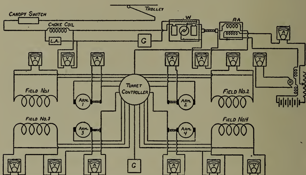
Fig. 50.—Diagram of Connections, Interurban Car Service Tests.
