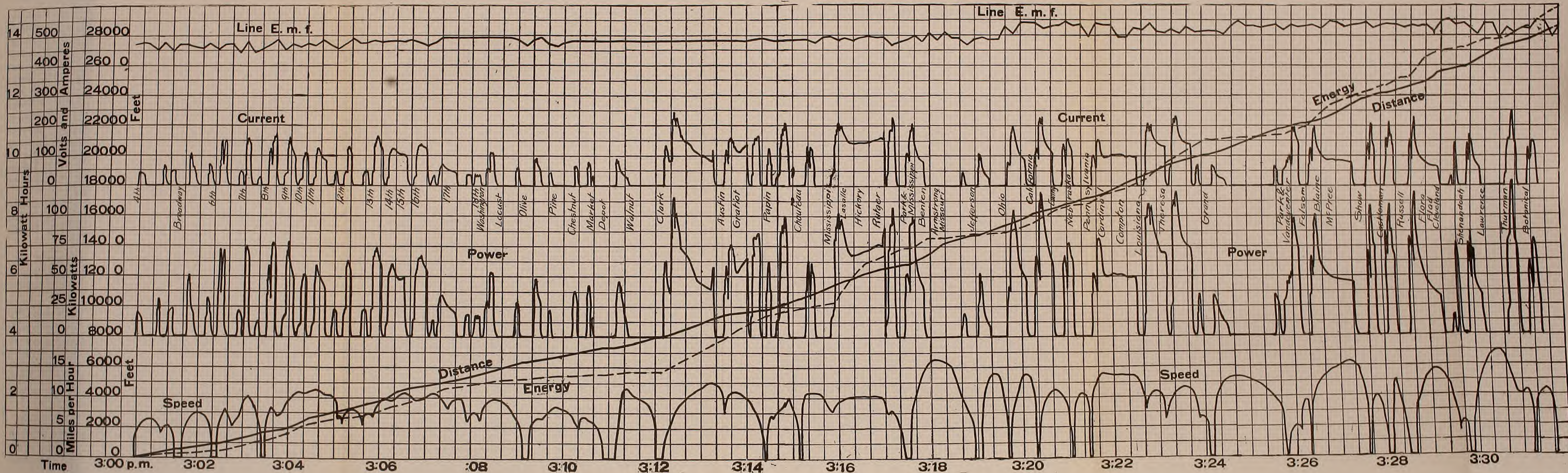
FIG. 45.—Graphical Log of One-Half Trip on Park Ave. Line, St. Louis, Mo.
