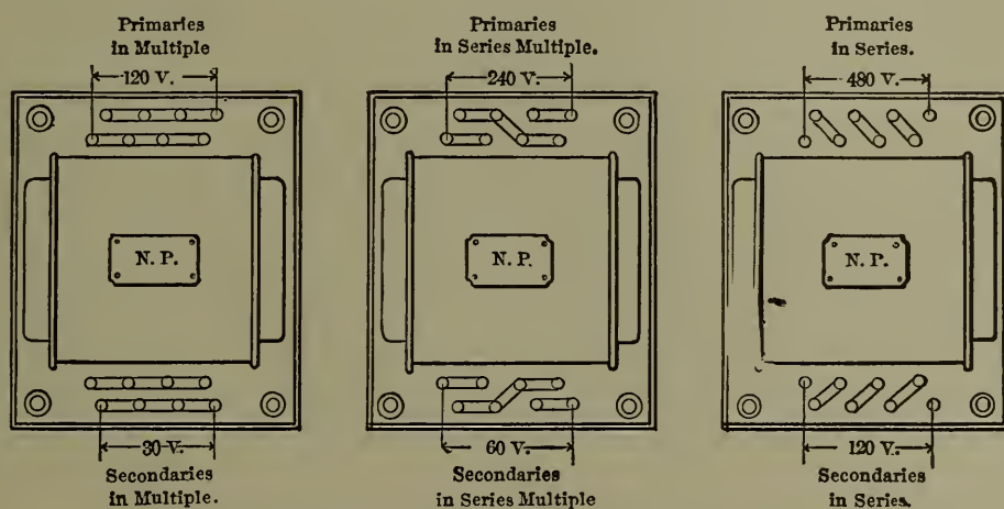
Fig. 114. — Pressure Transformers Connections for A. C. Tests.
