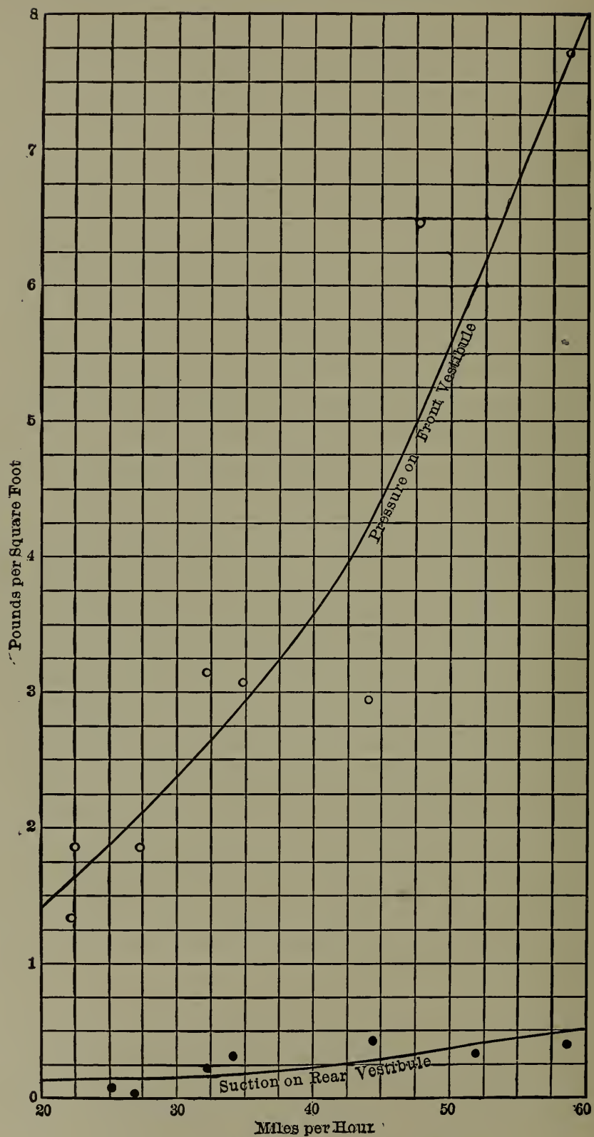
Fig. 201. — Air Resistance Curves for Flat Vestibule.
