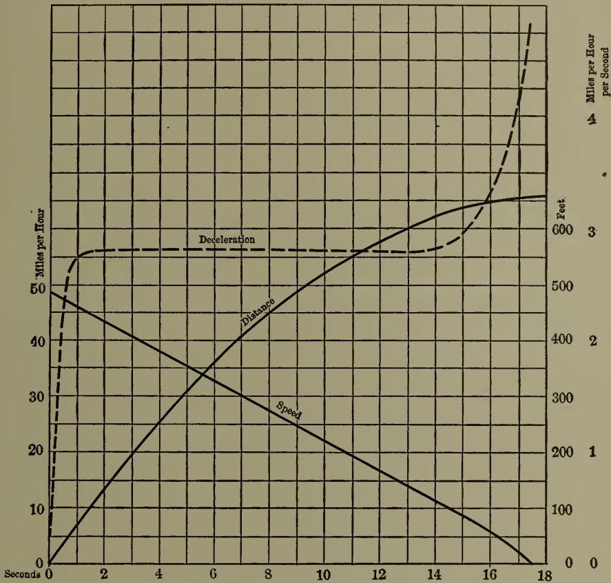
Fig. 92. — Speed and Distance Data. Test No. 32.
