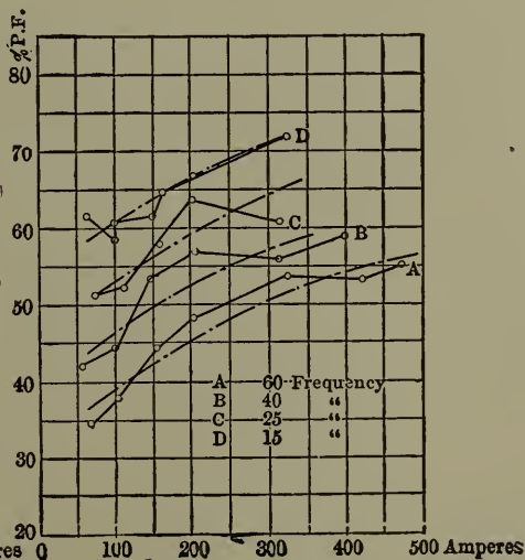
Fig. 161. — Variation of Power Factor with Total Current, Single Rail Alone.
