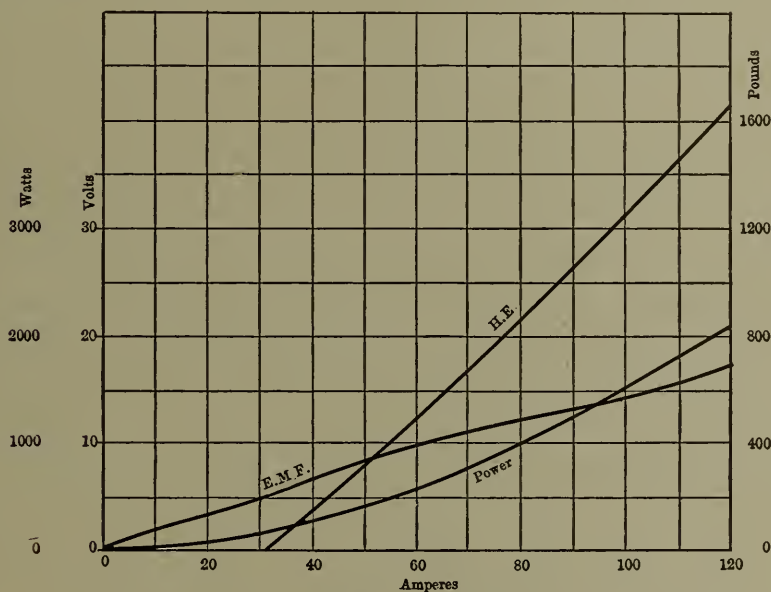
Fig. 110.—General Data, Industrial Locomotive Tests. Run No. 5.
