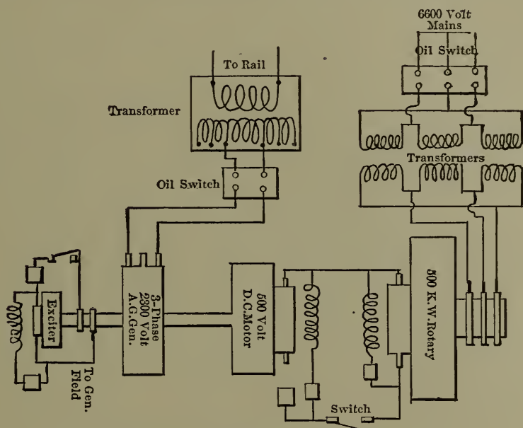
Fig. 112. — Diagram of Connections for A. C. Tests.
