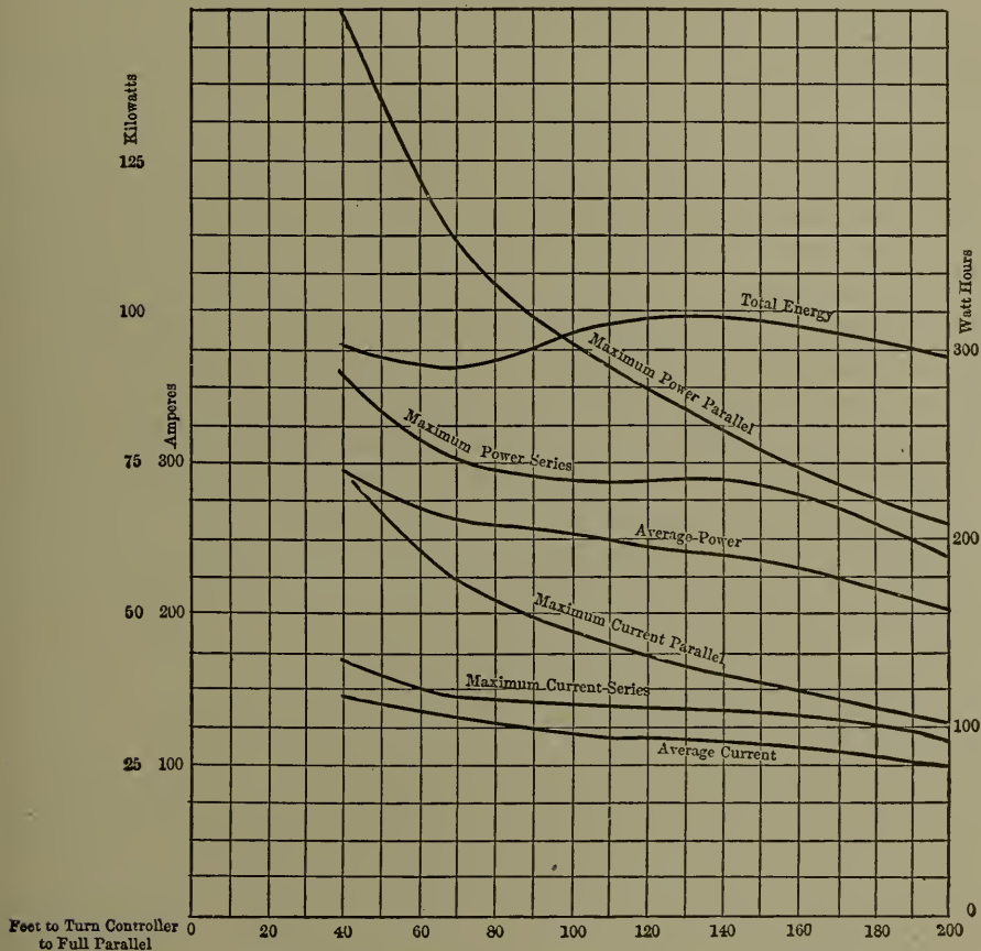
Fig. 67.—Summary of Electrical Data, Acceleration Tests of Single-Track Car.
