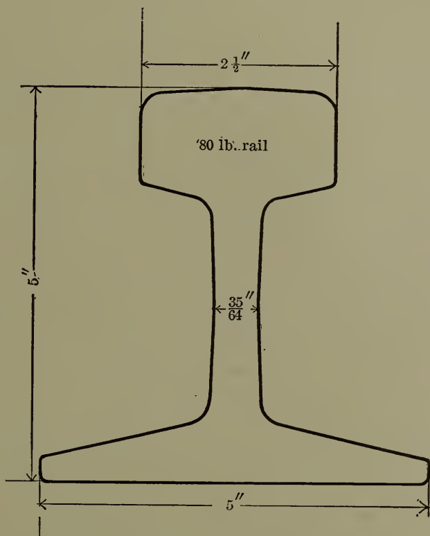
Fig. 128.—Section of 80 lb. Rail, A. C. Rail Tests.
