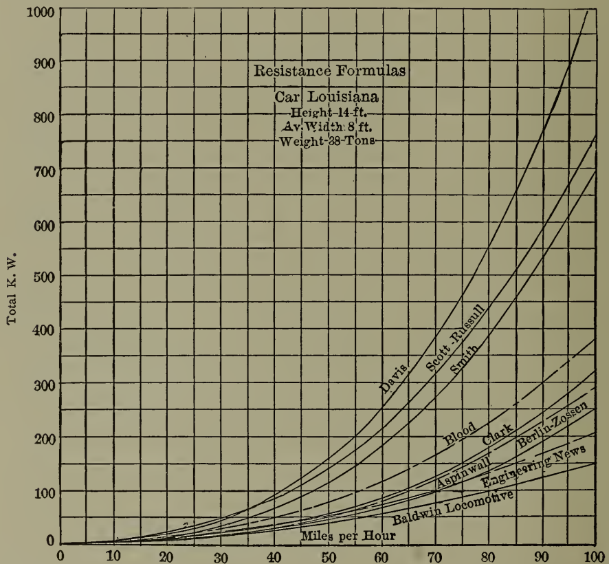
Fig. 163. — Application of Train Resistance Formulas to Car Louisiana (Results Shown in Kilowatts Lost at Various Speeds).
