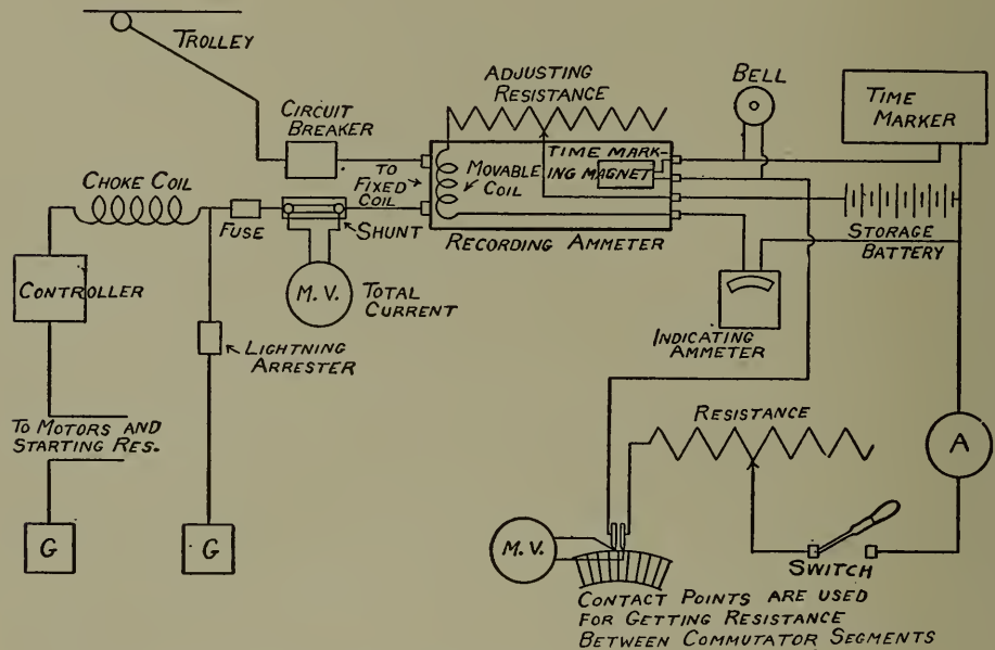
Fig. 44. — Diagram of Connections, Service Tests of Double-Truck City Car.
