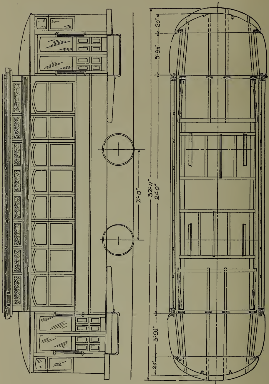
Fig. 4. — General Drawing of the Single-Truck Car.
