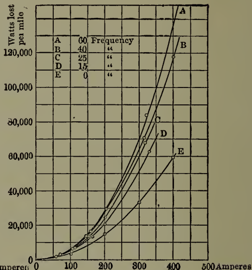
Fig. 155. — Variation of Power Lost with Total Current. Single Rail and Single Trolley.
