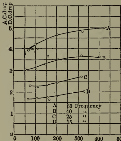
Fig. 156. — Variation of Ratio \frac{A. C. Drop}{D. C. Drop} Single Rail and Single Track.
