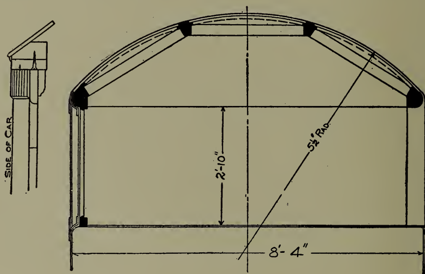
Fig. 189. — Detailed Sketch of "Standard" Vestibule.
