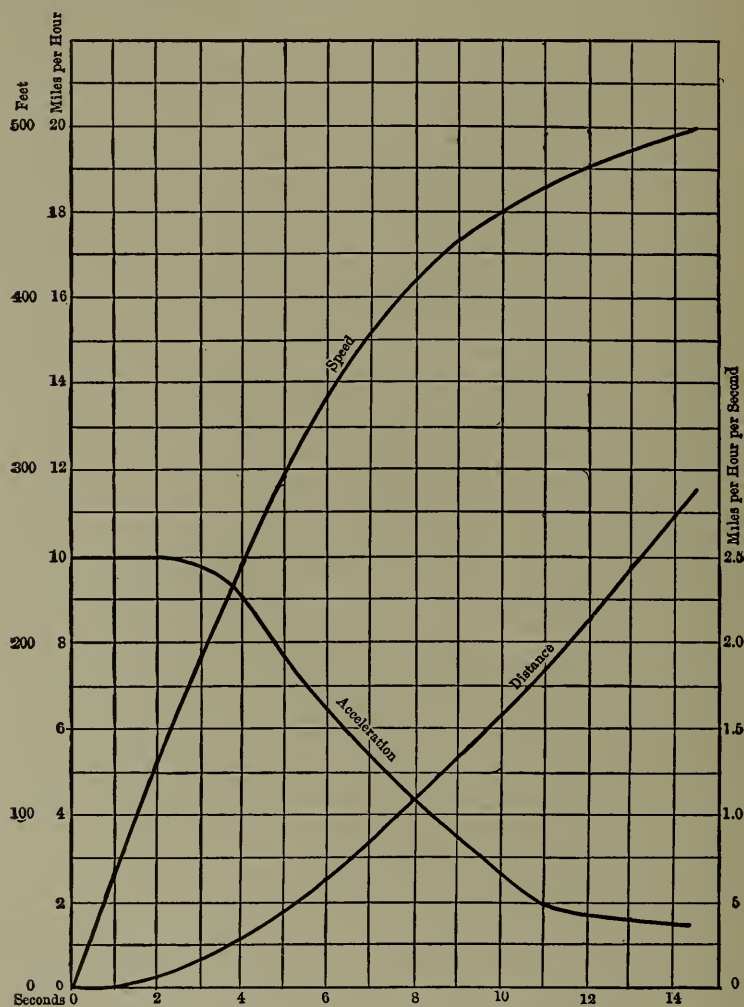
Fig. 58. — Speed and Distance Data, Test No. 13.
