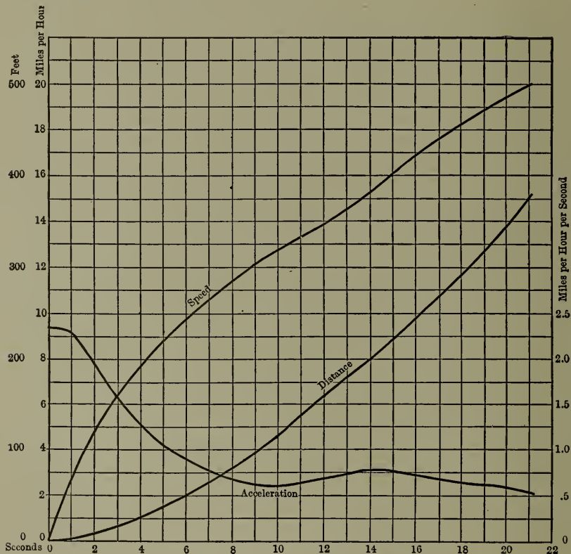
Fig. 66. — Speed and Distance Data, Test No. 17.
