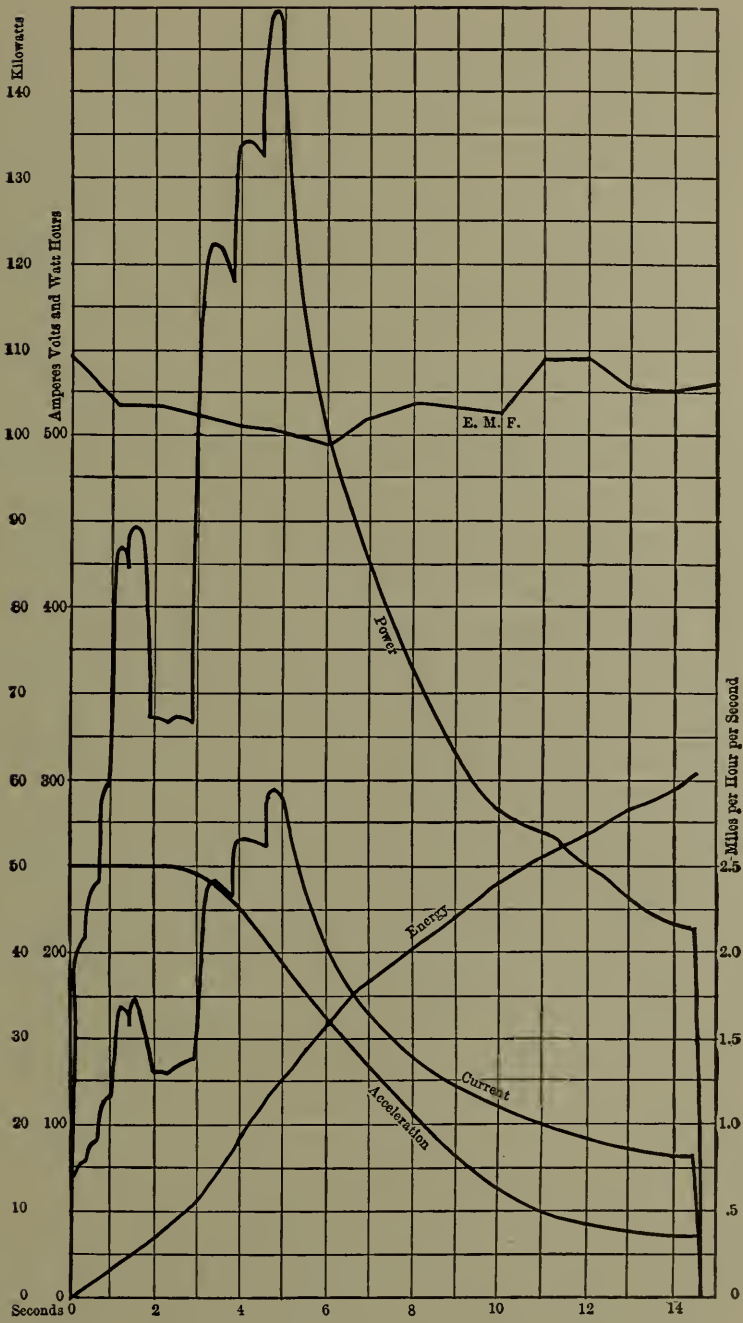
Fig. 57. — Electrical Data of Test No. 13.
