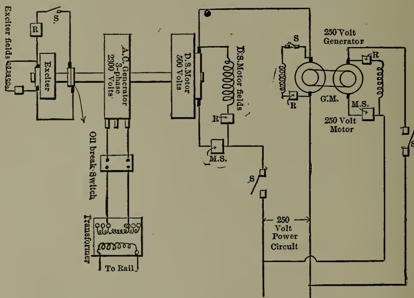
Fig. 113. — Diagram of Connections for A. C. Tests.
