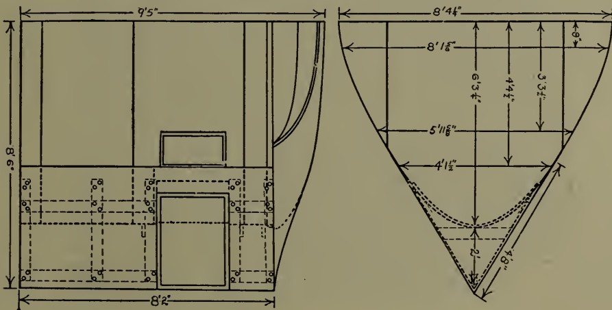
Fig. 175.—Sketch of "Parabolic Wedge" Movable Vestibule.
