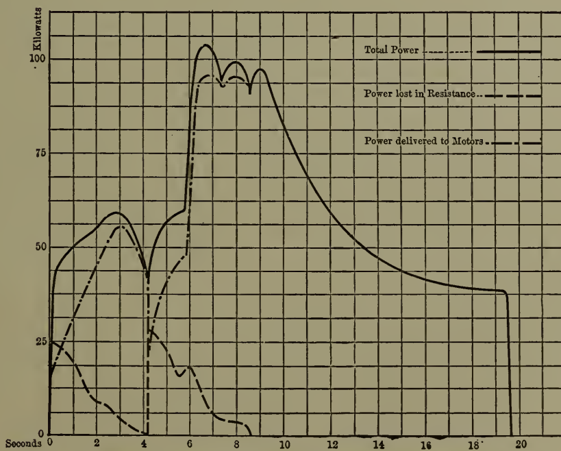
Fig. 41. — Division of Power in Test No. 5, Oct. 7, 1904.
