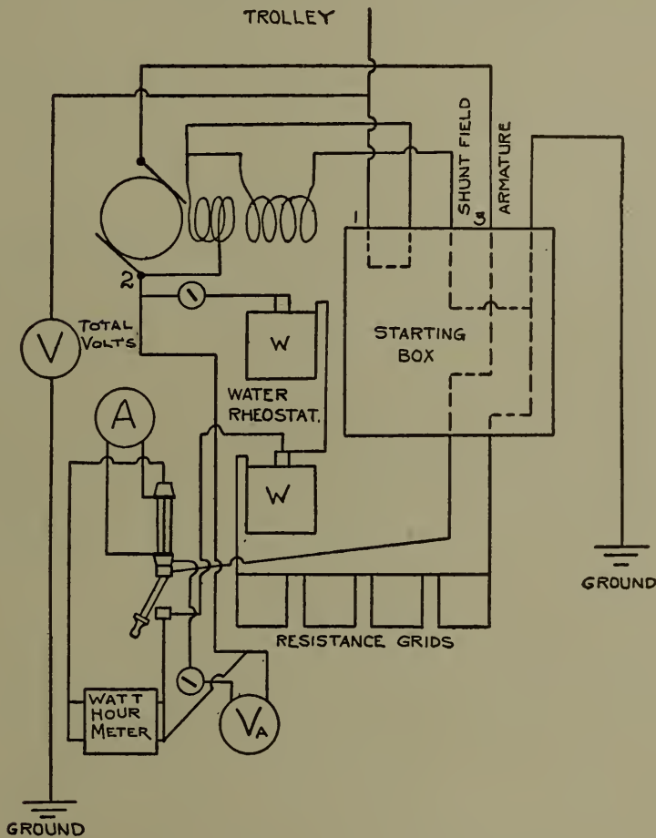
Fig. 81.—Connection for Electrical Measurements of Motor Losses.
