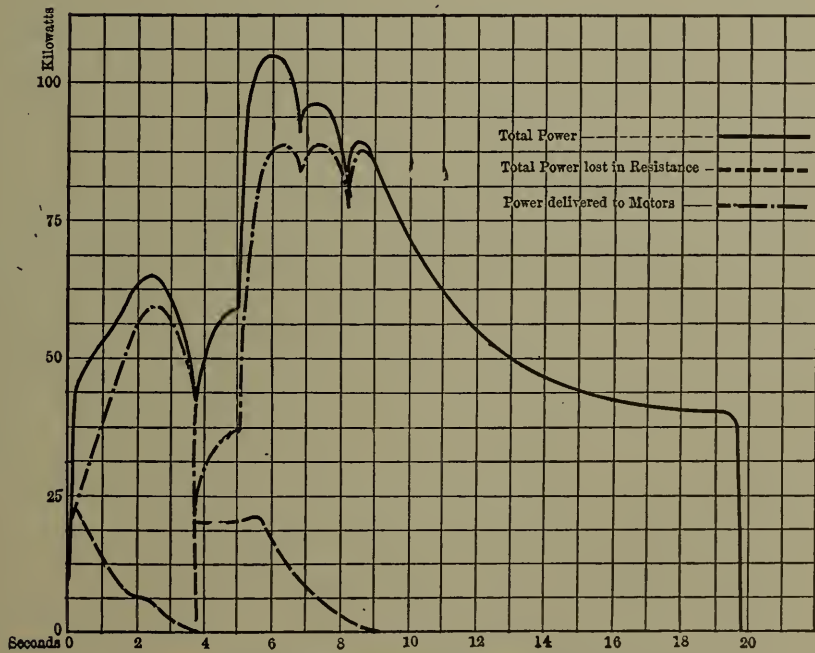
Fig. 38.—Division of Power In Test No. 4, Oct. 6, 1904.
