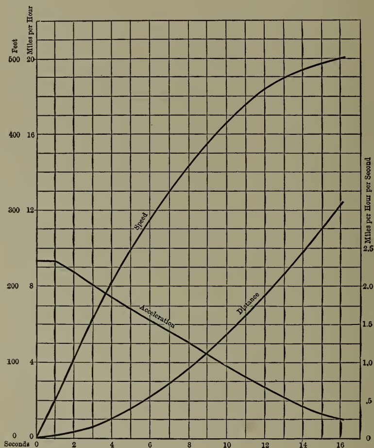
Fig. 60.—Speed and Distance Data, Test No. 14.
