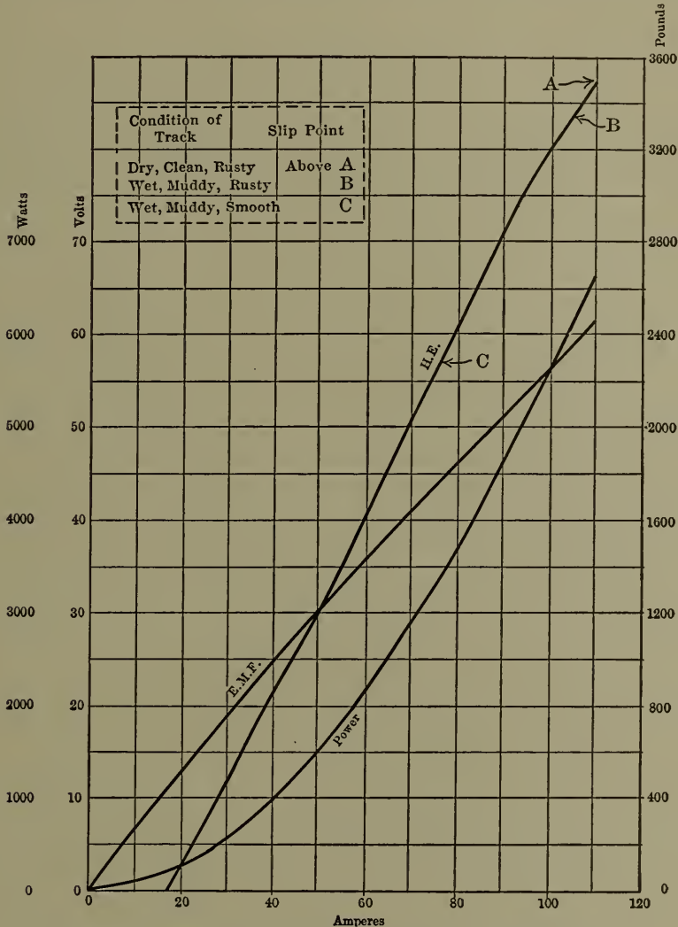
Fig. 108. — General Data, Industrial Locomotive Tests. Run No. 3.
