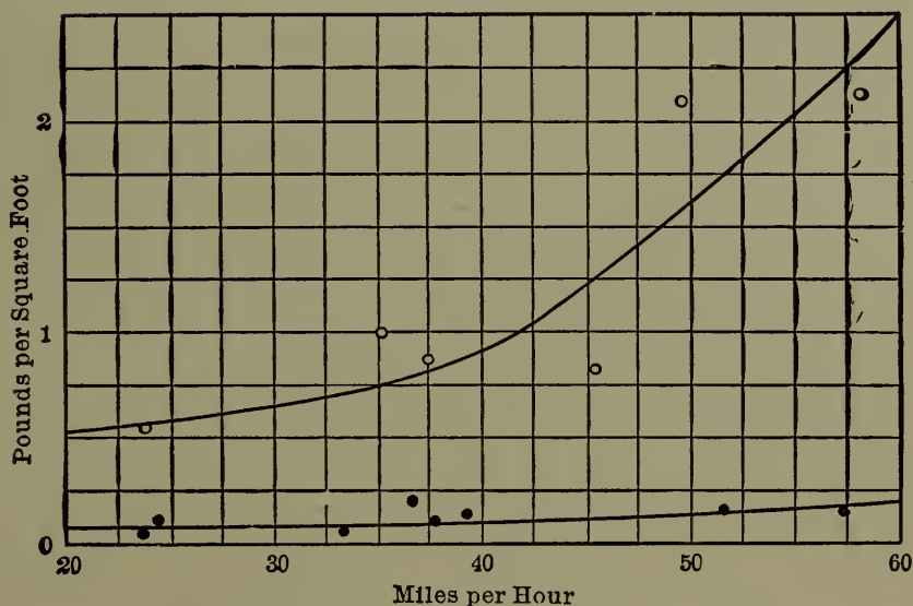
Fig. 200.—Air Resistance Curves for Parabolic Vestibule.
