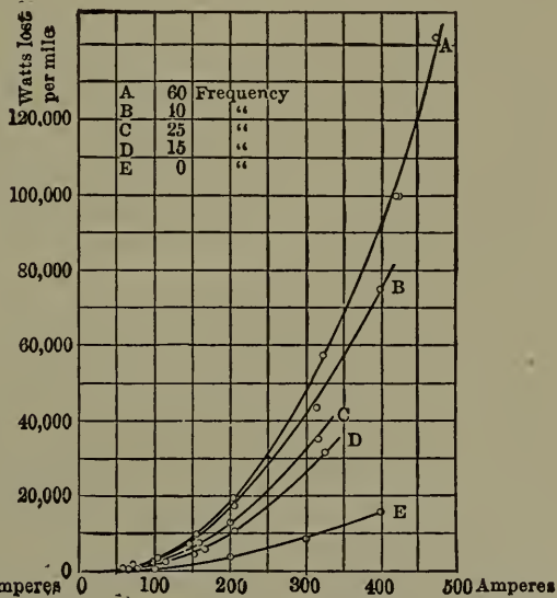
Fig. 159. — Variation of Pressure Lost per Mile with Total Current, Single Rail Alone.
