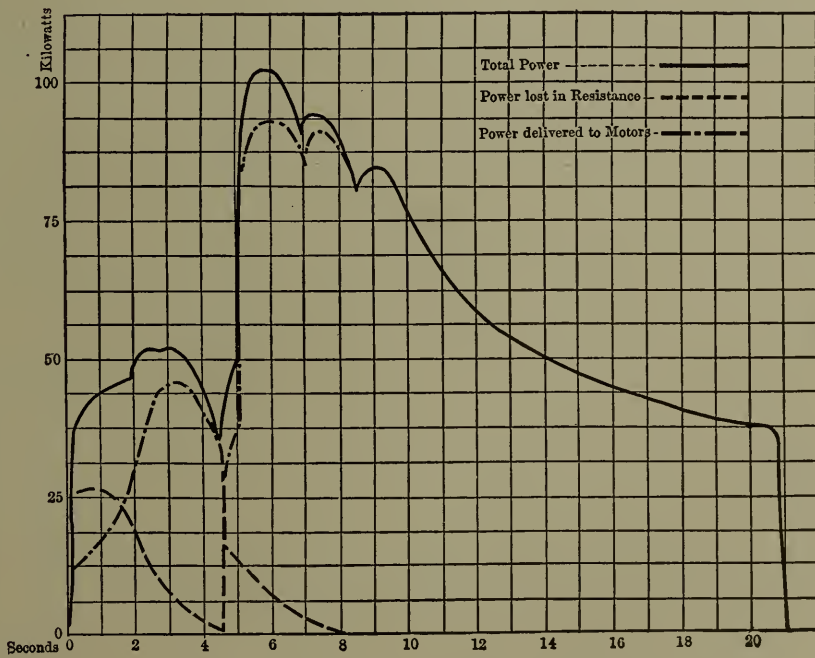
Fig. 35.—Division of Power in Test No. 3, Sept. 26, 1904.
