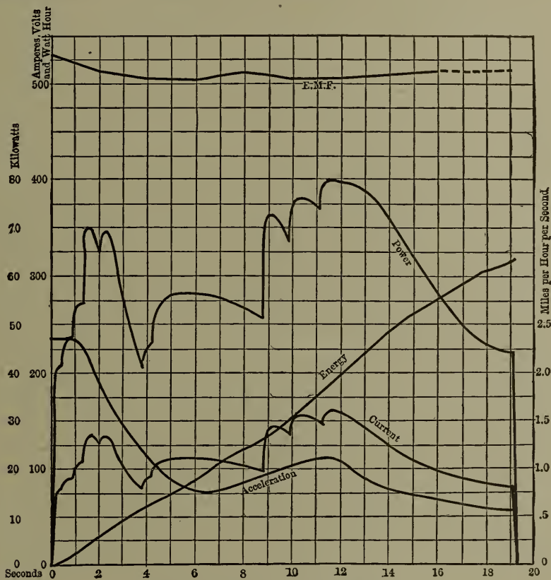
Fig. 63. — Electrical Data of Test No. 16.
