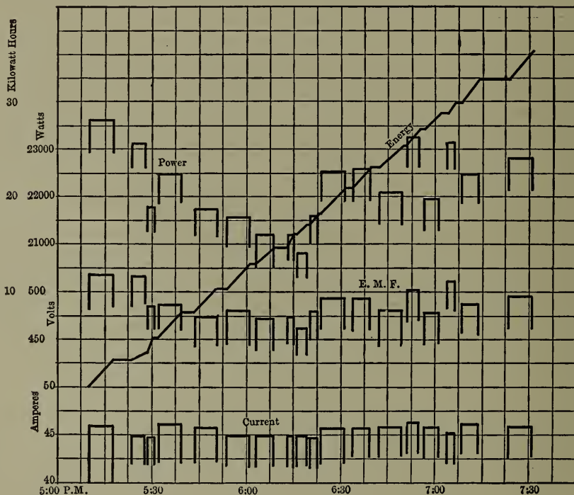
Fig. 82. — General Electrical Data of Test No. 21.
