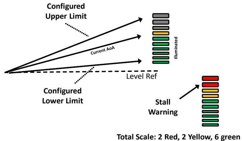
Figure 42 – AoA Upper and Lower Limits
