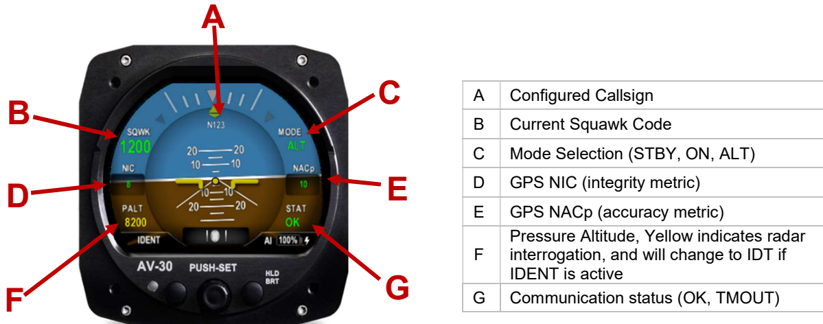
Figure 34 - Transponder Control
