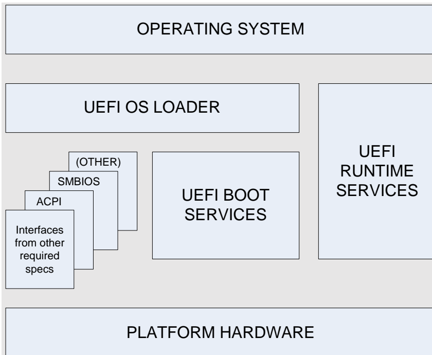
Figure 4 UEFI Architecture
