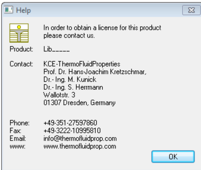
Figure 2.4 "Help" window
