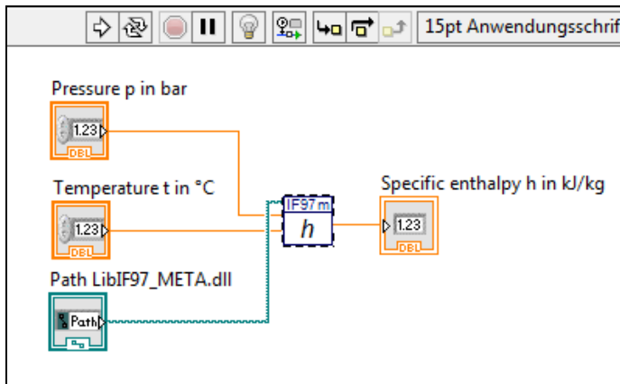
Figure 2.7 Block diagram of the example calculation
