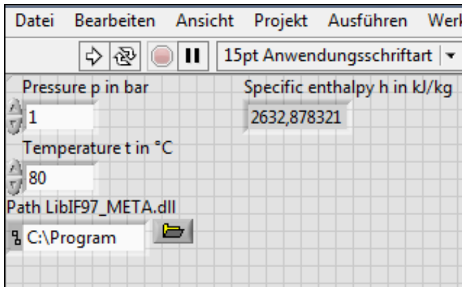
Figure 2.9 Result of the example calculation of h
