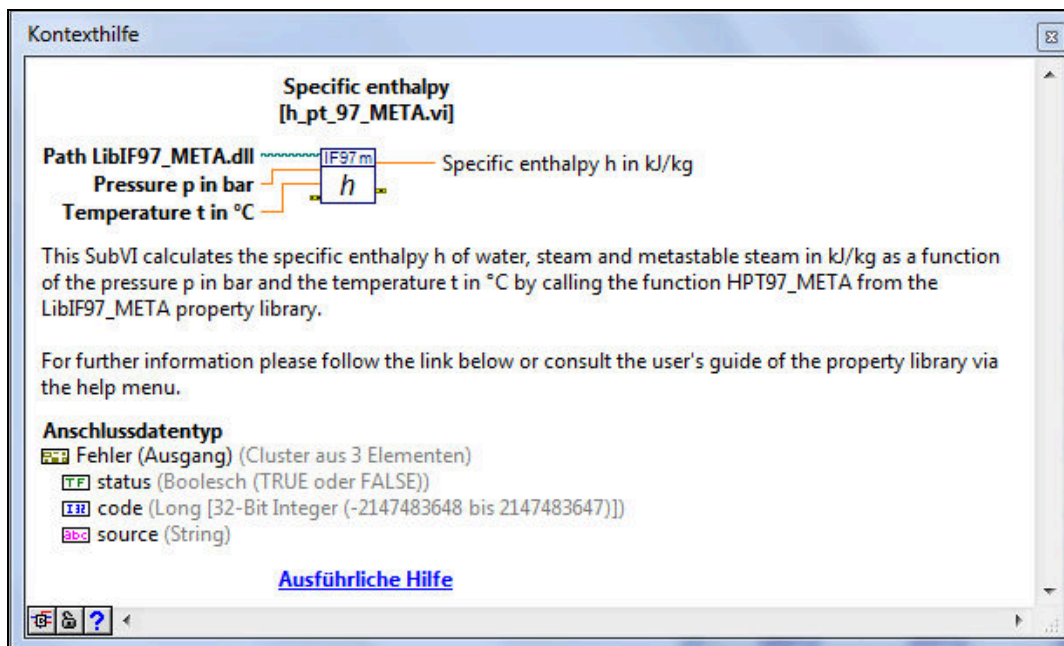
Figure 2.2 Context help window of the function h_pt_97_META.vi
