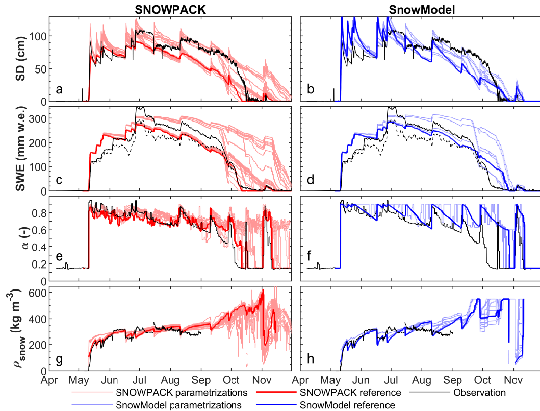
Figure 4. a-b) SD, c-d) SWE, e-f) albedo and g-h) snow density simulations (coloured) of the ensemble approaches for SNOWPACK (red) and SnowModel (blue) and observations (black). The bold coloured lines show the reference simulations chosen as the most optimal parameterization set according to the measured albedo. The solid (dotted) line in c-d) indicates the more (less) reliable SWE measurement from potassium (thallium) rays.
