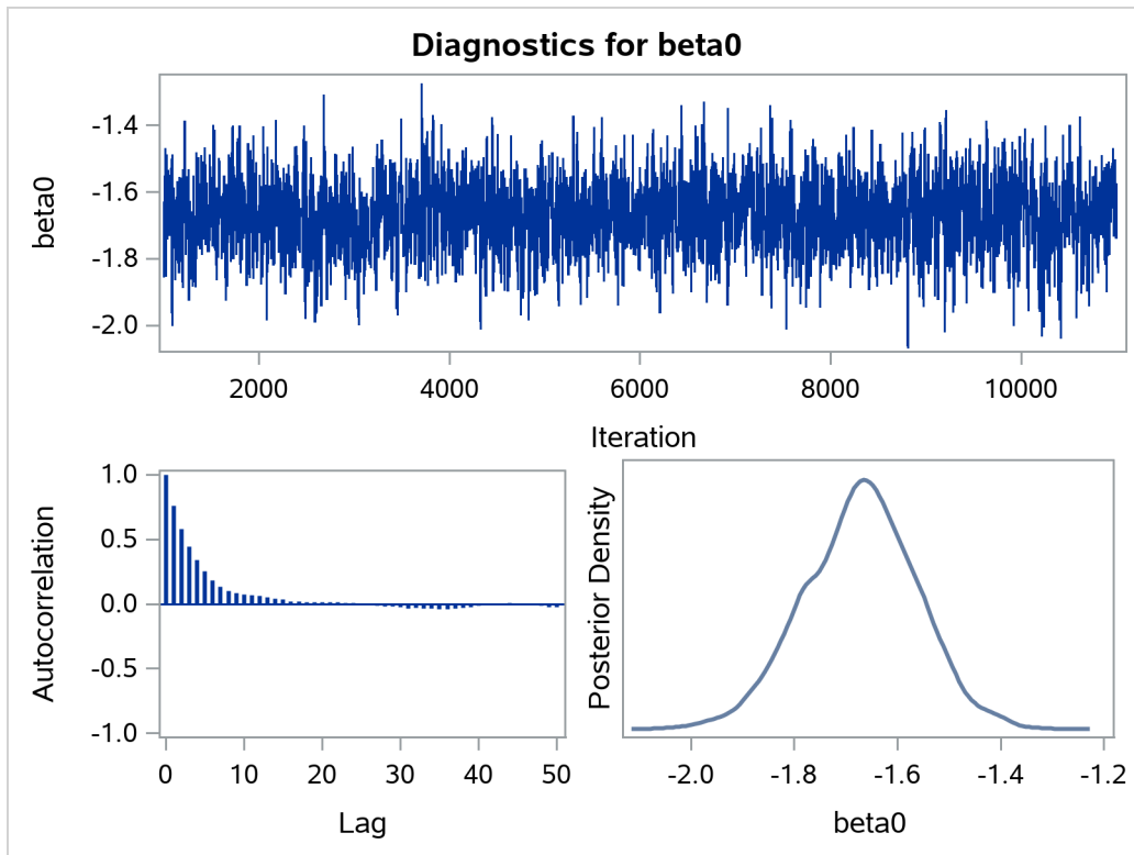
Output 77.13.1 Posterior Plots for \beta_0 and \beta_1 in the Exponential Survival Analysis
