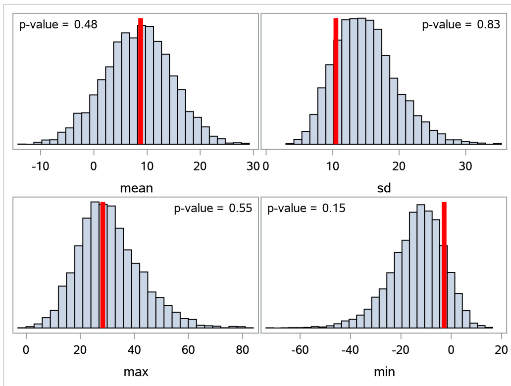
Figure 77.27 Posterior Predictive Distribution Check for the SAT example
