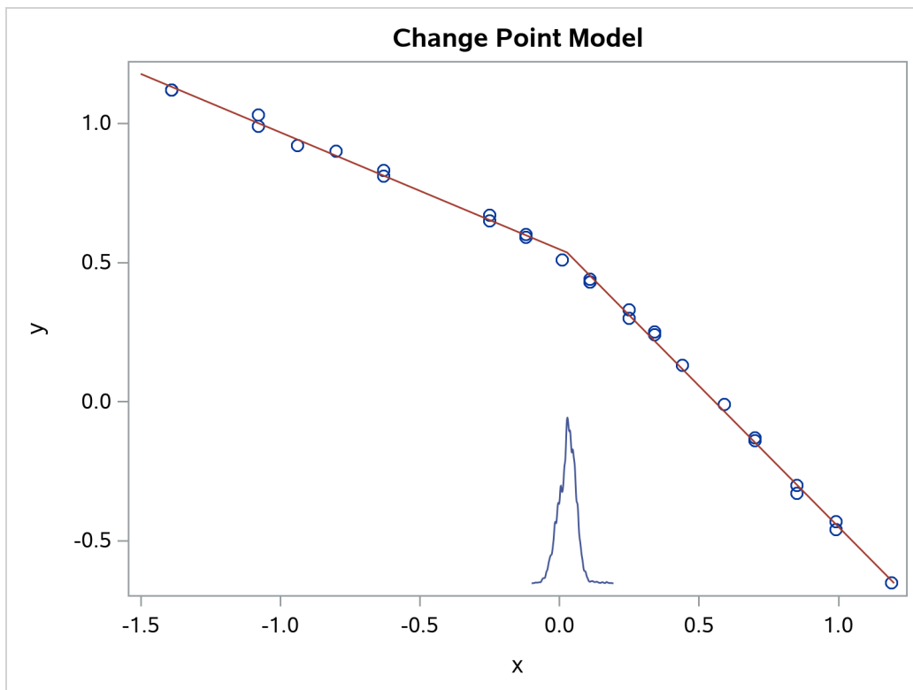
Output 77.12.3 Estimated Fit to the Stagnant Data Set
