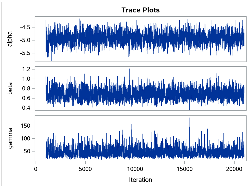
Output 77.6.4 Plots for Parameters, Sampling on the Log Scale of Gamma
