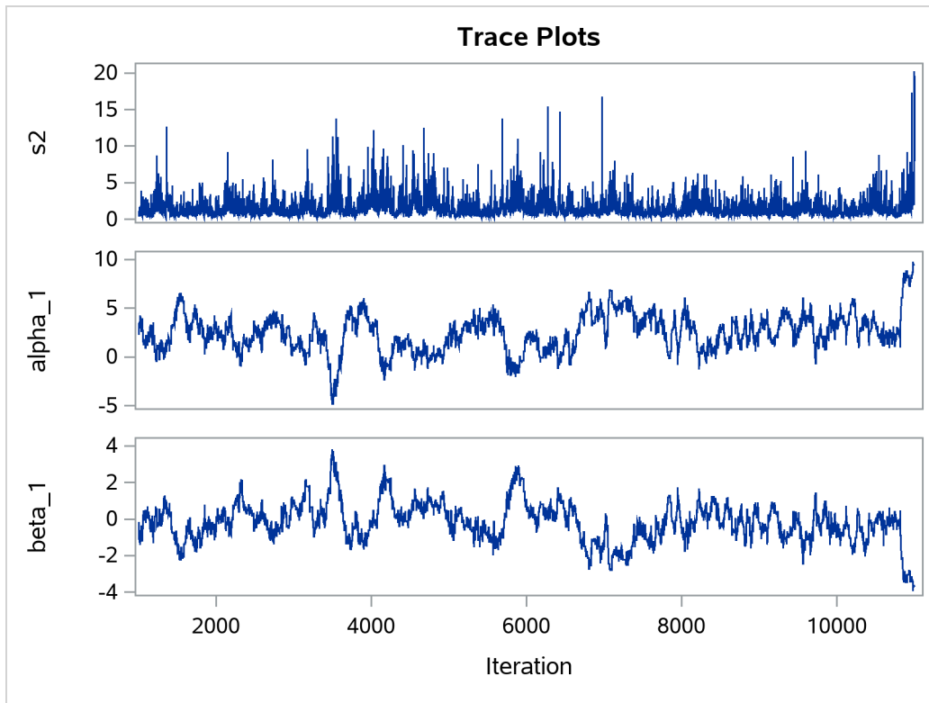
Output 77.8.1 Trace Plots of \sigma^2 , \alpha , \beta , and e_8 without Hierarchical Centering
