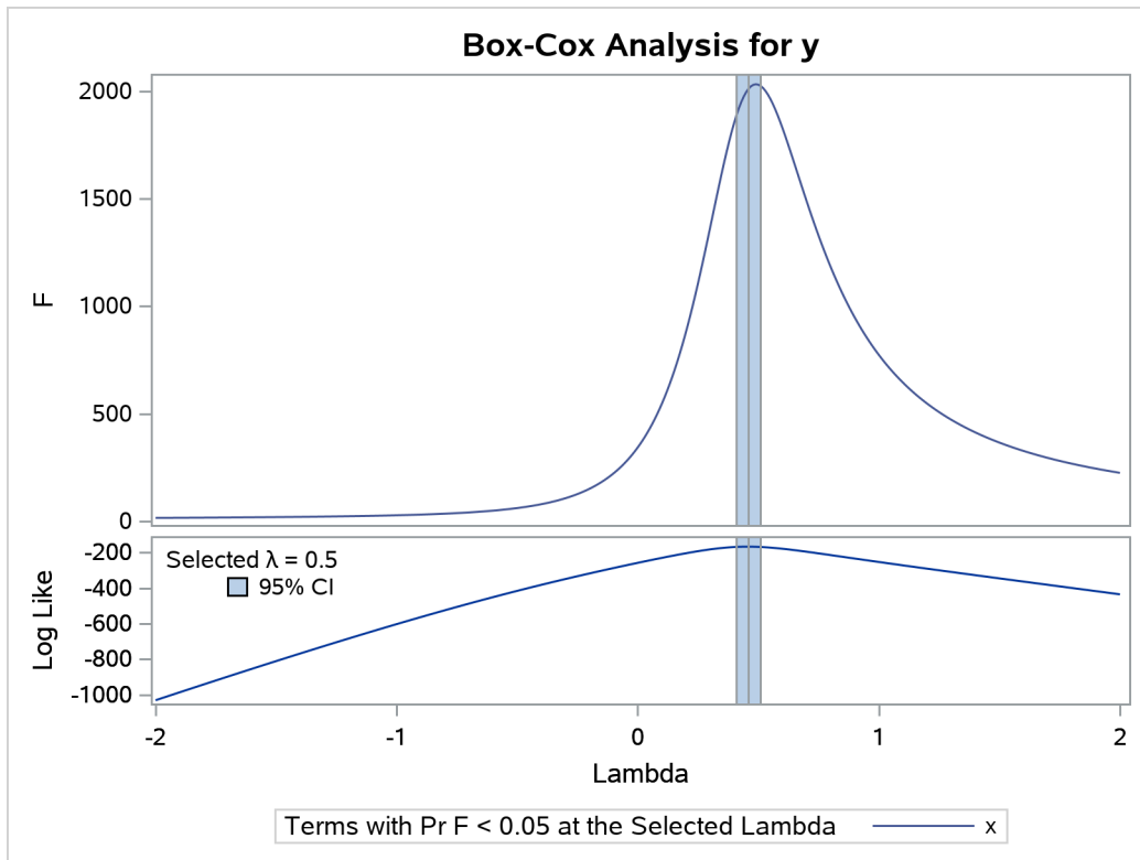
Output 77.2.3 Box-Cox Transformation Using PROC TRANSREG
