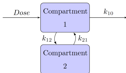
Figure 77.18 Two-Compartment Model
