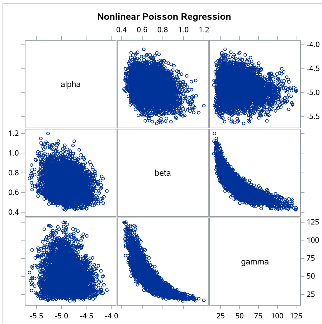
Output 77.6.3 Pairwise Scatter Plots of the Parameters
