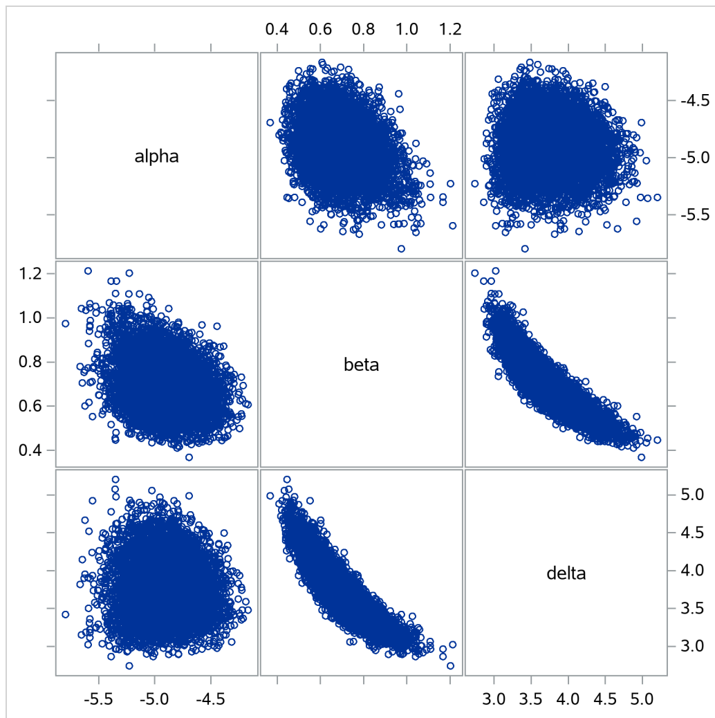
Output 77.6.7 Pairwise Scatter Plots of the Transformed Parameters
