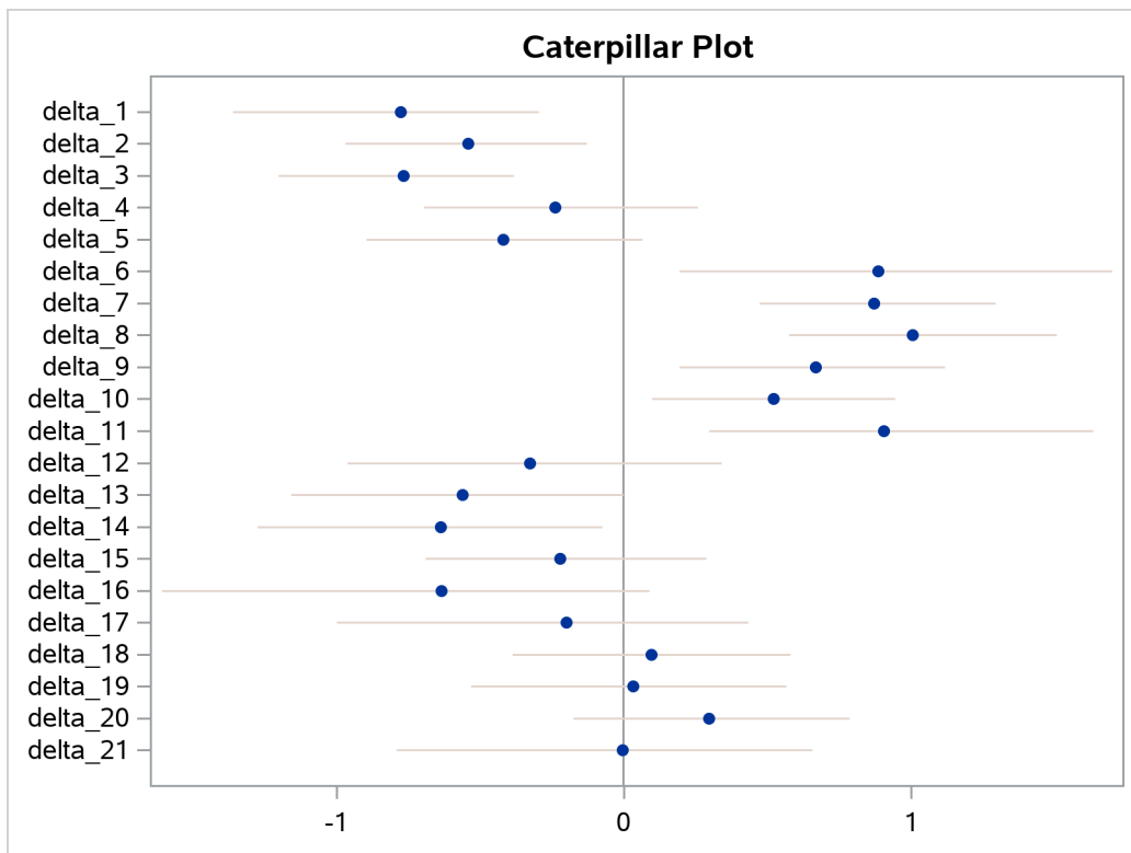
Figure 77.24 Caterpillar Plot of the Random-Effects Parameters
