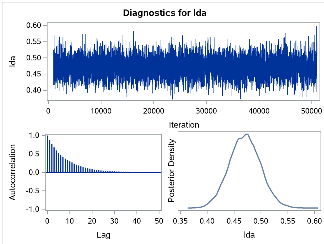
Output 77.2.2 Diagnostic Plots for \lambda
