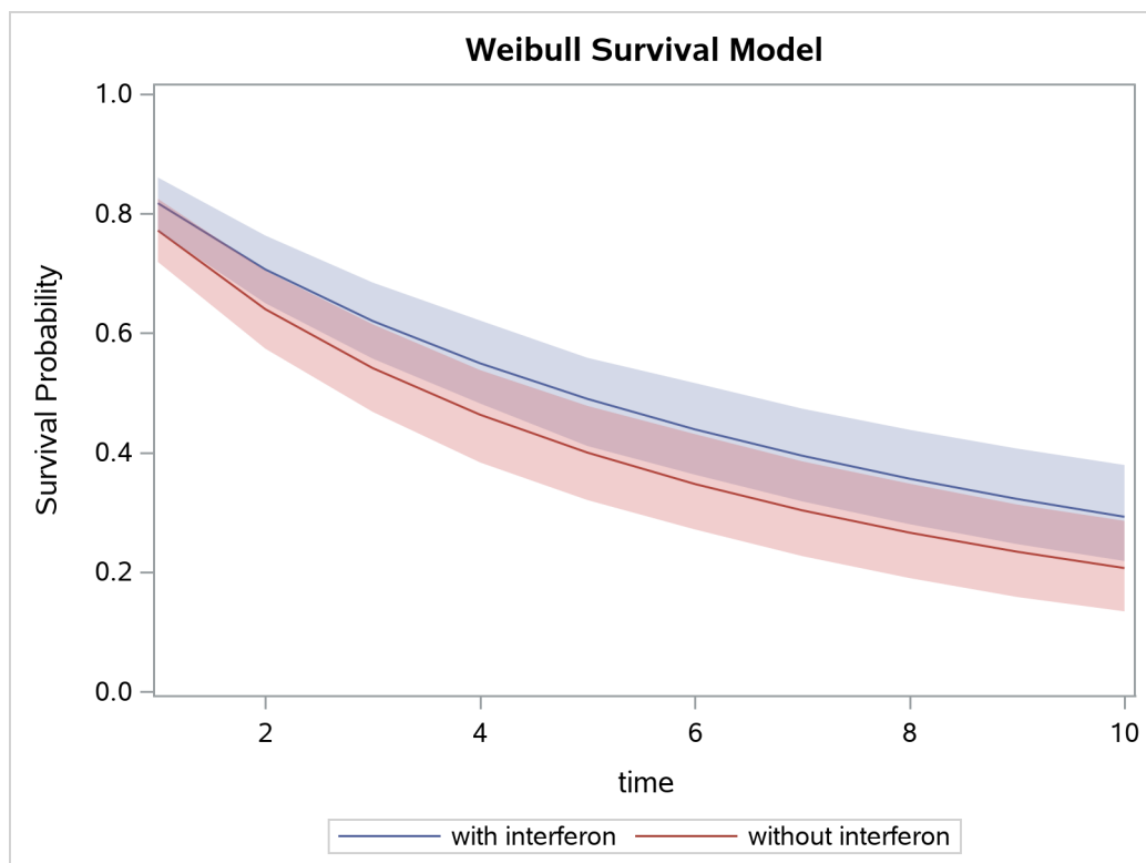
Output 77.13.7 Predicted Survival Probability Curves with 95% HPD Intervals
