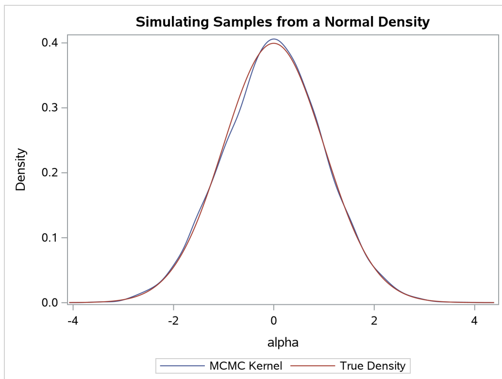
Output 77.1.4 Estimated Density versus the True Density
