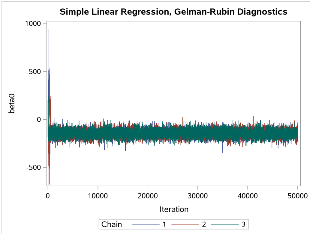
Output 77.21.2 Trace Plots of Three Chains for Each of the Parameters
