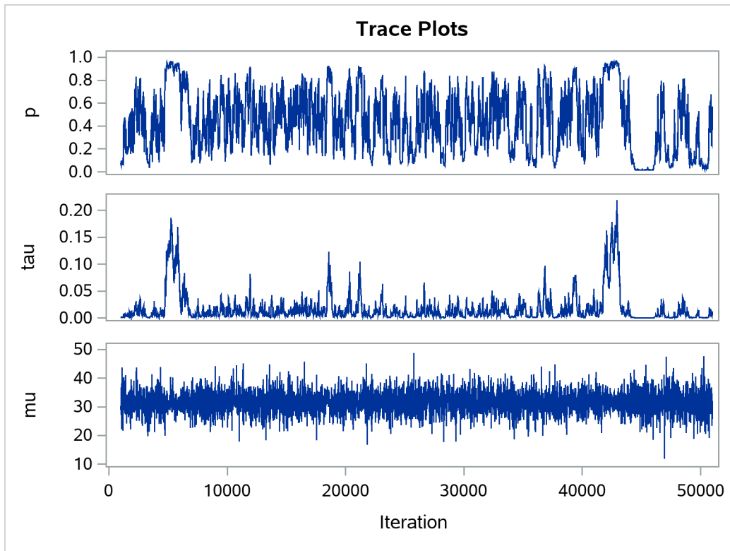
Output 77.20.1 Trace Plots
