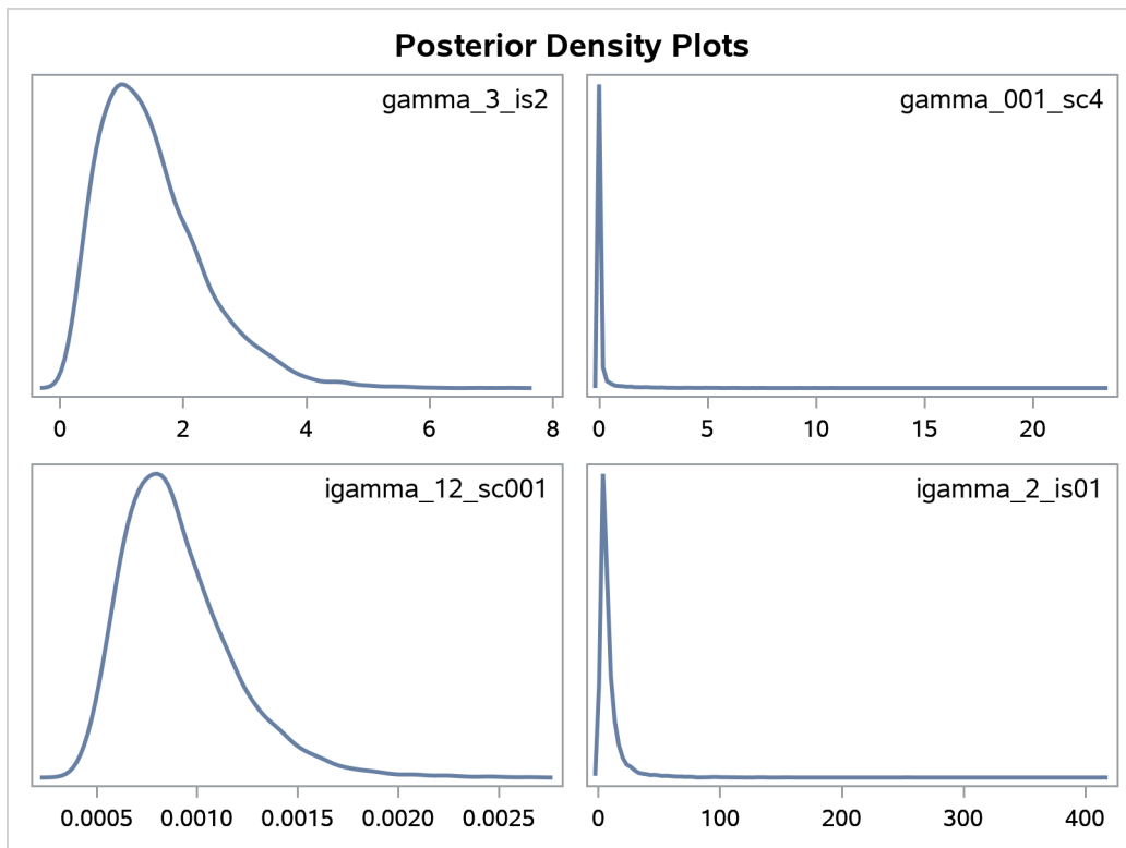
Figure 77.26 Density Plots of Different Gamma and Inverse Gamma Distributions
