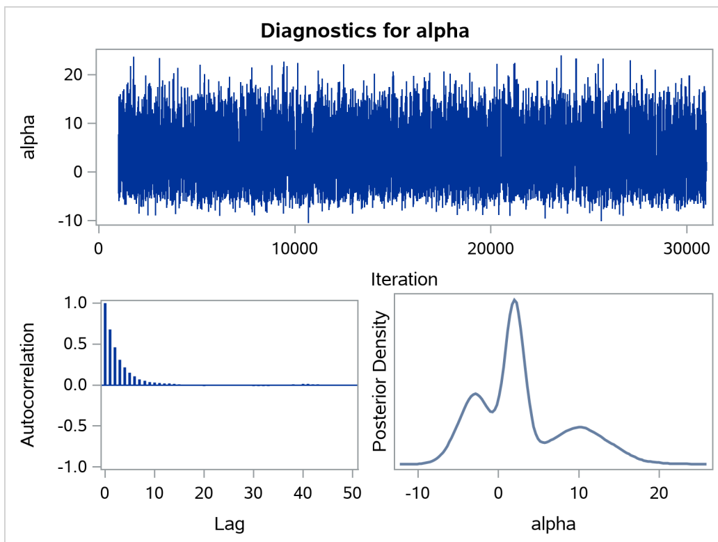
Output 77.1.8 Plots of Posterior Samples from a Mixture Normal Distribution
