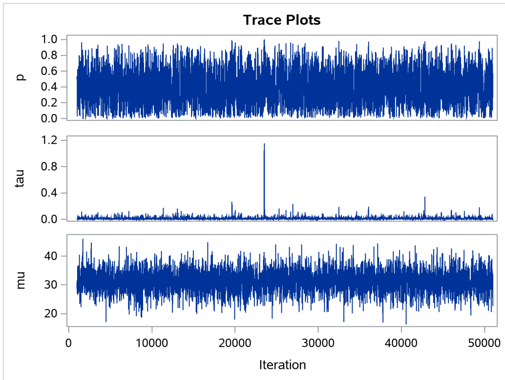
Output 77.20.4 Trace Plots after Transformation
