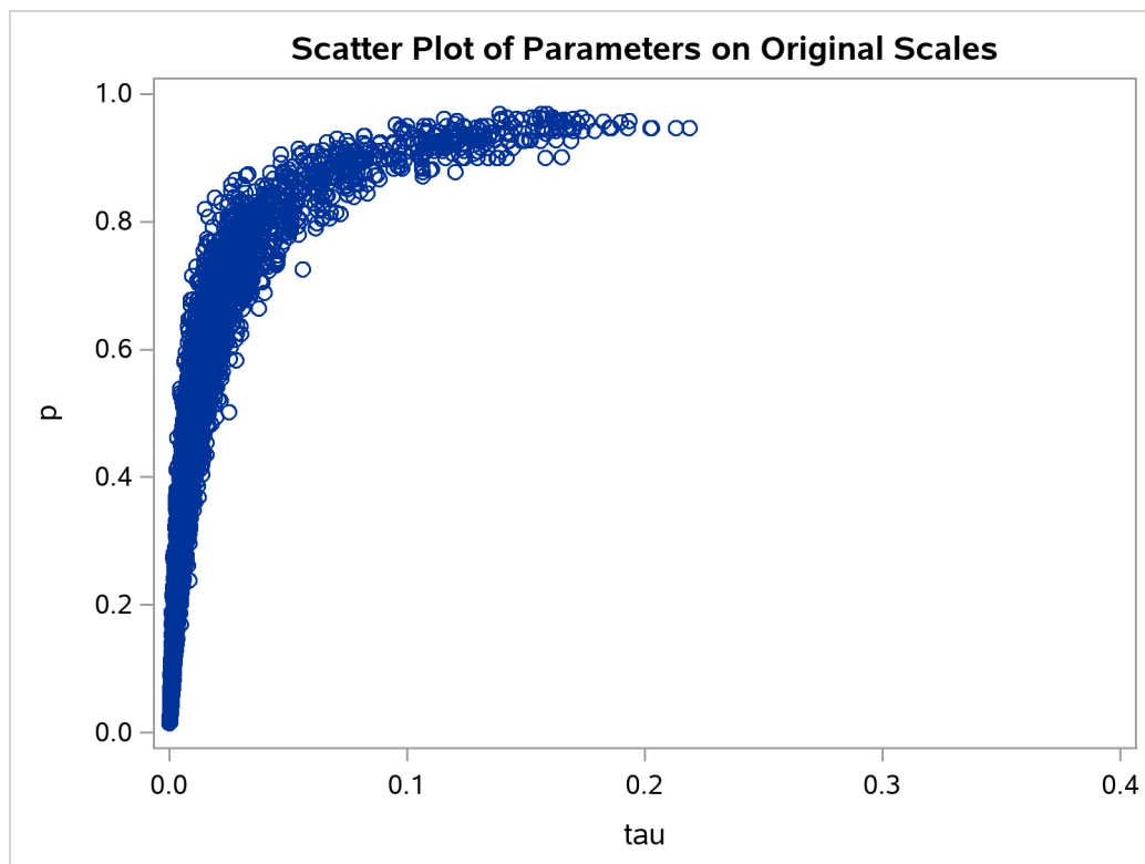
Output 77.20.3 Scatter Plot of \tau versus p
