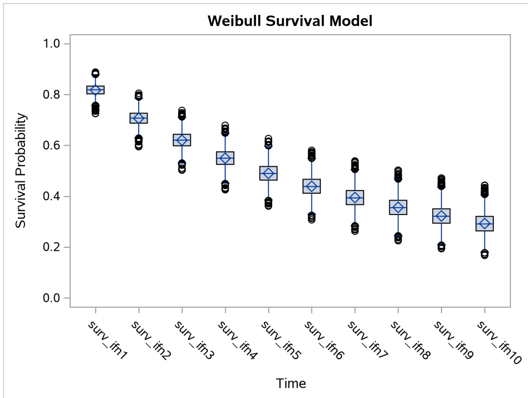
Output 77.13.6 Side-by-Side Box Plots of Estimated Survival Probabilities
