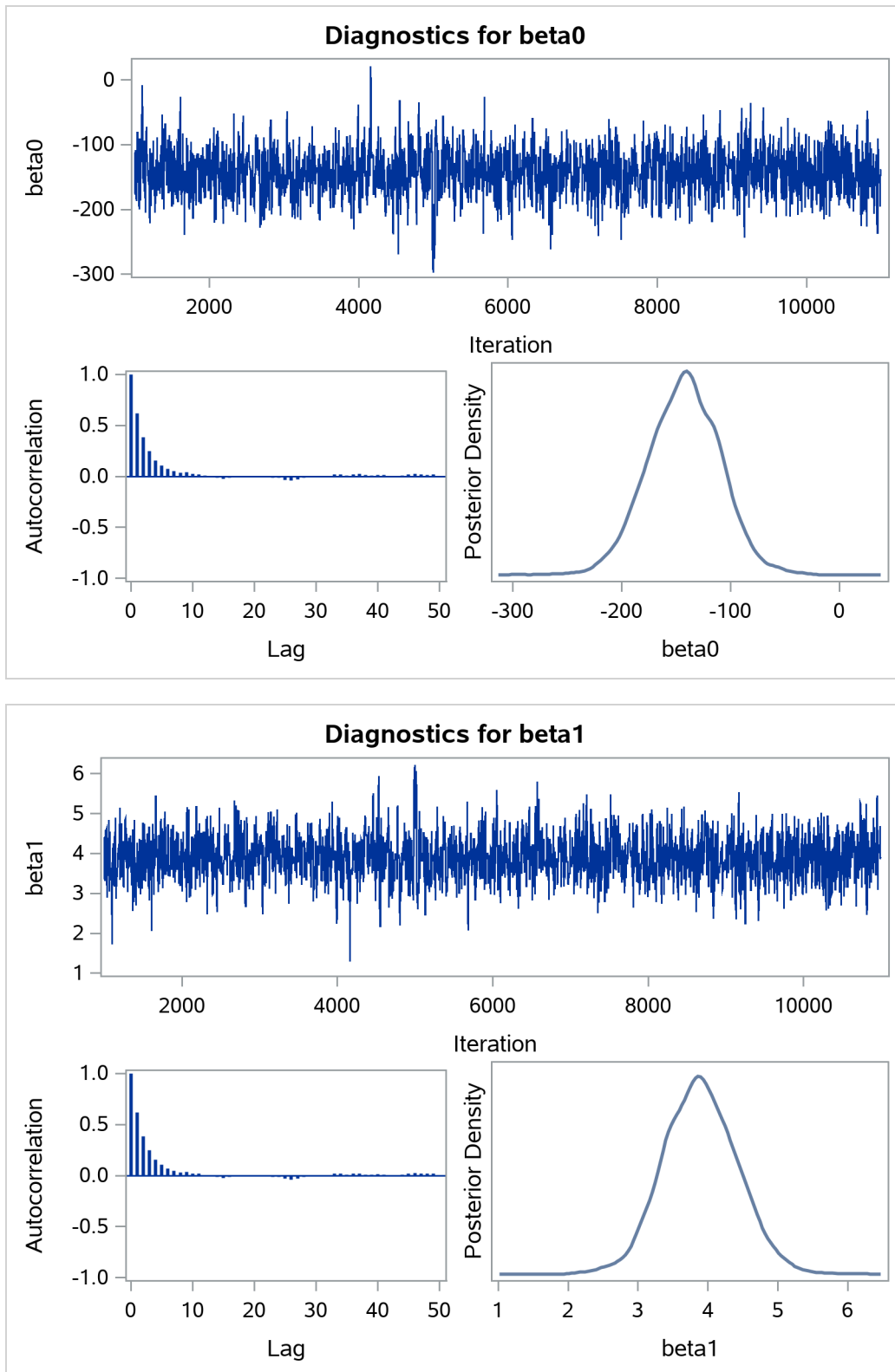
Figure 77.5 Diagnostic Plots for \beta_0 , \beta_1 and \sigma^2
