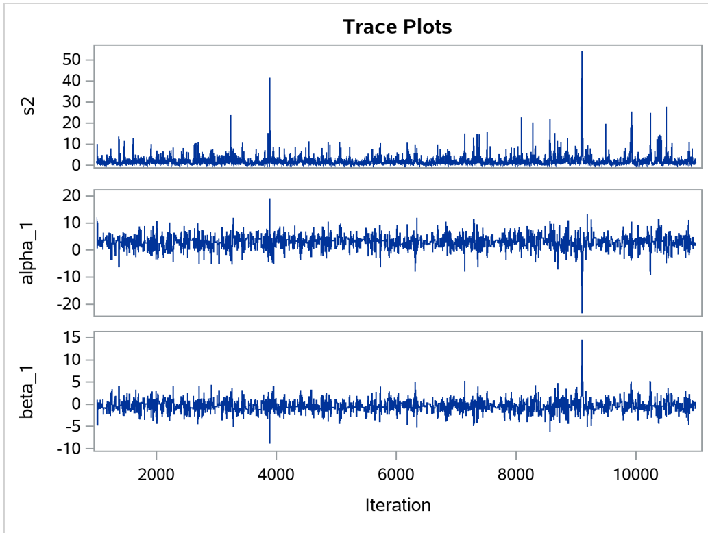
Output 77.8.2 Trace Plots of \sigma^2 , \alpha , and \beta with Hierarchical Centering
