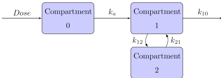
Figure 77.21 Two-Compartment Model with Absorption Phase
