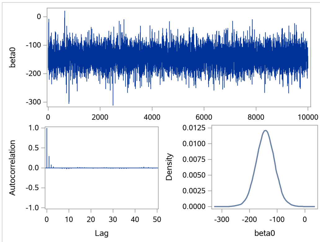
Figure 77.23 Regenerated Diagnostics Plots for beta0 and Logpost
