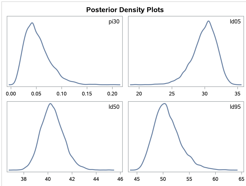
Output 77.3.5 Density Plots of Quantities of Interest in the Logistic Regression Example
