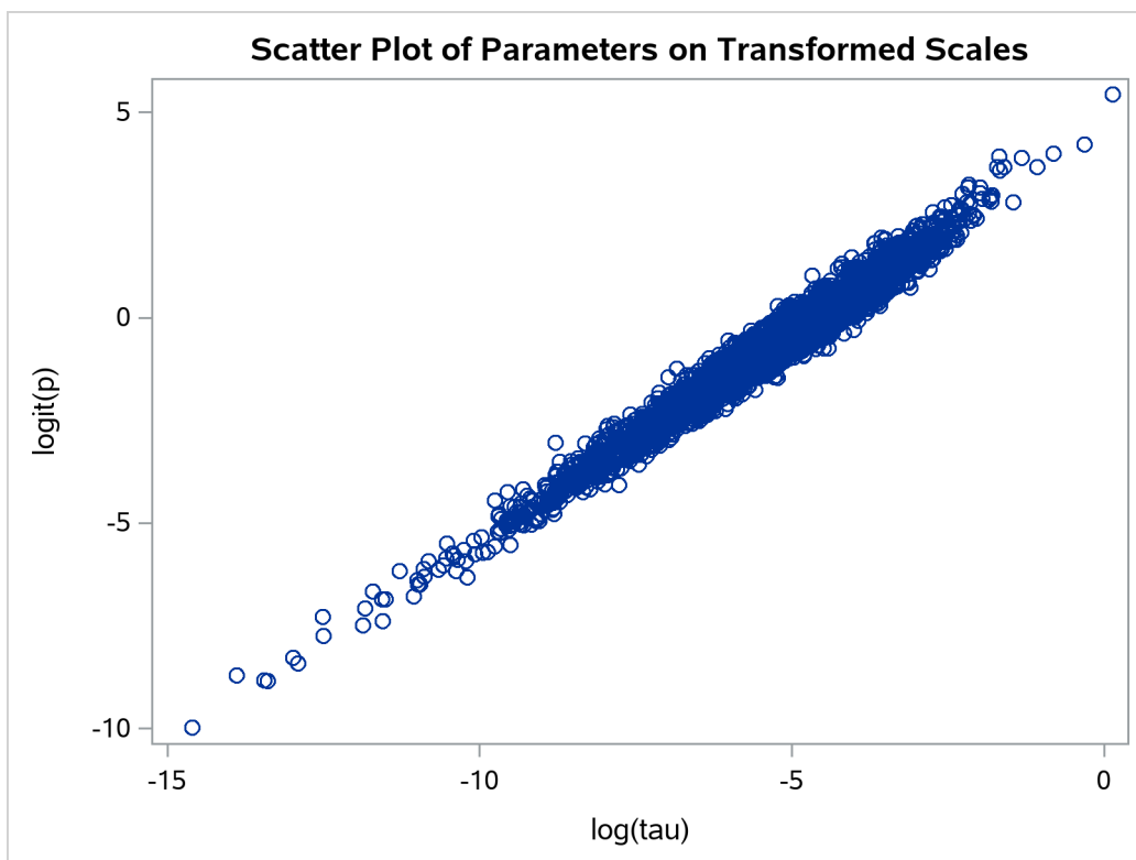
Output 77.20.6 Scatter Plot of \log(\tau) versus \text{logit}(p) , After Transformation
