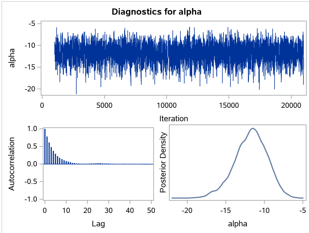
Output 77.3.2 Plots for Parameters in the Logistic Regression Example
