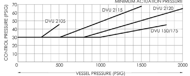
VALVE OPERATING PRESSURE MINIMUM ACTUATION PRESSURE
