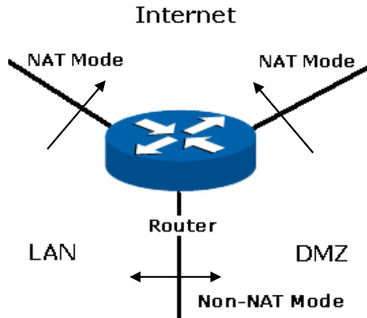
Figure 3-17 DMZ – Private Mode
