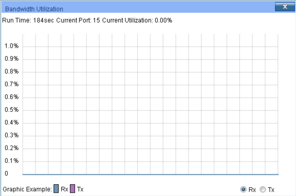
Figure 4-3 Bandwidth Utilization
