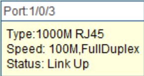
Figure 4-2 Port Information
