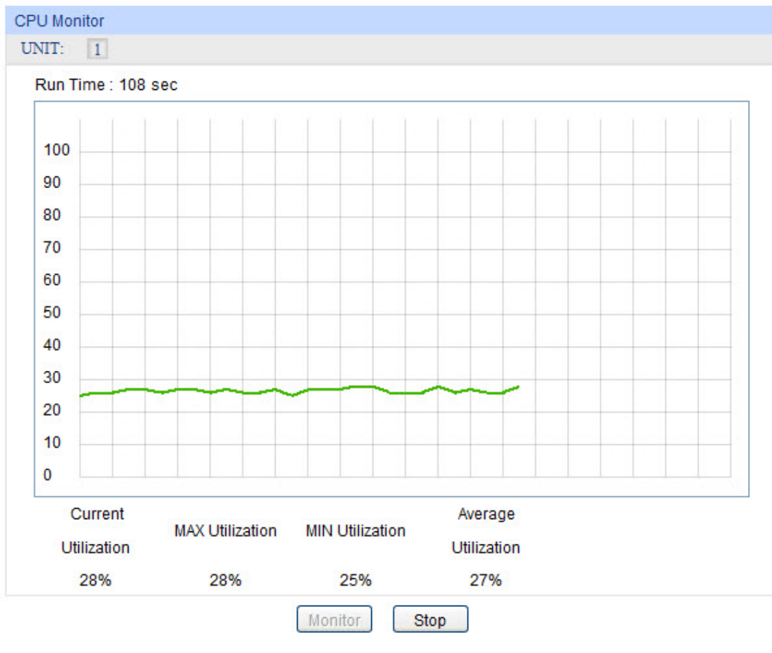
Figure 16-1 CPU Monitor
