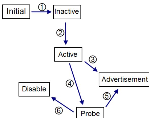
Figure 8-11 DLDP Process
