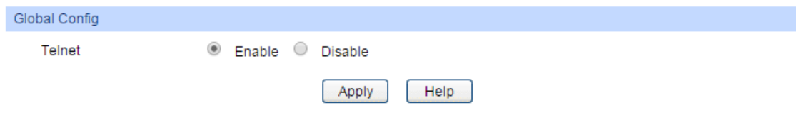
Figure 4-21 Access Control
