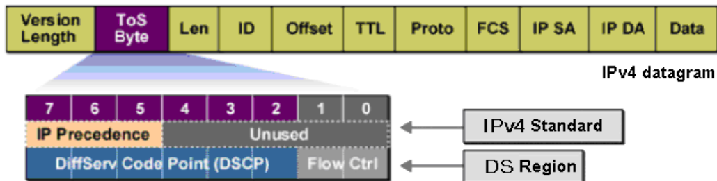
Figure 11-3 IP datagram
