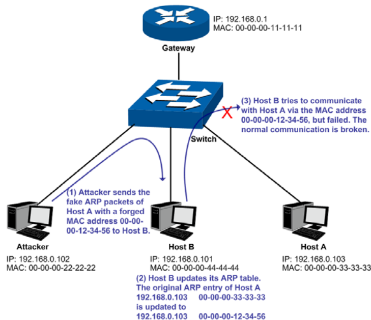
Figure 13-17 ARP Attack – Cheating Terminal Hosts
