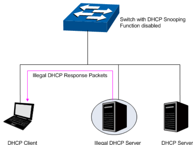
Figure 13-10 DHCP Cheating Attack Implementation Procedure
