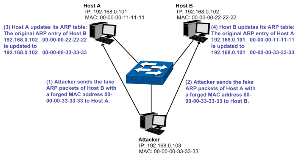
Figure 13-18 Man-In-The-Middle Attack
