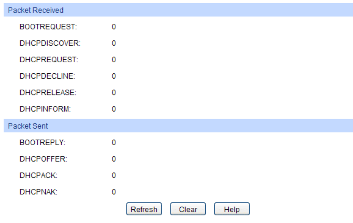
Figure10-20 Statistics
