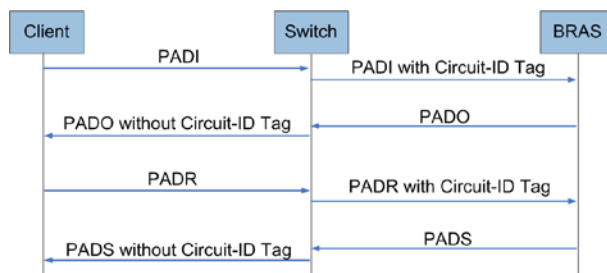
Figure 13-1 PPPoE Discovery Process
