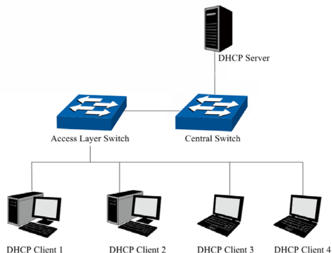
Figure 13-8 Network diagram for DHCP-snooping implementation
