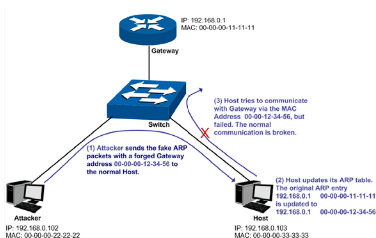
Figure 13-15 ARP Attack - Imitating Gateway
