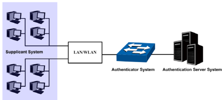
Figure 13-25 Architecture of 802.1X authentication
