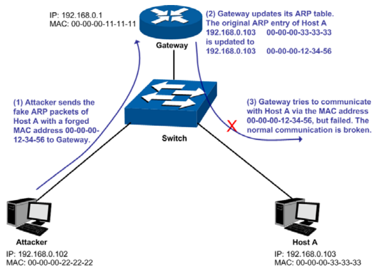
Figure 13-16 ARP Attack – Cheating Gateway
