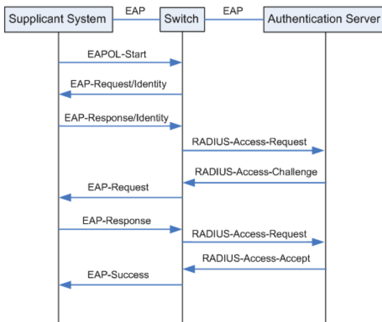
Figure 13-26 EAP-MD5 Authentication Procedure
