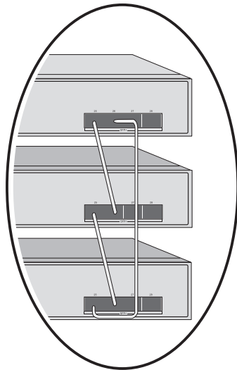
Figure 3-4 Ring Connection
