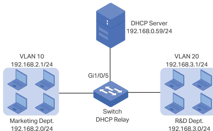
Figure 5-1 Network Topology for DHCP Relay
