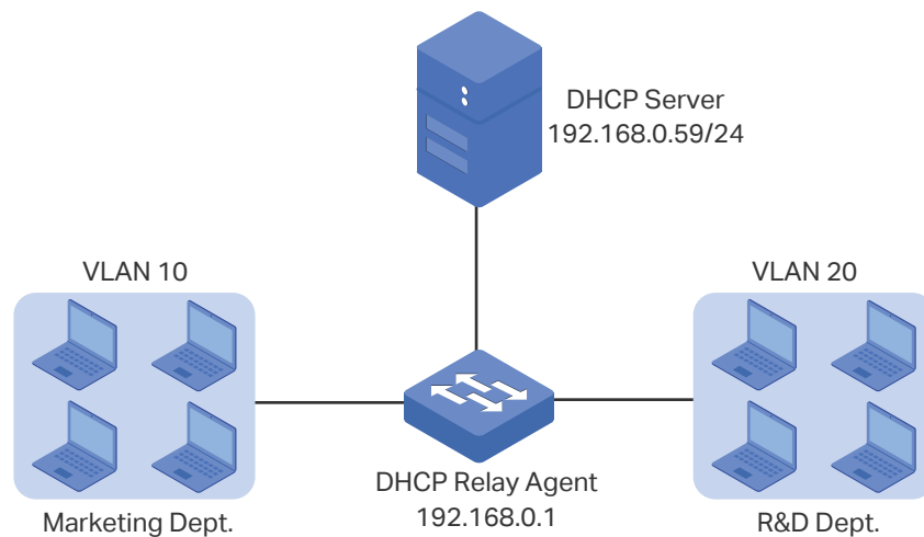
Figure 5-4 Network Topology for DHCP VLAN Relay
