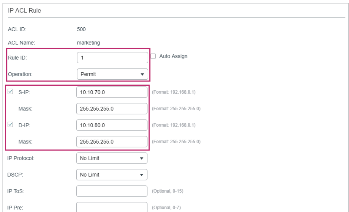
Figure 3-16 Configuring Rule 1
