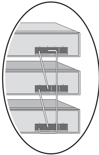
Figure 3-6 Ring Connection
