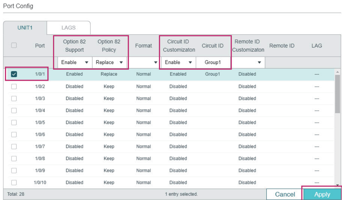
Figure 5-3 Configuring Port 1/0/1
