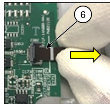
(6) Cable
