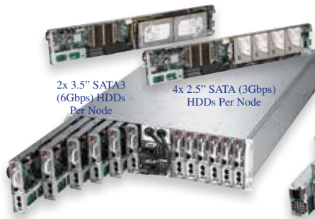
2x 3.5" SATA3 (6Gbps) / SAS HDDs w/ selected HBA or RAID card Per Node
