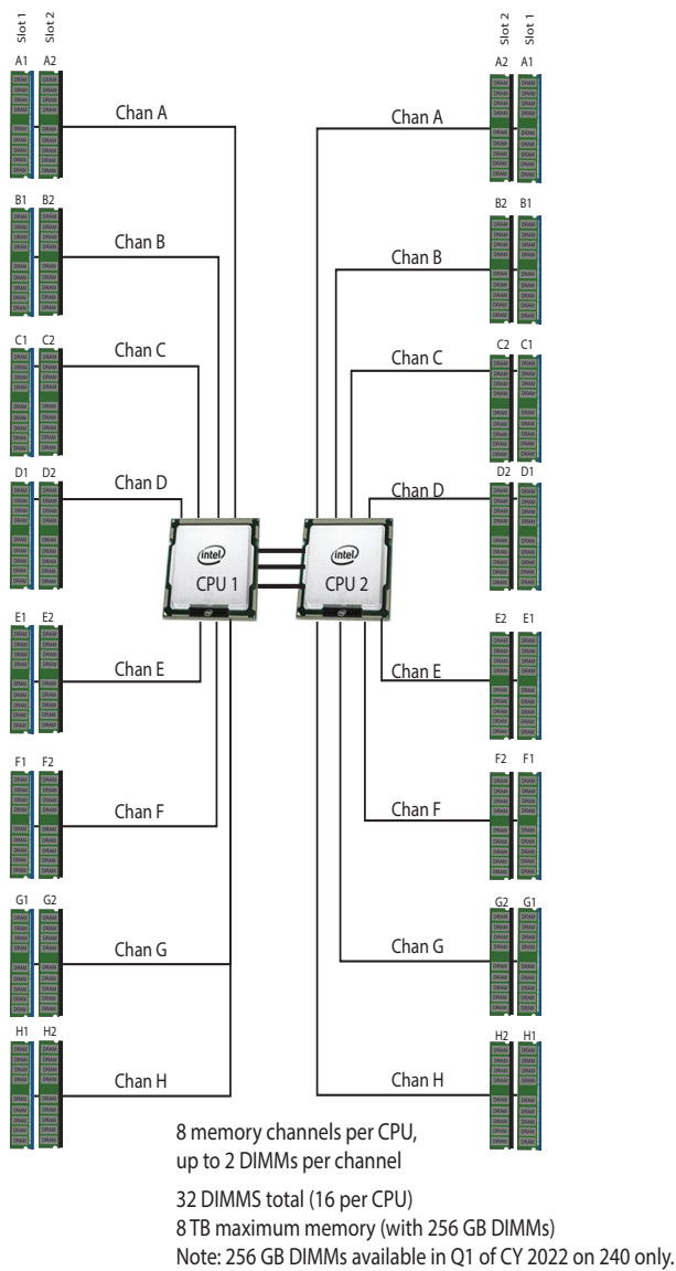
Figure 11 C240 M6 SFF Memory Organization
