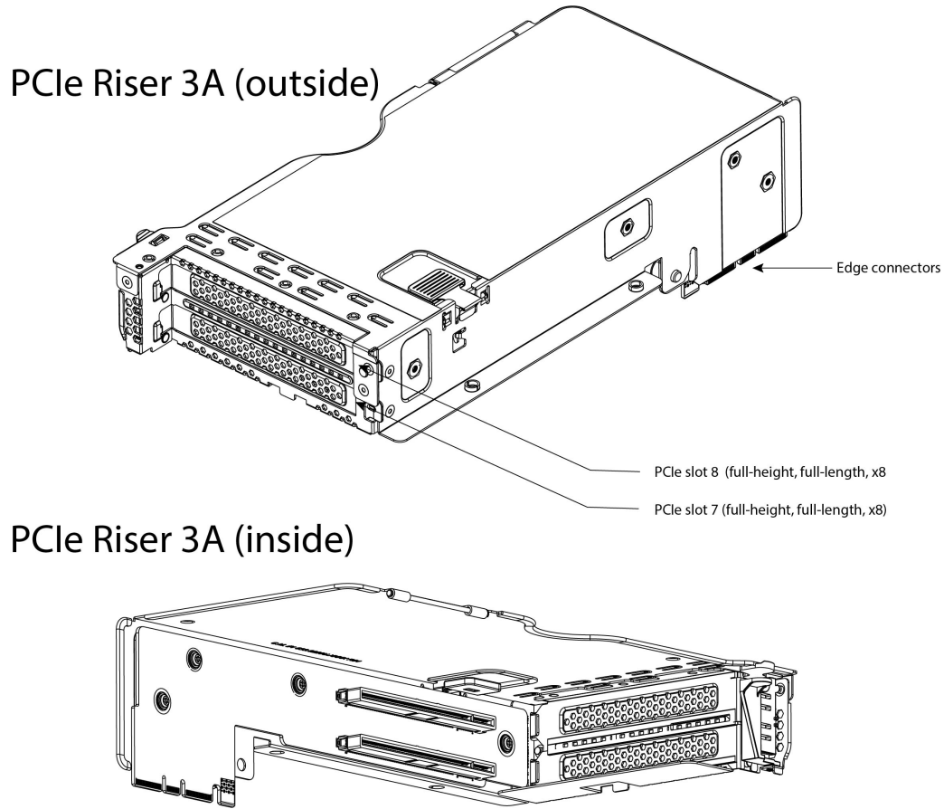
Figure 24 Riser Card 3A
