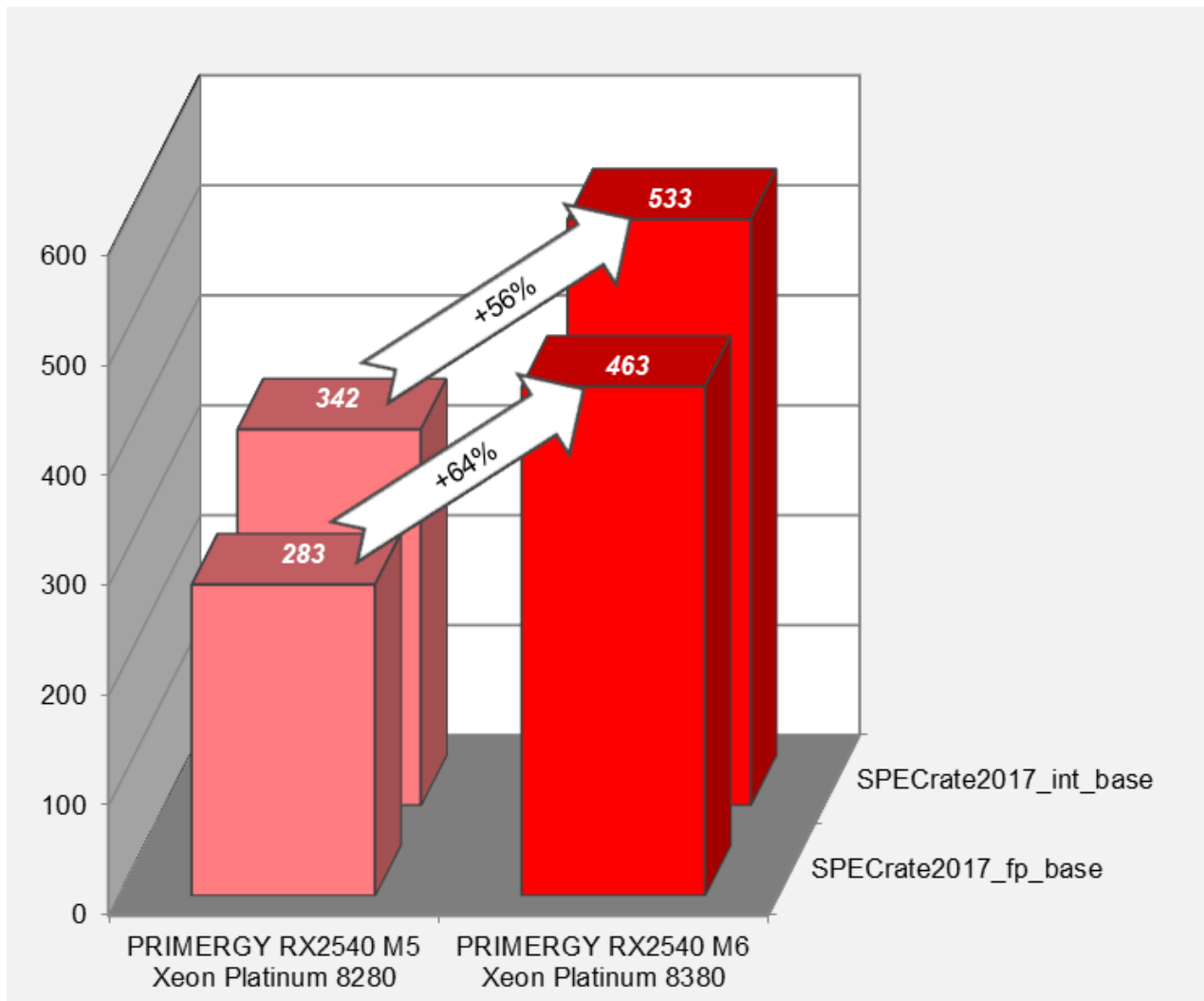
SPECrate2017: Comparison of PRIMERGY RX2540 M6 and PRIMERGY RX2540 M5
