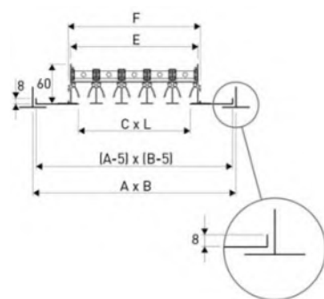
SHF-P VERSION STANDARD
