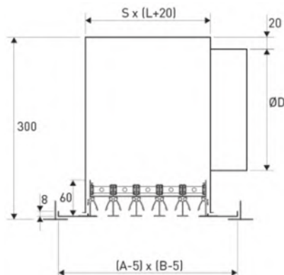
SHF-P + PLENUM VERSION STANDARD
