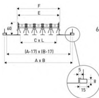
SHF-P VERSION FINE LINE
