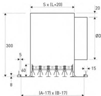
SHF-P + PLENUM VERSION FINE-LINE
