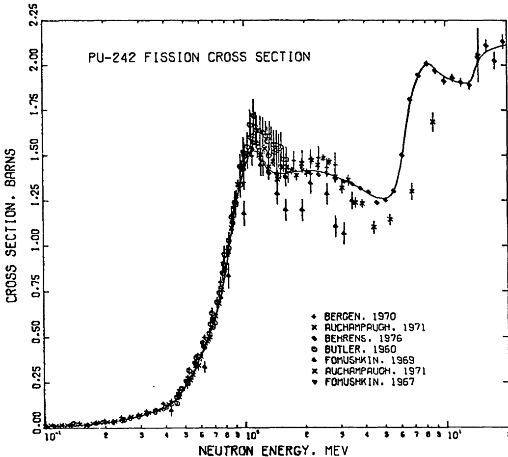
Fig. 7. Experimental and evaluated ^{242}\text{Pu}(n,f) cross sections between 0.1 and 20 MeV. The solid curve is the LASL-78 evaluation.
