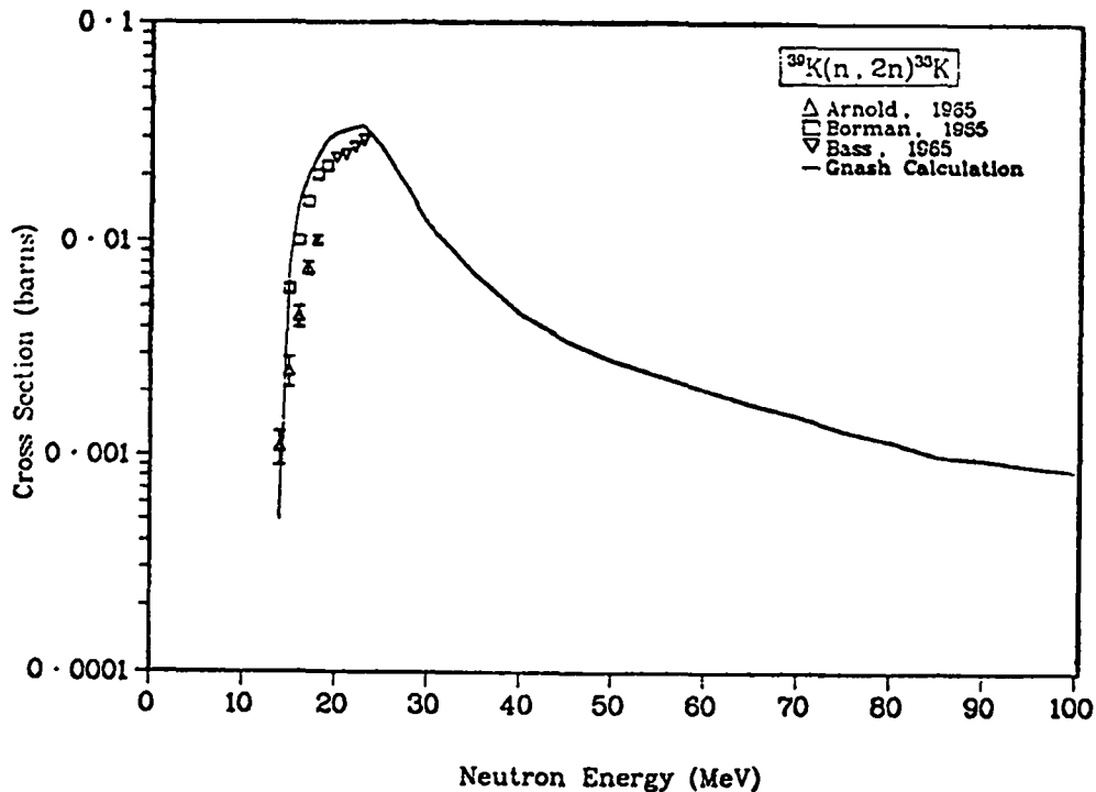
Fig. 3. Calculation of the ^{39}\text{K}(n,2n) cross section from threshold to 100 MeV made using GNASH is shown.
