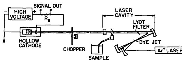
Fig. 5a. OGE detector of intracavity absorption.
