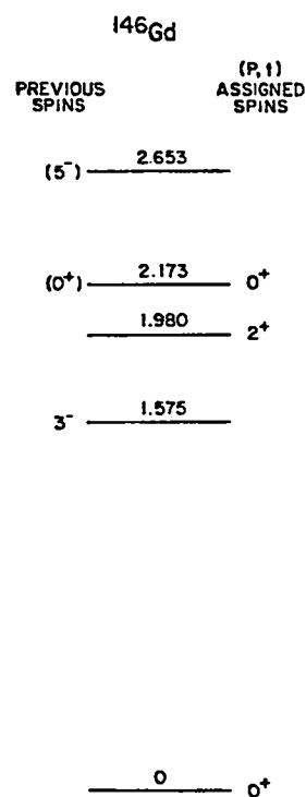
Fig. 57. Low-lying levels in ^{146}\text{Gd} .
