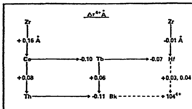
Fig. 29. Trends in size differences of tetravalent elements.
