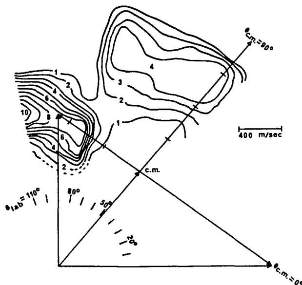
Fig. 34. Center-of-mass recoil angle and velocity flux contour map of the NO 2 product from the NO + O 3 reaction at a relative translational energy of 14.2 kcal/mole. Contour map is superimposed on the "Newton diagram" showing the most probable NO ( \theta_{\text{lab}} = 0^\circ ) and O 3 ( \theta_{\text{lab}} = 90^\circ ) velocity vectors.
