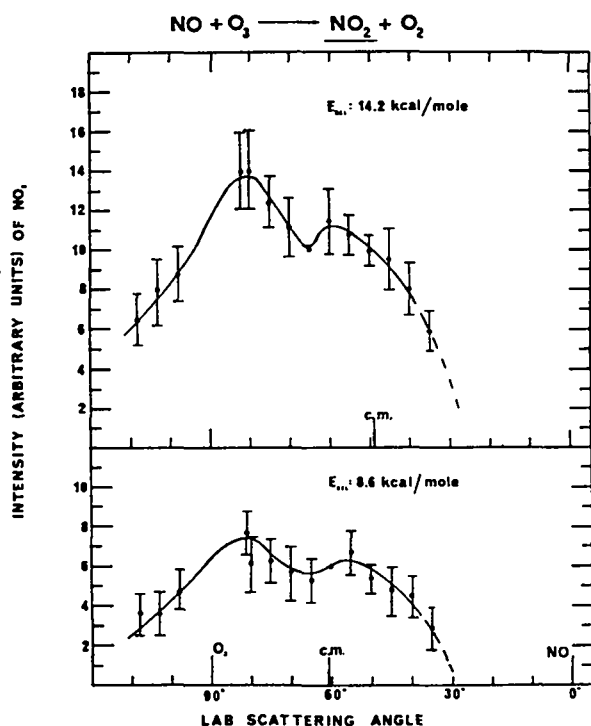
Fig. 33. Angular distribution of the NO 2 product from the NO + O 3 reaction at relative translational energies of 8.6 and 14.2 kcal/mole. O 3 beam at 90°, NO beam at 0°.
