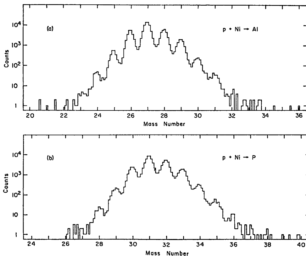
Fig. 59. Mass spectra observed in 800-MeV proton bombardment of nat Ni for the elements (a) aluminum and (b) phosphorus.
