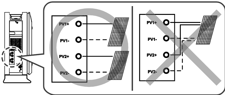
[Figure 2-3: PV connections]
