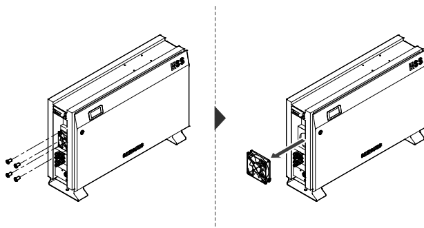
[Figure 6-2: Fan removal]
