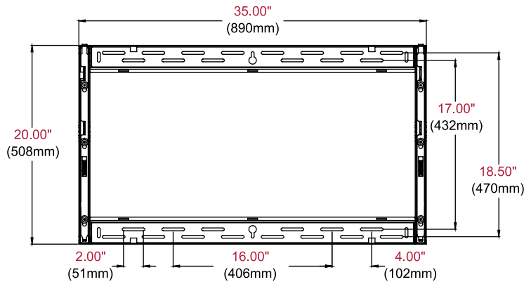
WALL PLATE DETAIL
