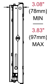
SIDE VIEW COLLAPSED
