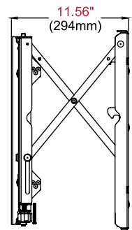
SIDE VIEW EXTENDED
