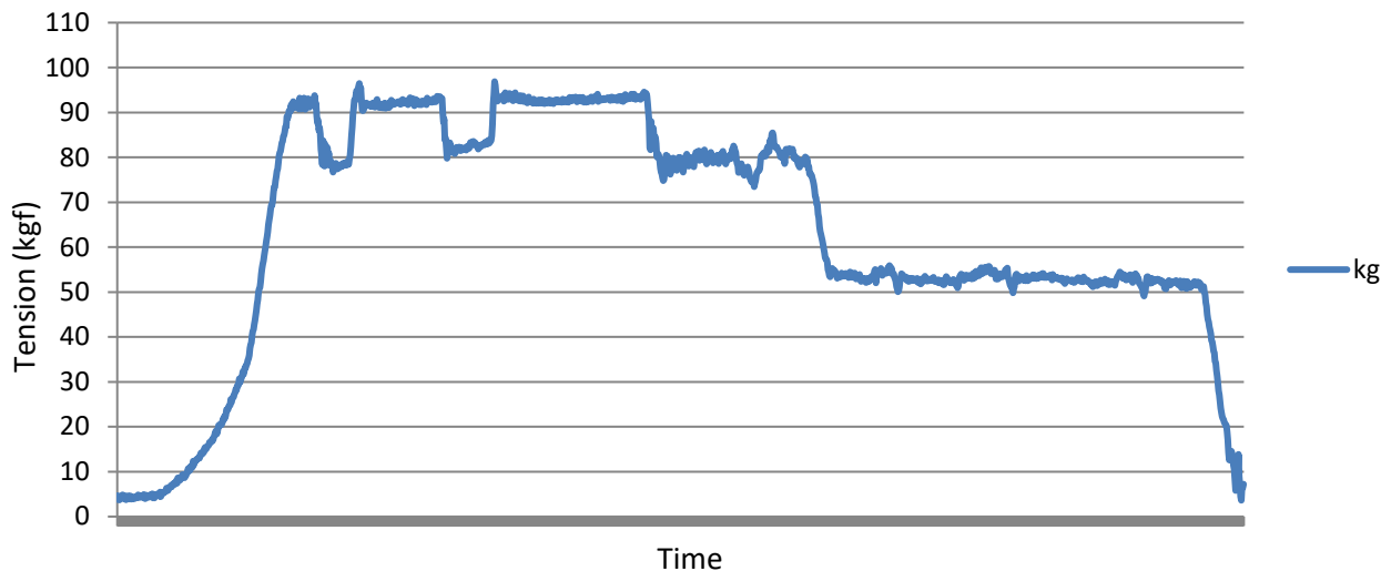
11.1mm Sterling HTP rope, 90 degree bend over 60mm polished Aluminium tube, 75kg test mass: raise, rest, then lower.
