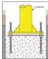
Leveling Plate
