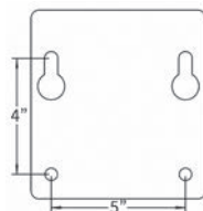
Mounting Plate (GBA-18042)
